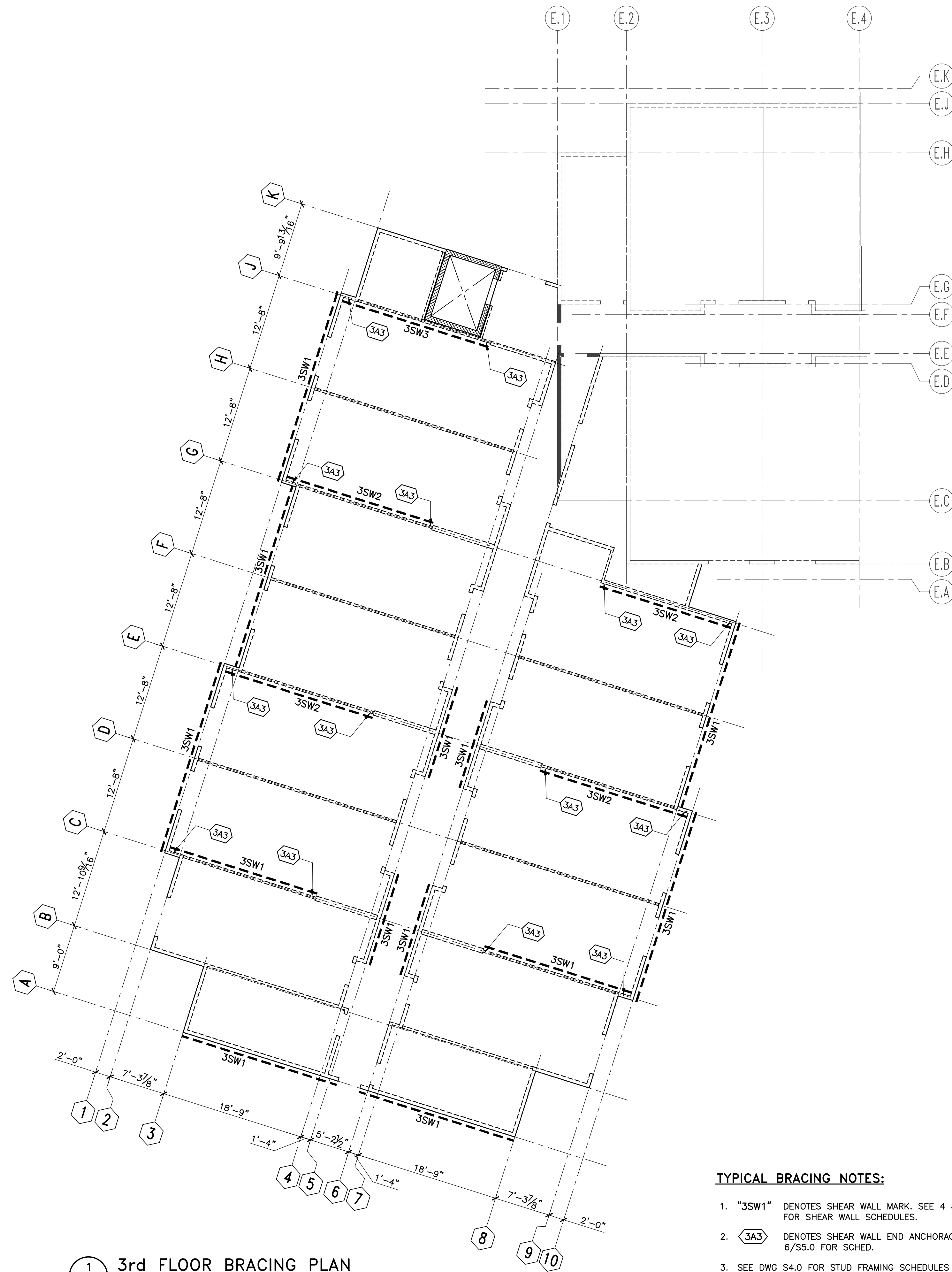
1 3rd FLOOR BRACING PLAN S5.3 SCALE: 1/8" = 1'-0"
