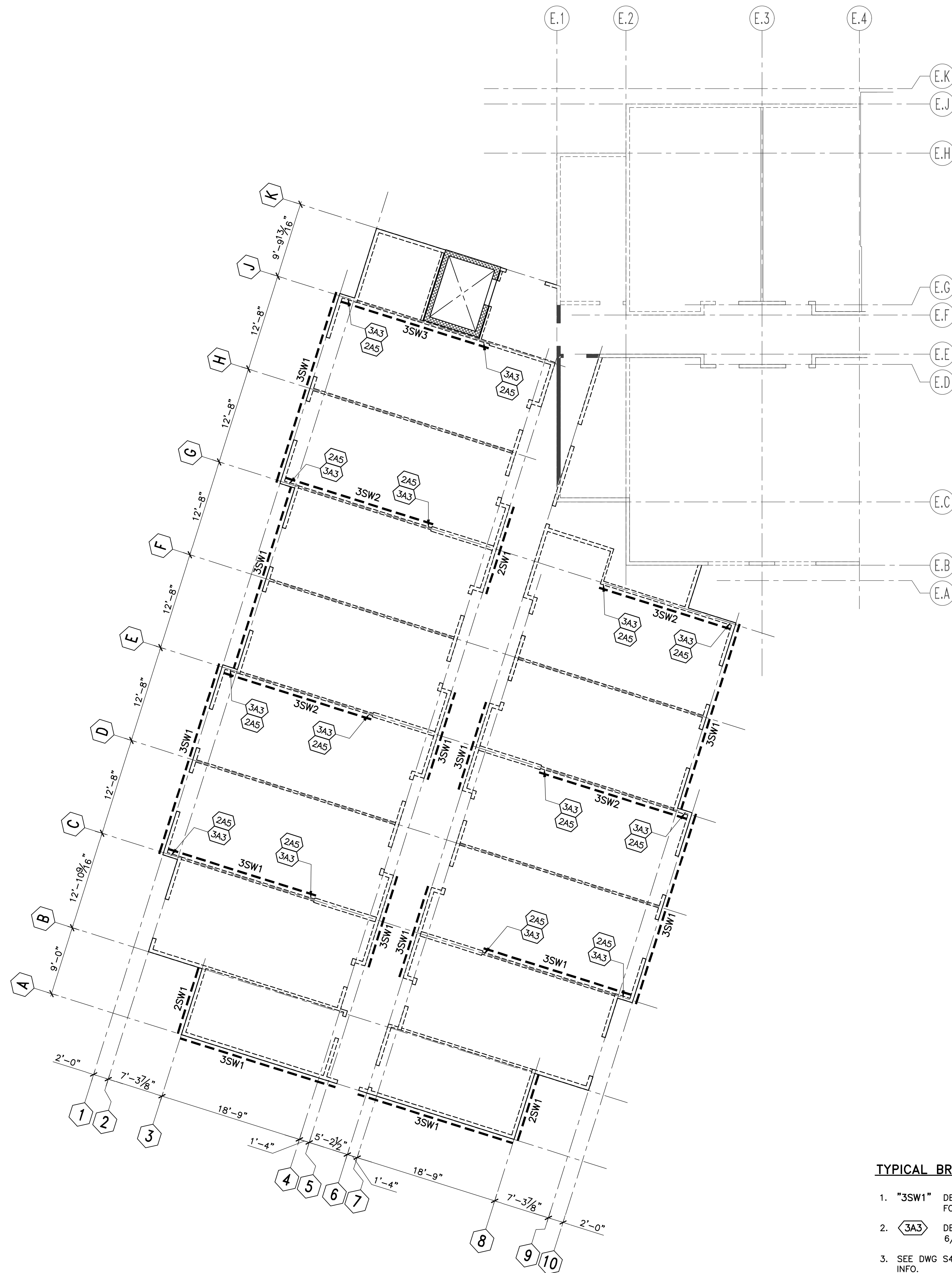
1 2nd FLOOR BRACING PLAN S5.2 SCALE: 1/8" = 1'-0"
