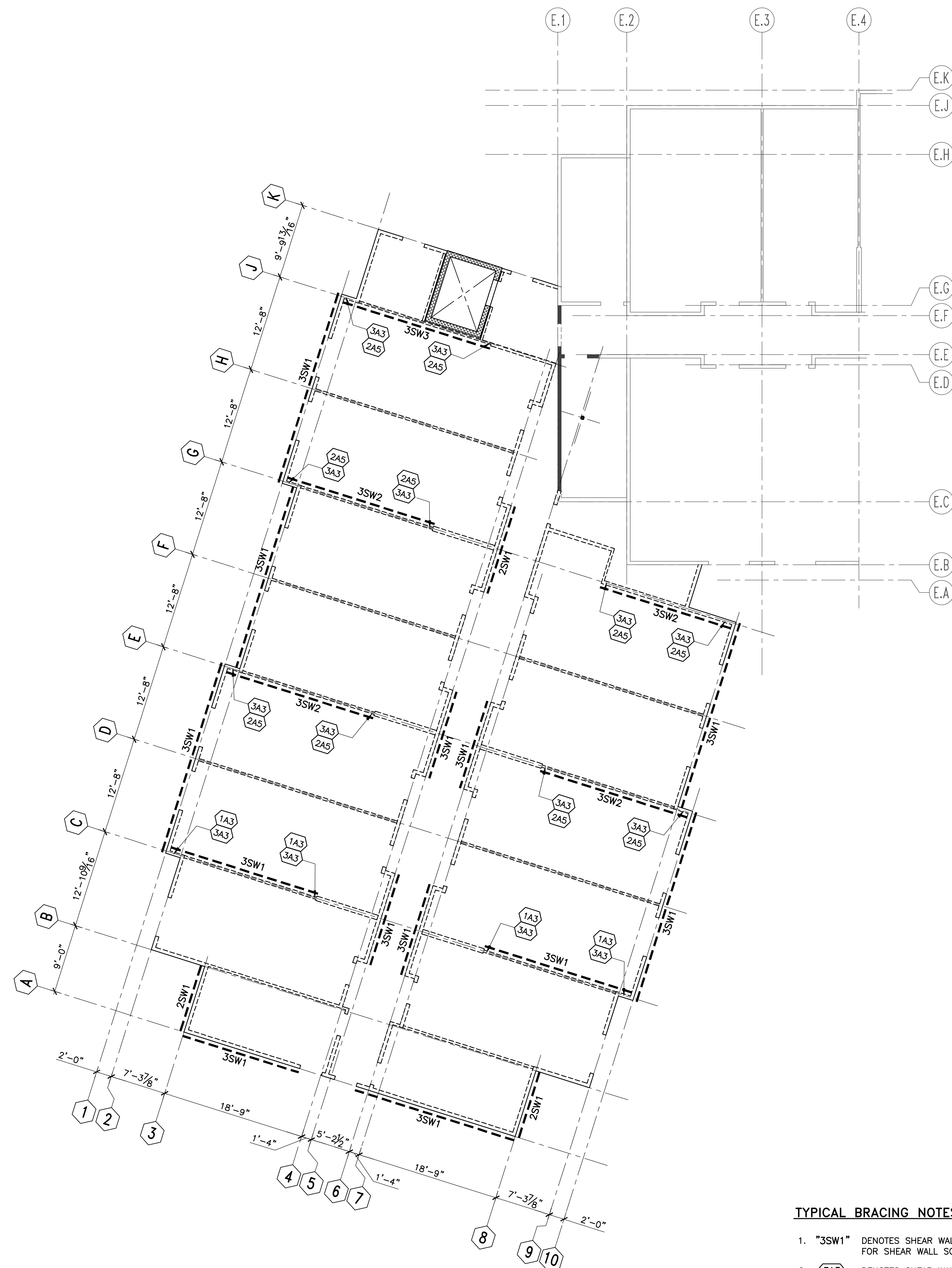
1 1st FLOOR BRACING PLAN S5.1 SCALE: 1/8" = 1'-0"
