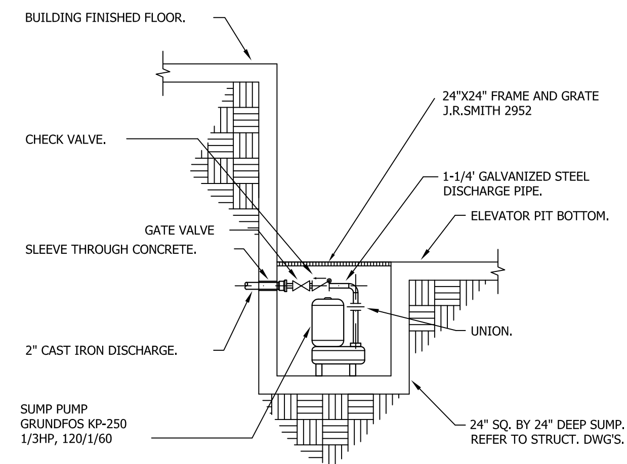
2 ELEVATOR SUMP PUMP DETAIL P4.01 NOT TO SCALE
