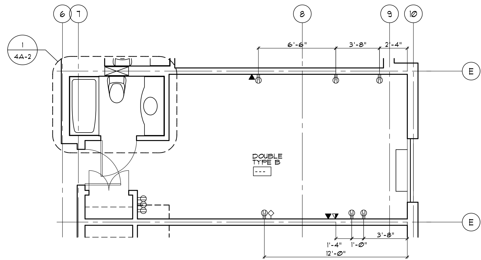
2 TYPE B DOUBLE ROOM ELECTRICAL LAYOUT SCALE 1/4"=1'-0"
