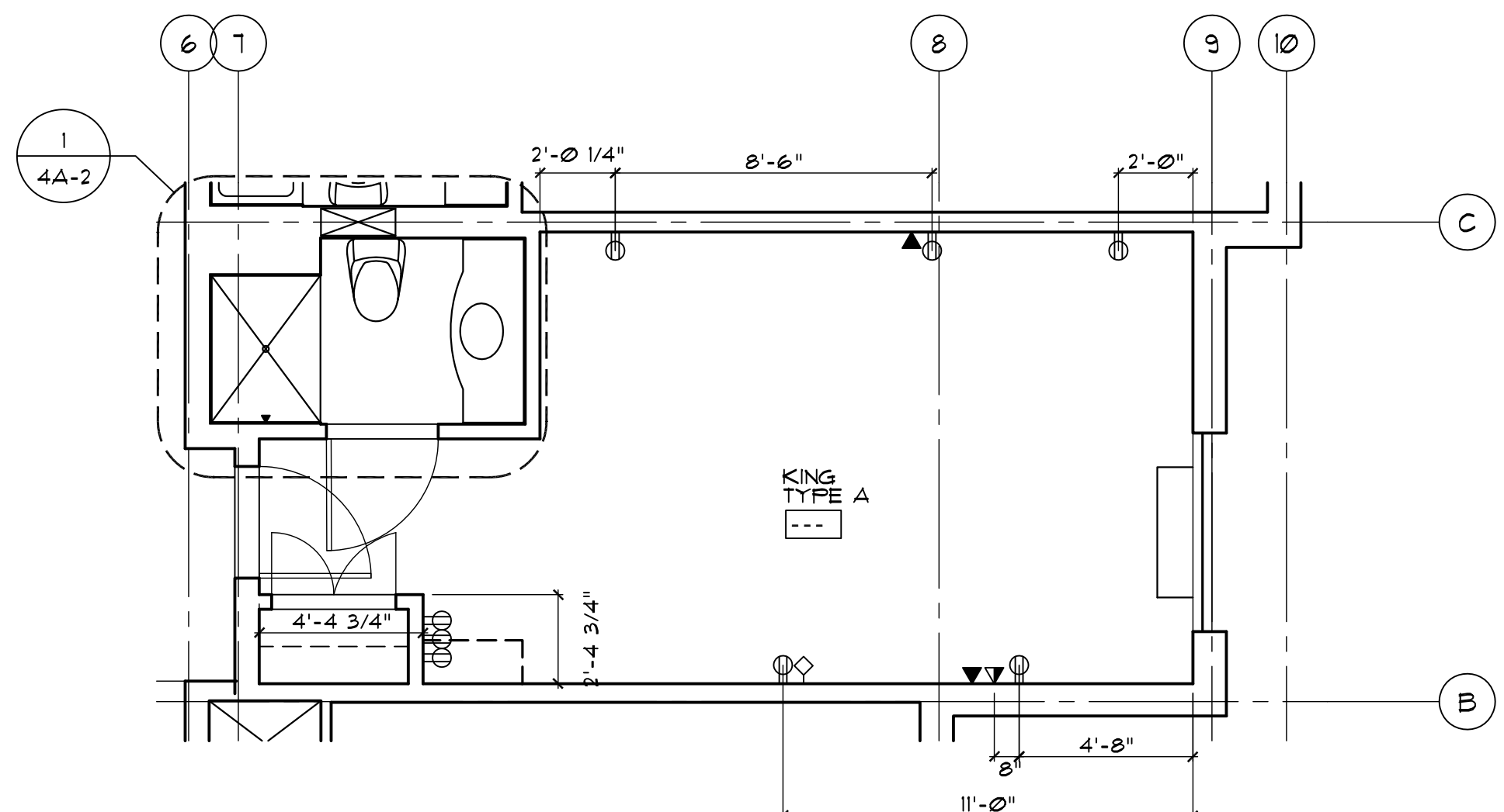
1 TYPE A KING ROOM ELECTRICAL LAYOUT SCALE 1/4"=1'-0"
