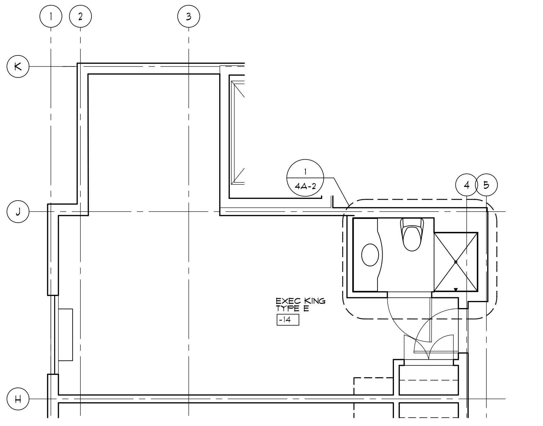
4 TYPE E EXEC KING ROOM ELECTRICAL LAYOUT SCALE 1/4"=1'-0"
