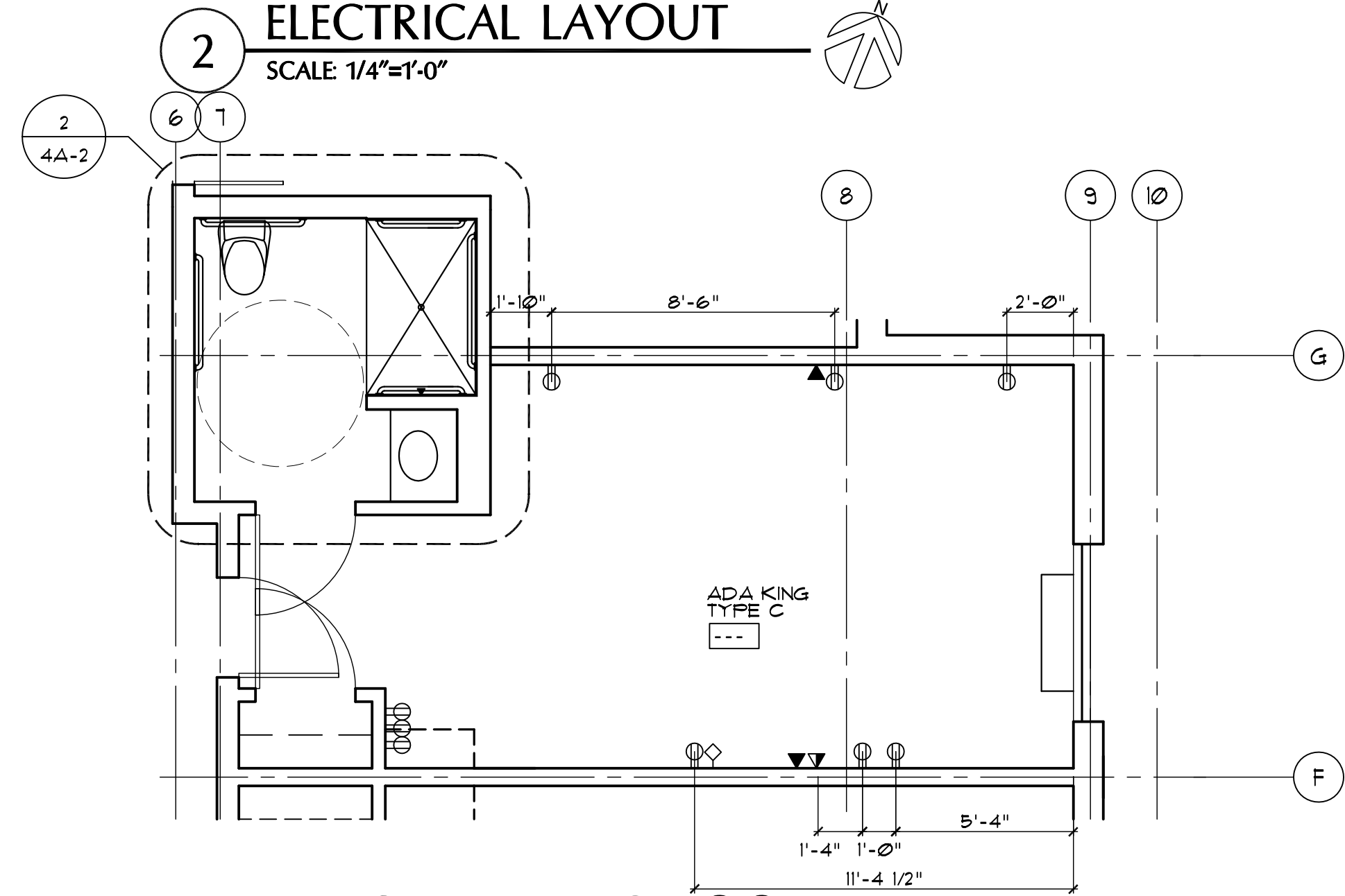
3 TYPE C ADA KING ROOM ELECTRICAL LAYOUT SCALE 1/4"=1'-0"
