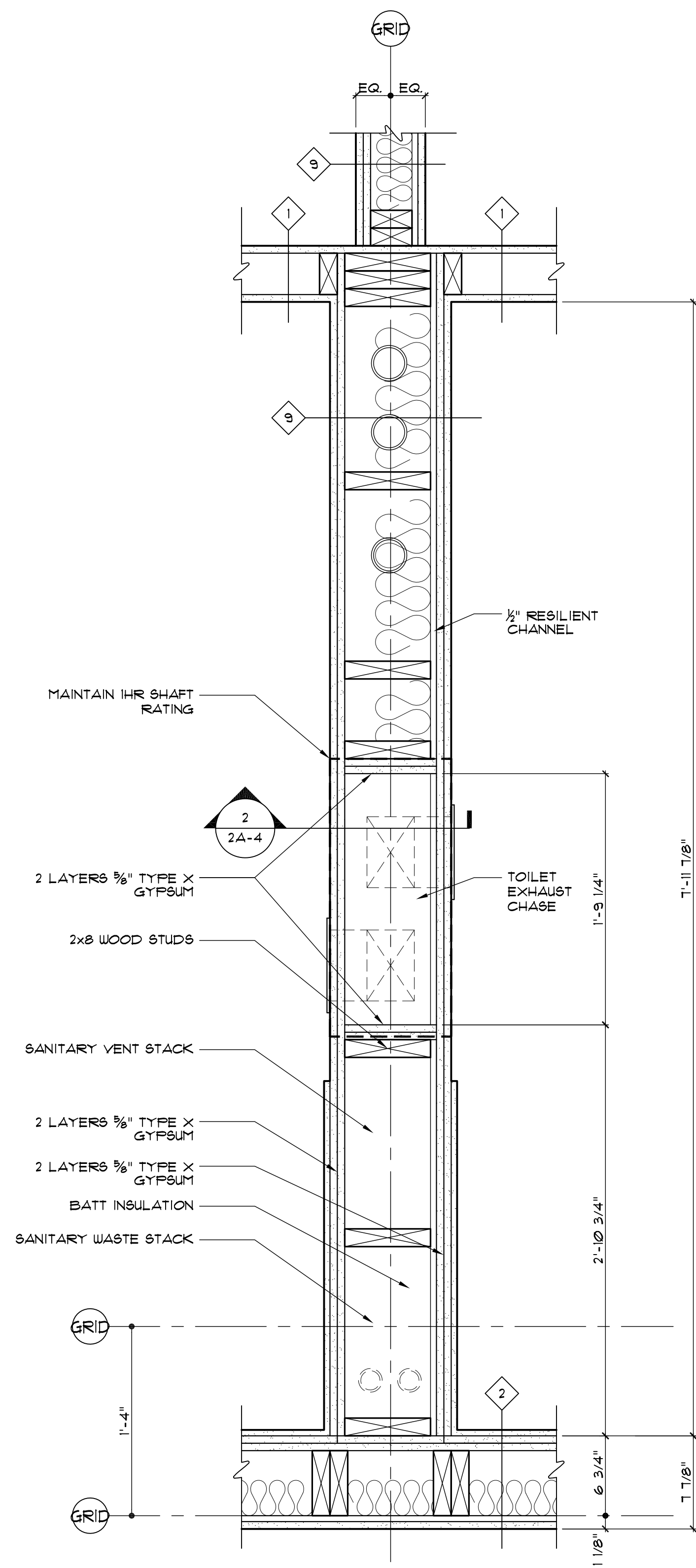
5 TYPICAL CHASE DETAIL SCALE 1 1/2"=1'-0"
