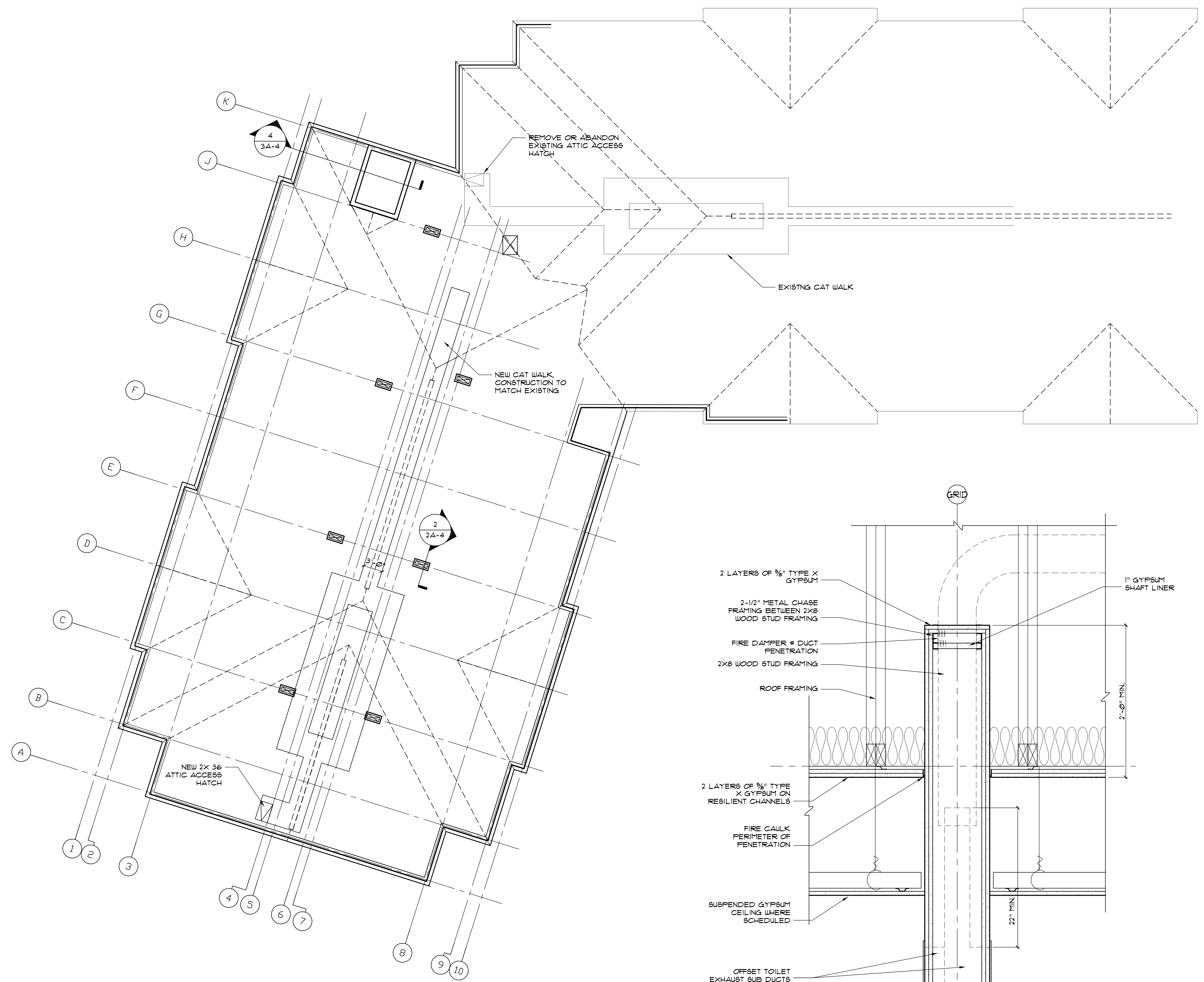
1 ATTIC PLAN SCALE: 1/8"=1'-0"
