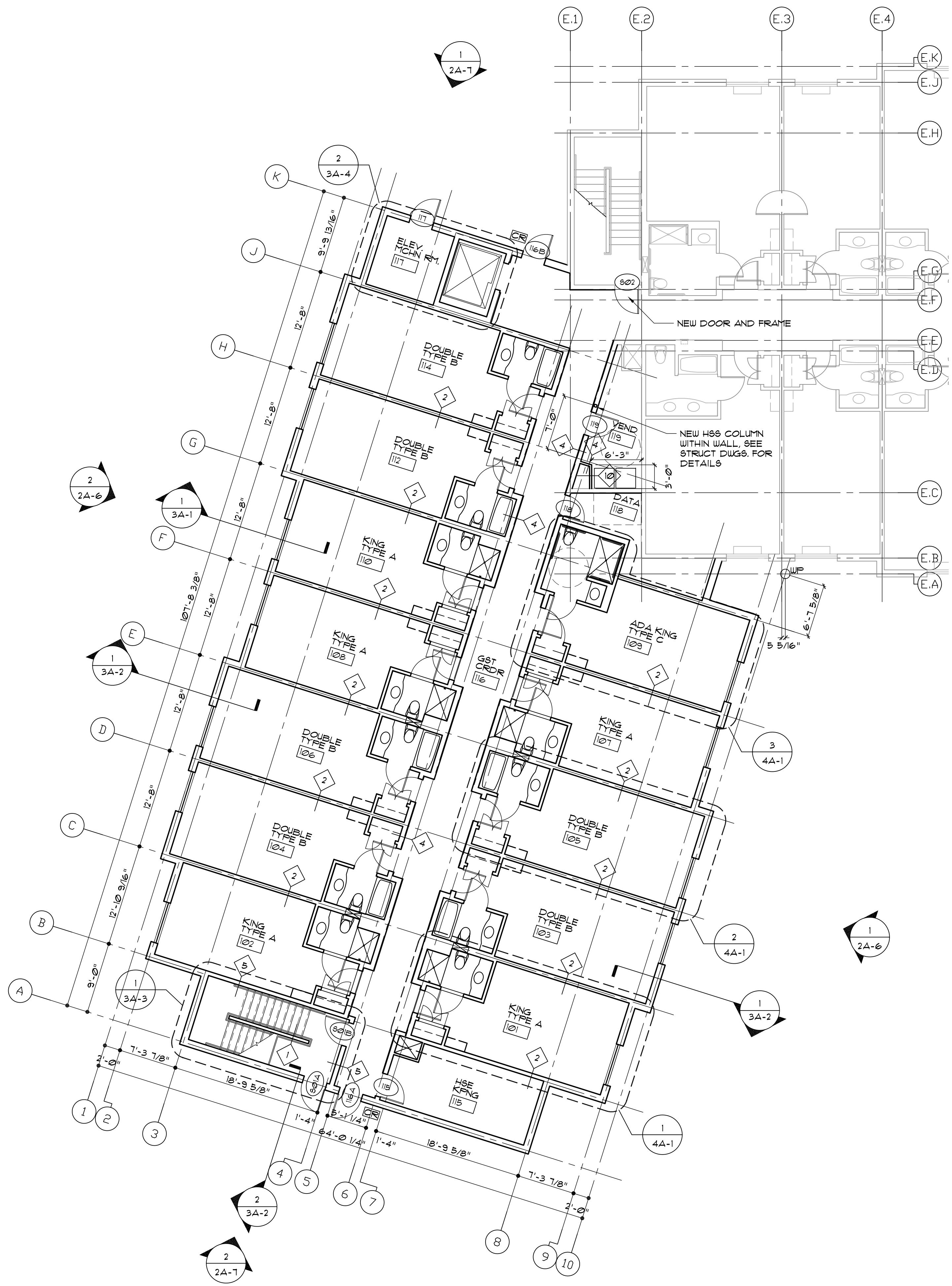
1 LOBBY LEVEL PLAN SCALE: 1/8"=1'-0"
