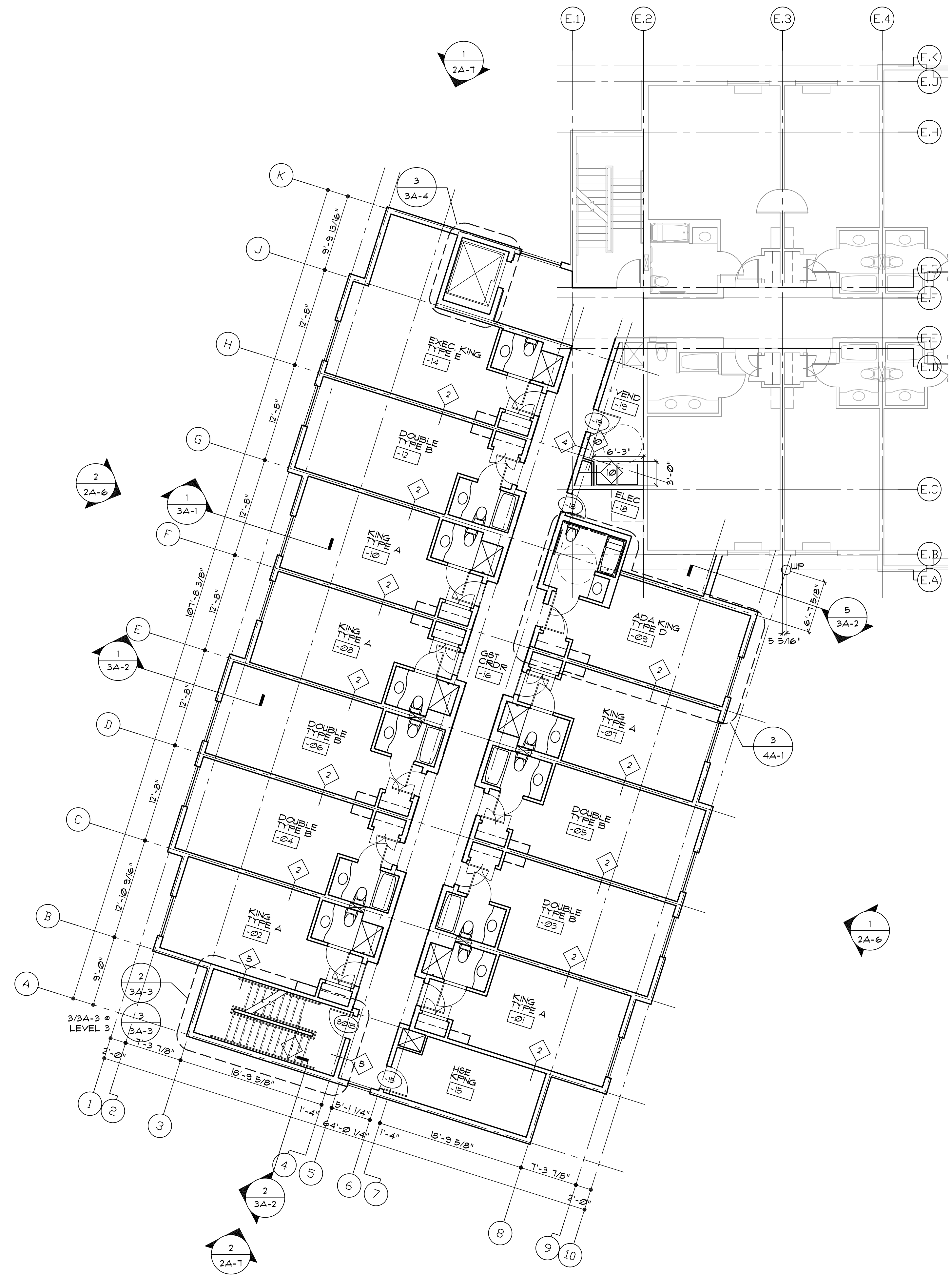
2 2ND & 3RD LEVEL PLAN SCALE: 1/8"=1'-0" SEE 3/3A-3 FOR LEVEL 3 STAIRS
