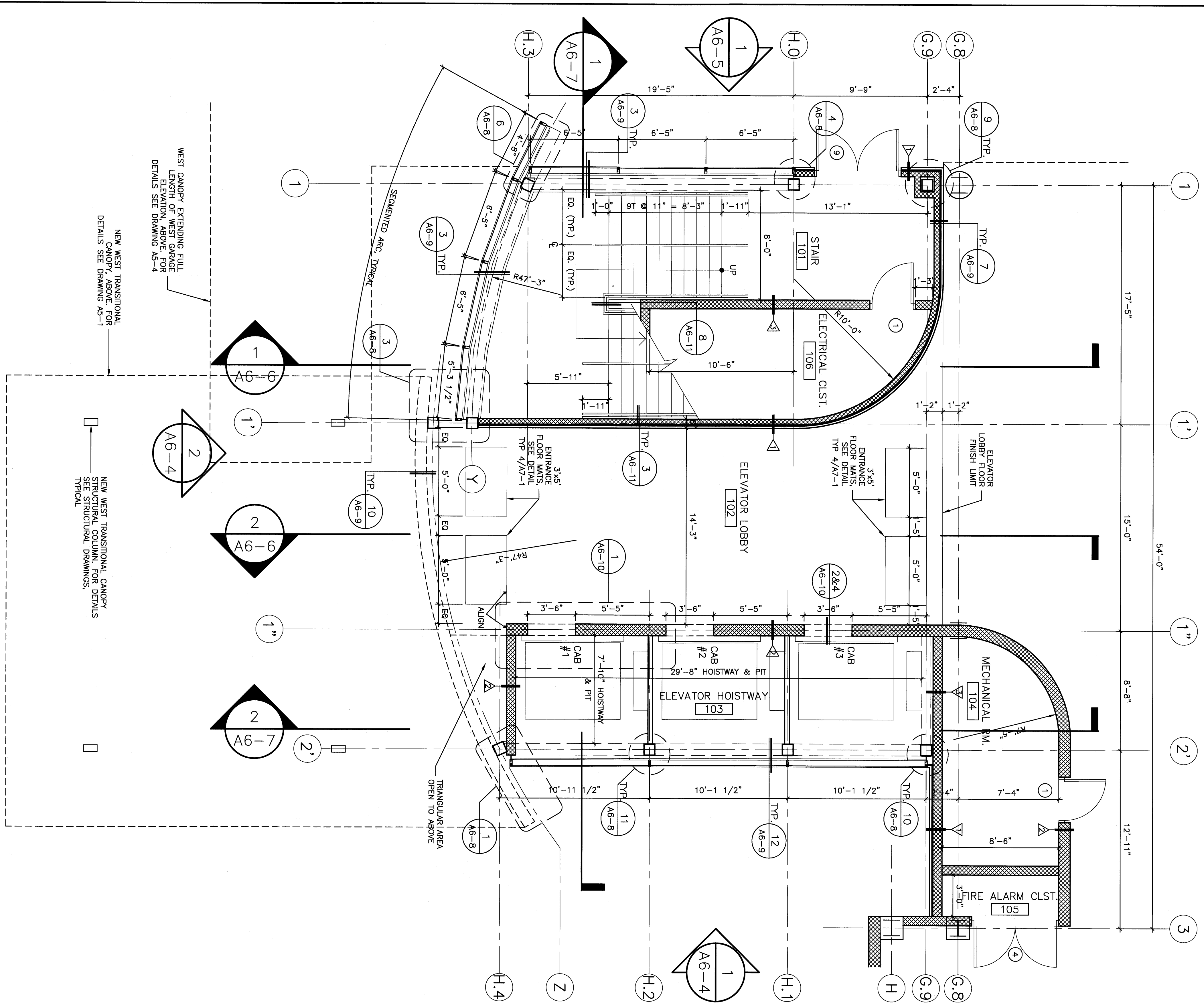
1 LEVEL 1 - GROUND FLOOR SCALE 1/4" = 1'-0"
