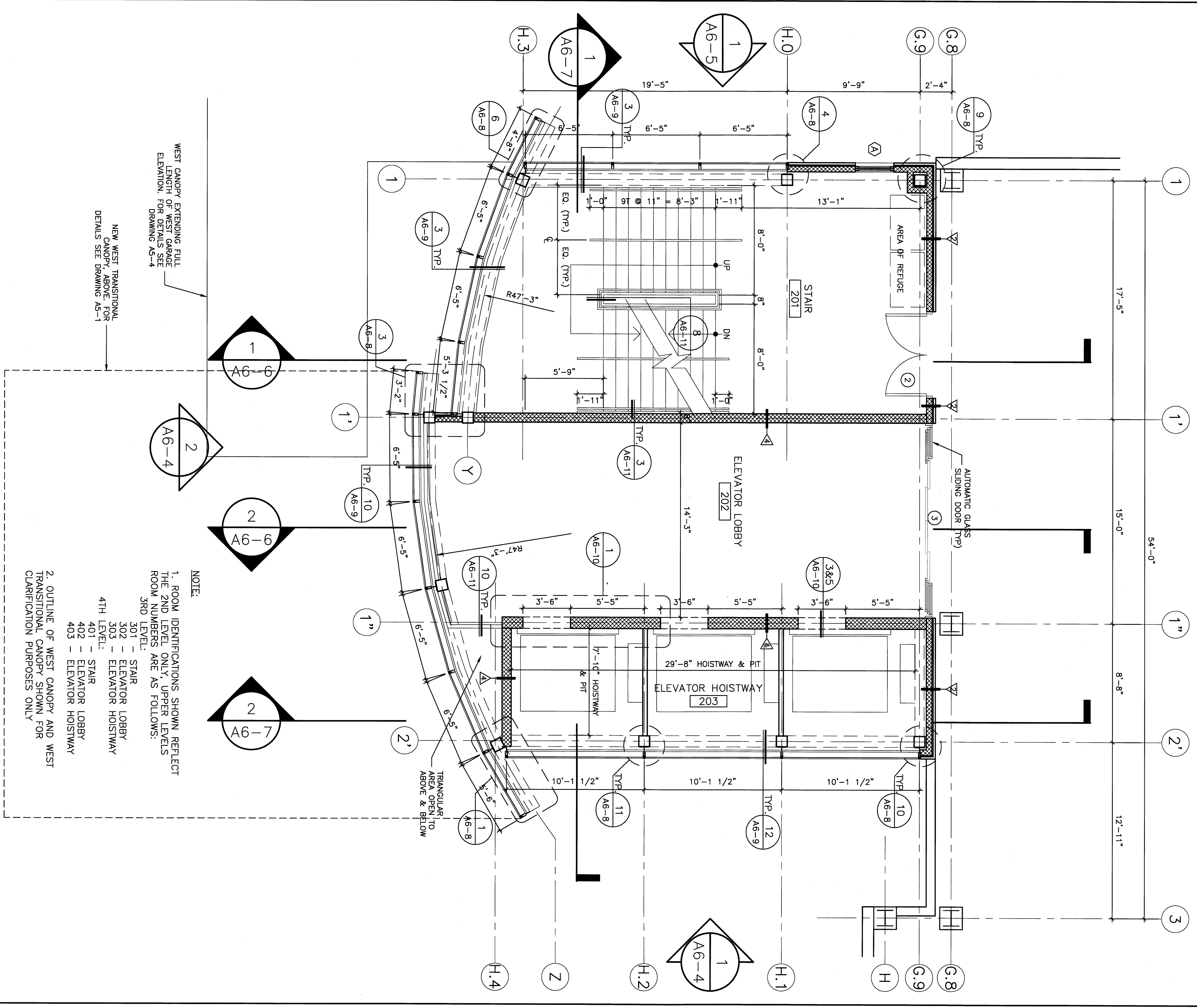
2 TYPICAL LEVEL - 2ND TO 4TH SCALE 1/4" = 1'-0"
