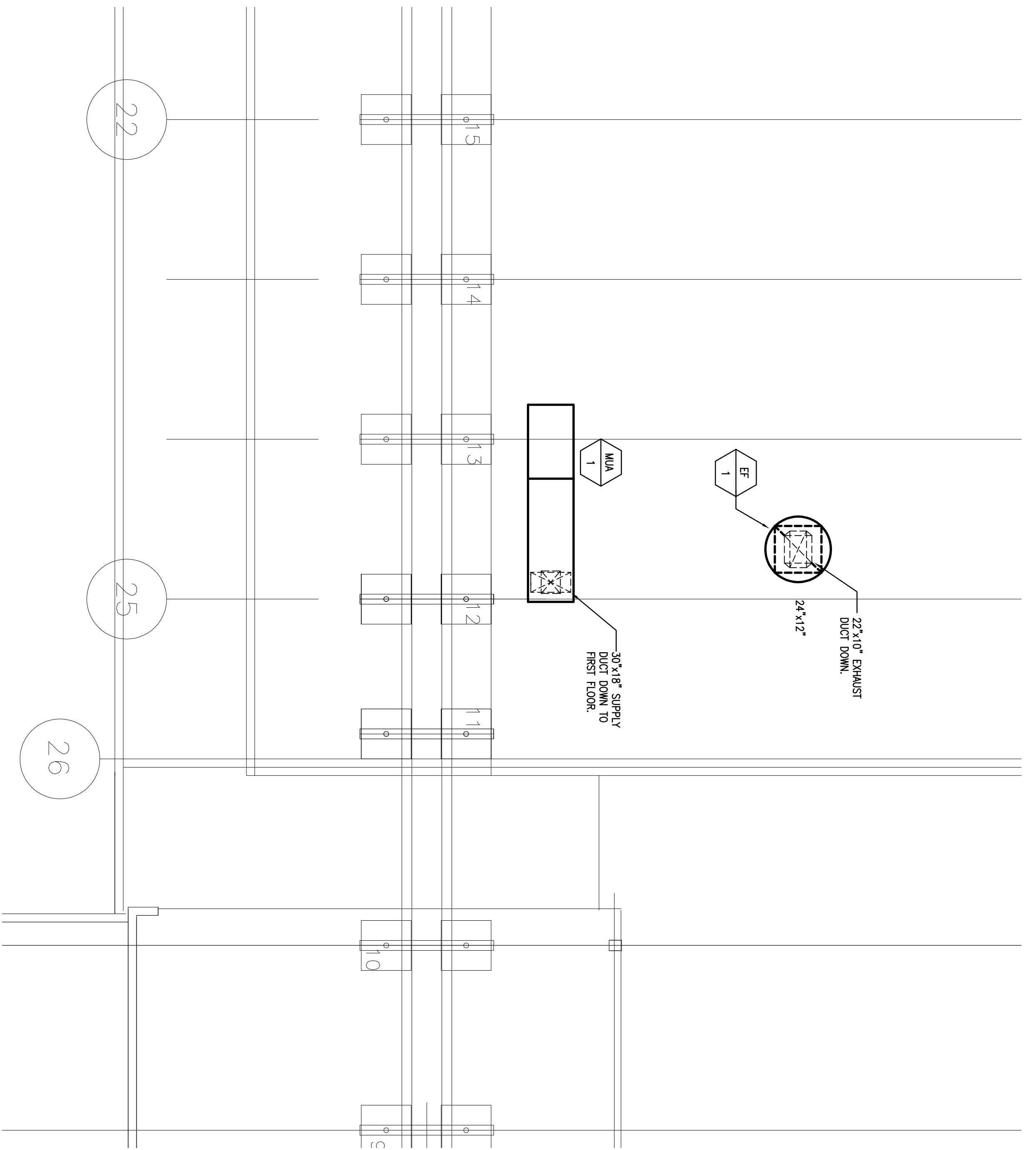
2 HVAC Roof Plan 1/4"=1'-0"
