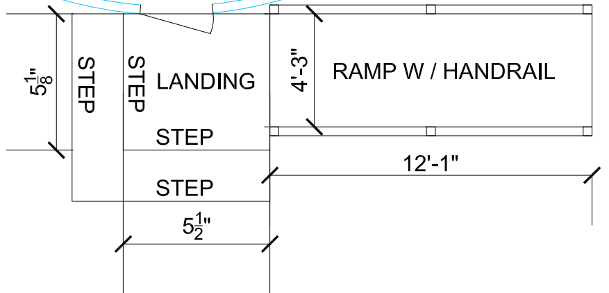
30' DIA. WARMING HUT TENT PLAN VIEW
