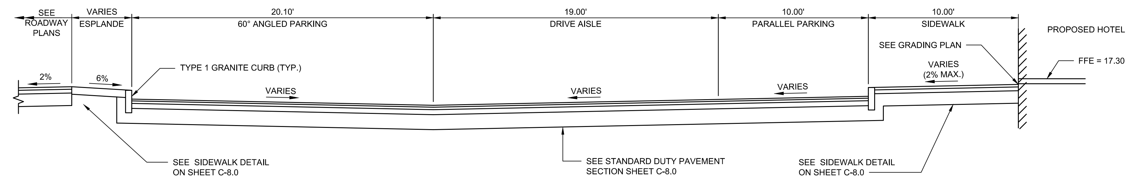
TYPICAL ROADWAY SECTION A-A NOT TO SCALE
