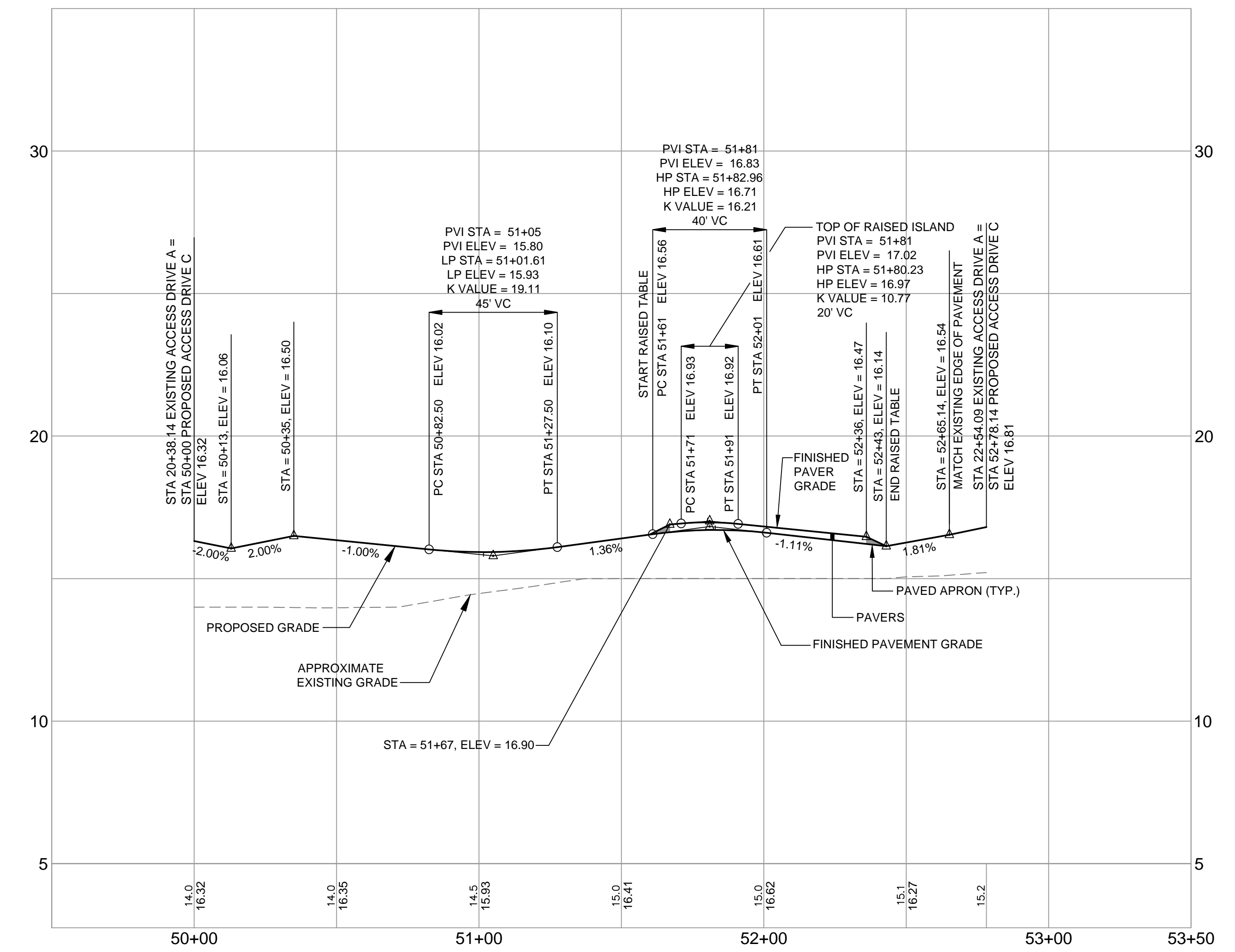
ACCESS ROAD PROFILE 'C'
