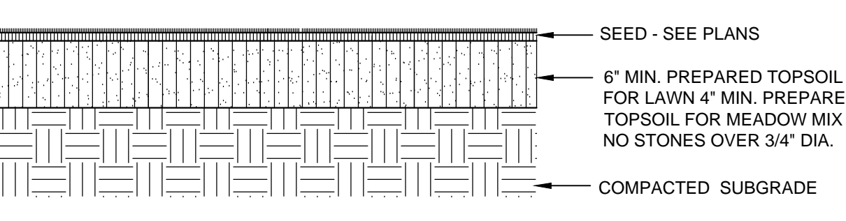
3 LAWN OR MEADOW SEED PLANTING SCALE: 1"=1'-0"
