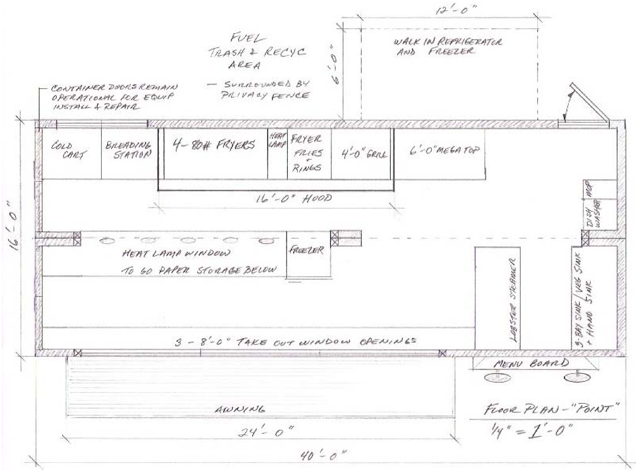
FIGURE A-2 FLOOR PLAN
