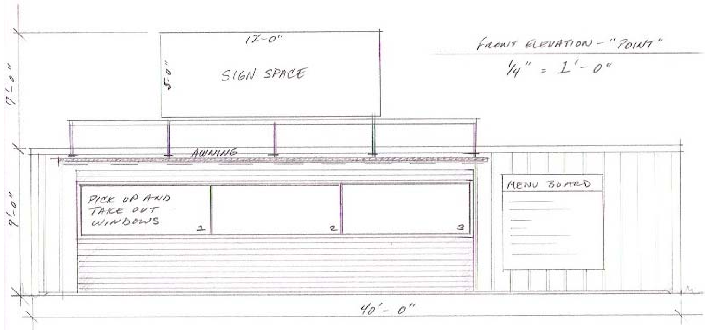
FIGURE A-1 FRONT ELEVATION
