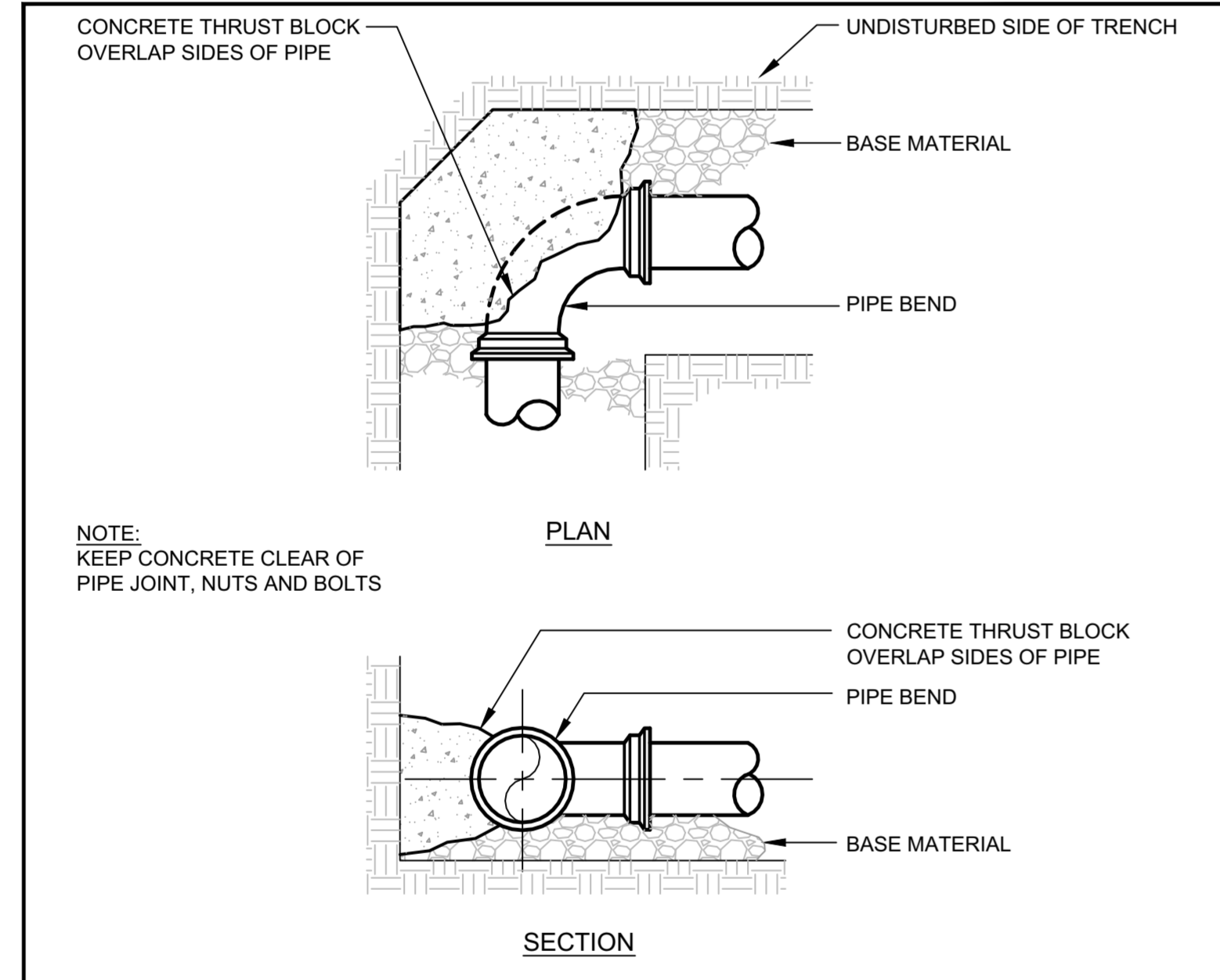
(H) TYPICAL THRUST BLOCK PLACEMENT BENDS N.T.S.
