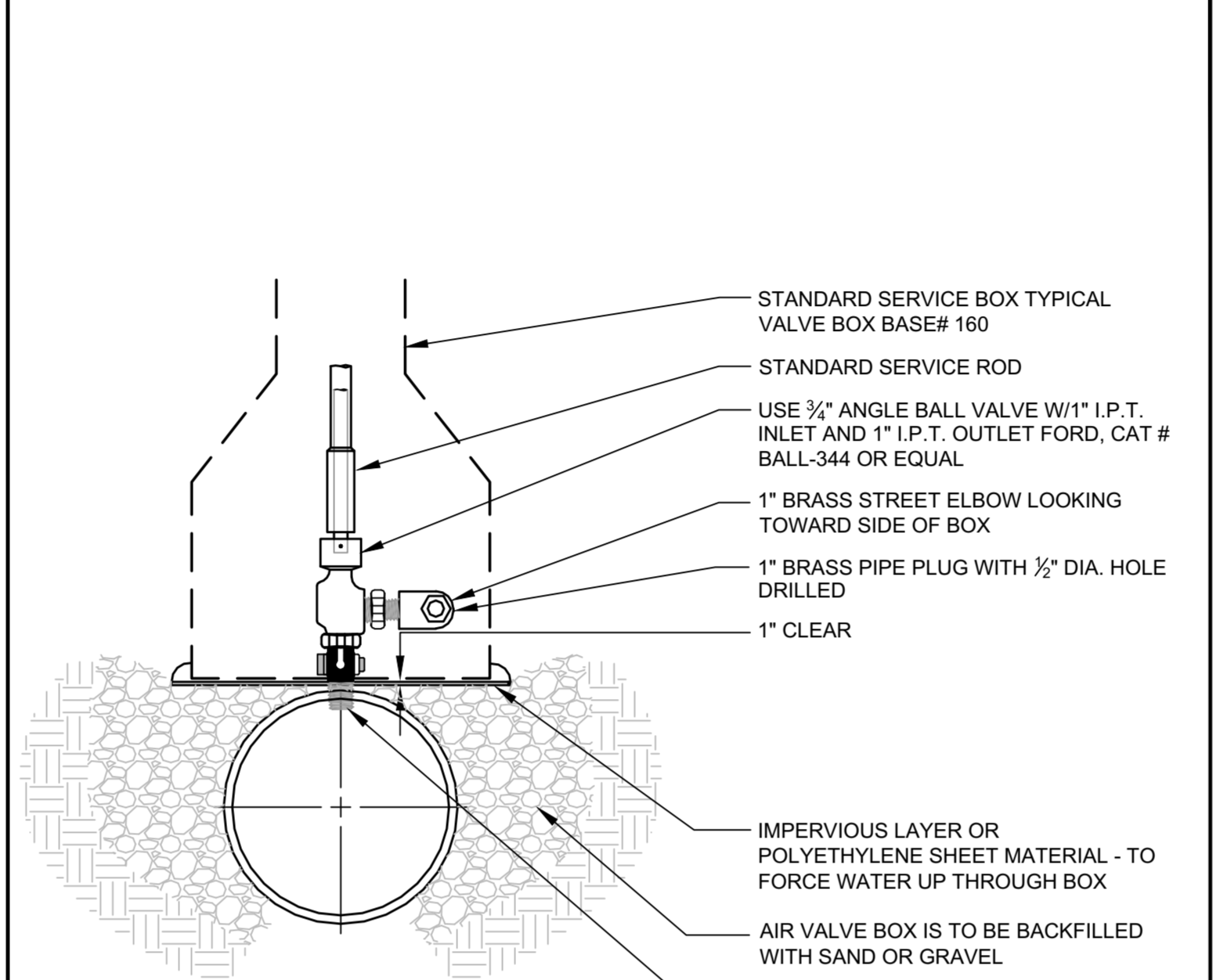
(F) TYPICAL AIR VALVE SECTION (1") N.T.S.
