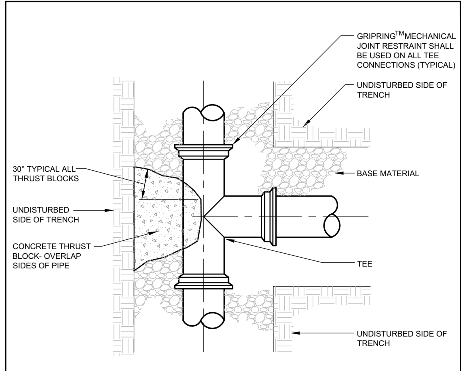
(I) TYPICAL THRUST BLOCK PLACEMENT ON TEES N.T.S.
