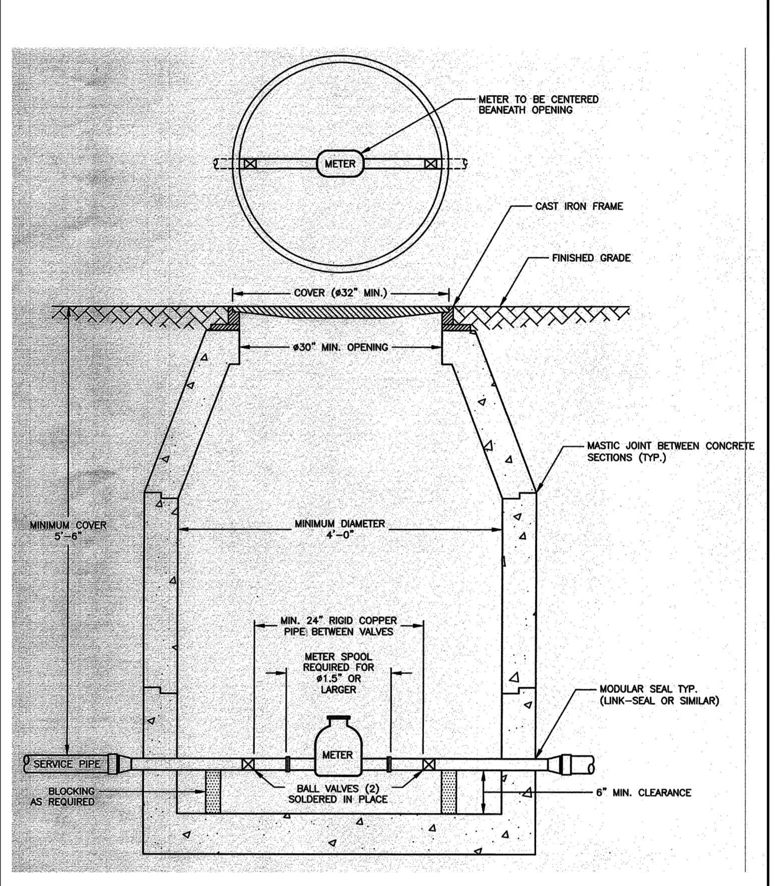
(G) WATER METER PIT DETAIL N.T.S.
