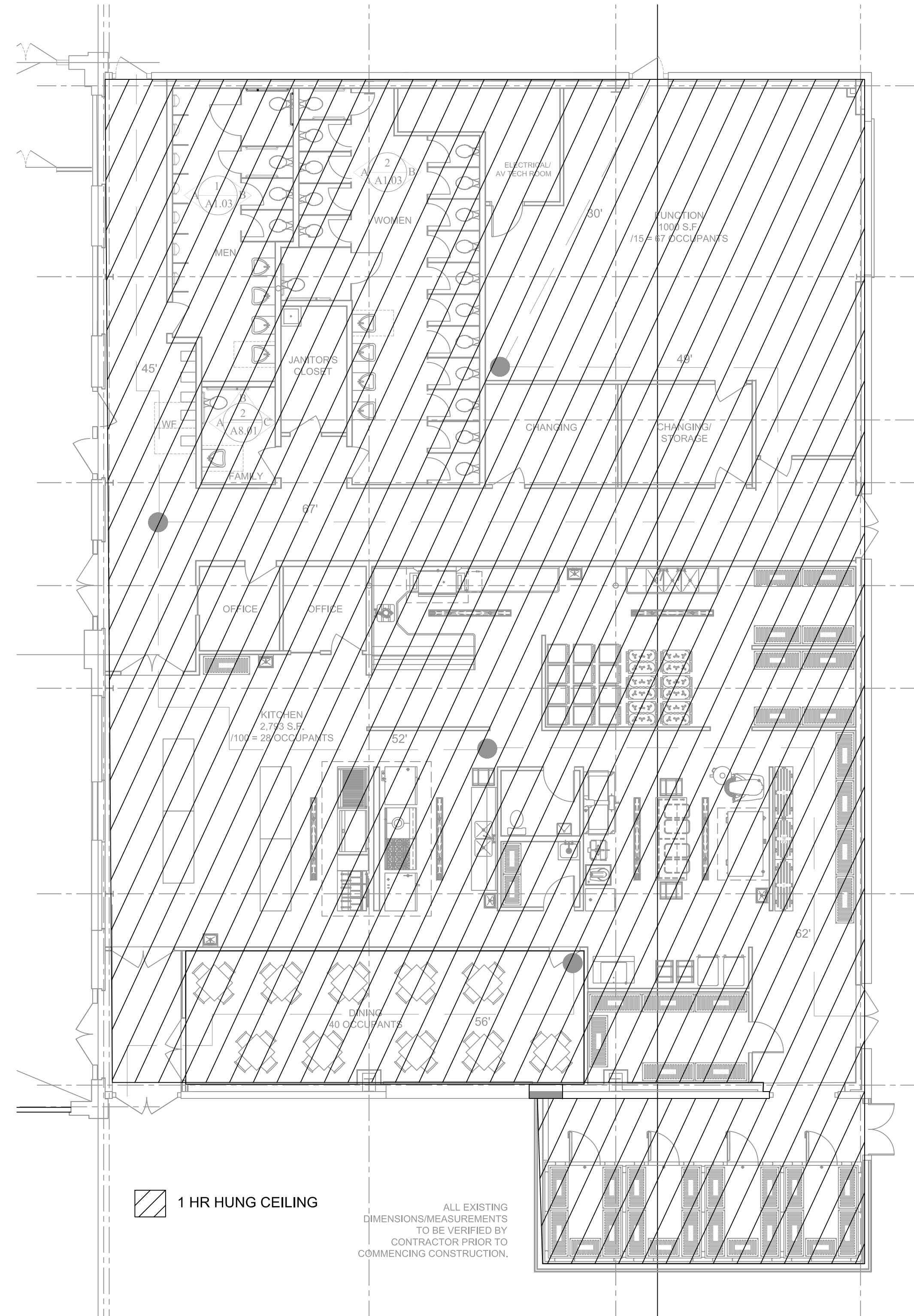
3 EAST ANNEX CEILING PLAN A1.02 1/8" = 1'-0"
