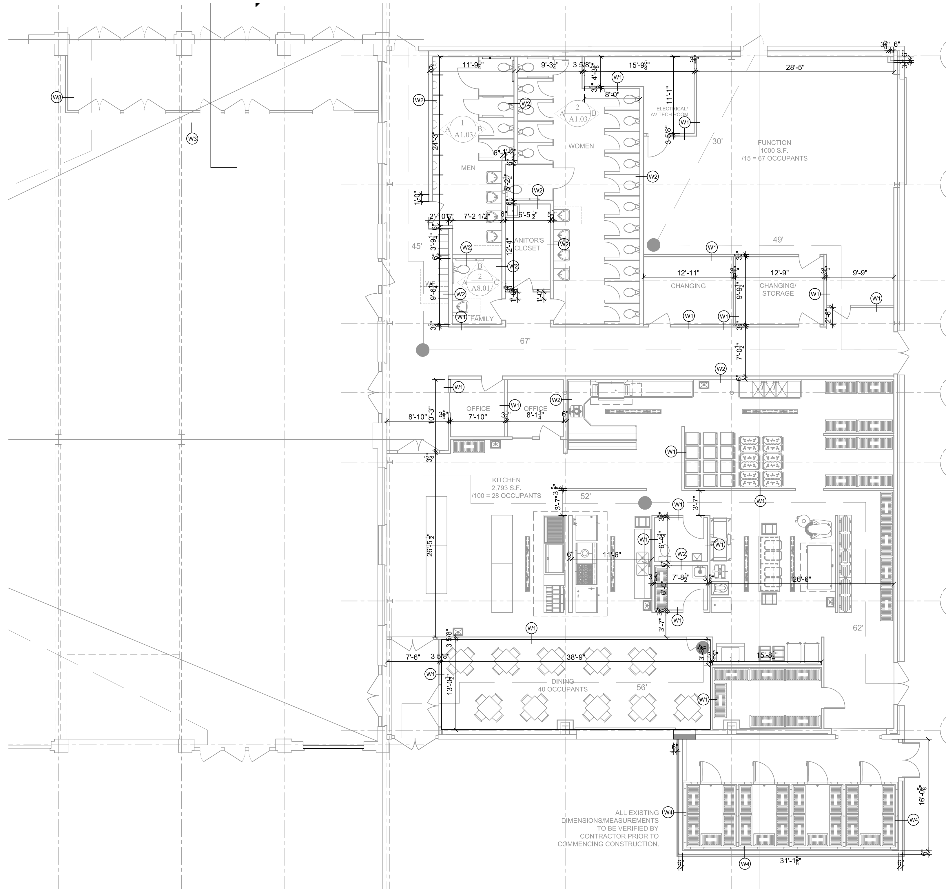
2 EAST ANNEX DIMENSION PLAN A1.02 1/8" = 1'-0"
