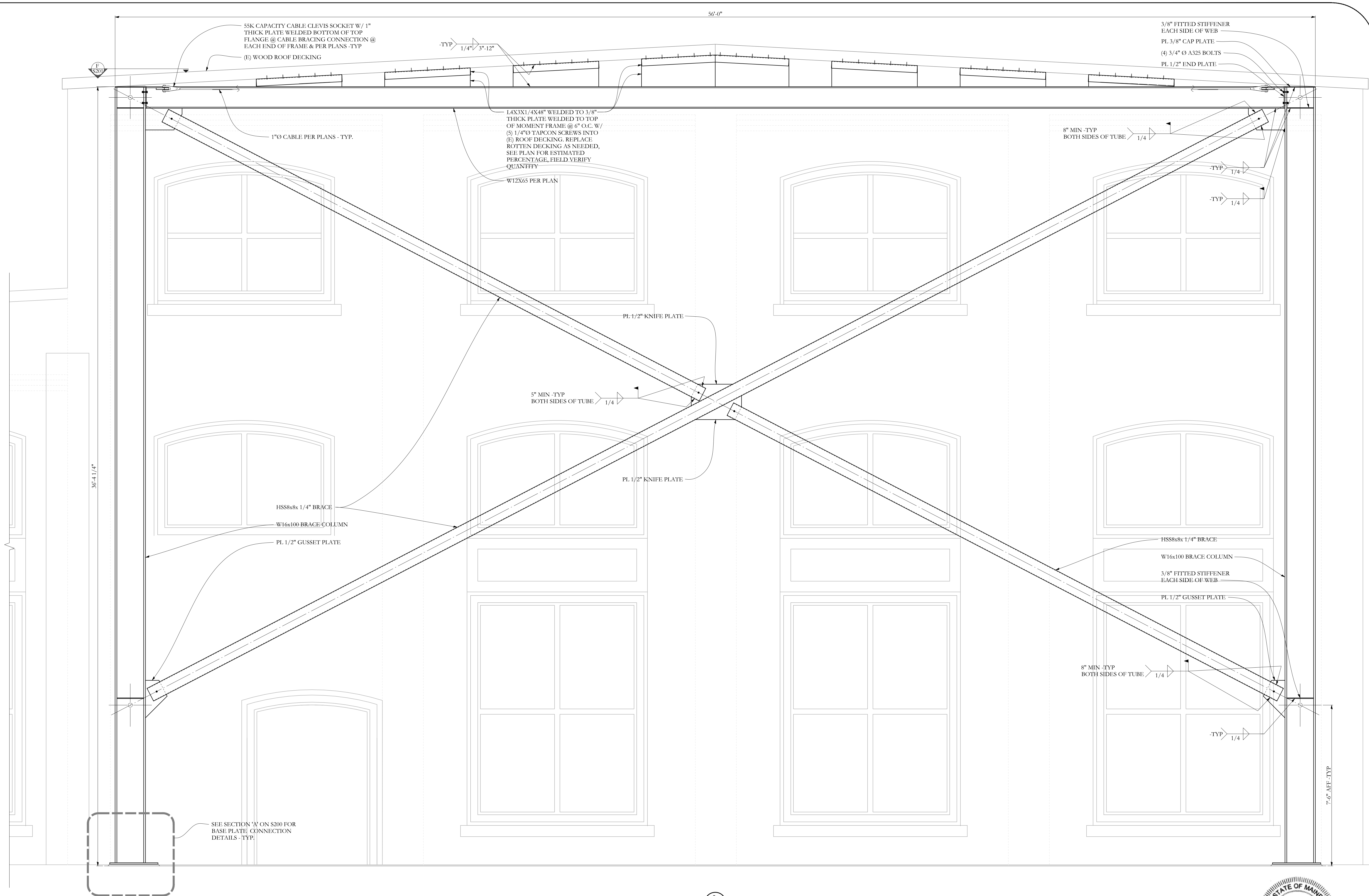
SECTION L S202 1/2"=1'-0"
