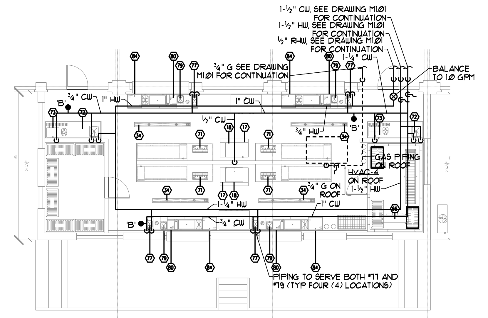
BAR AREA DOMESTIC WATER PLUMBING AND GAS PIPING PLAN SCALE - 1/8" = 1'-0"
