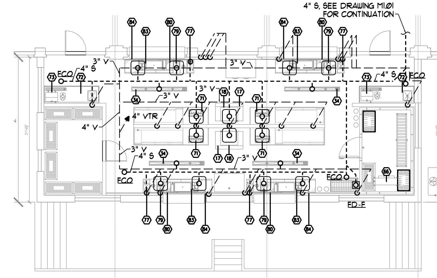
BAR AREA SANITARY PLUMBING PLAN SCALE - 1/8" = 1'-0"
