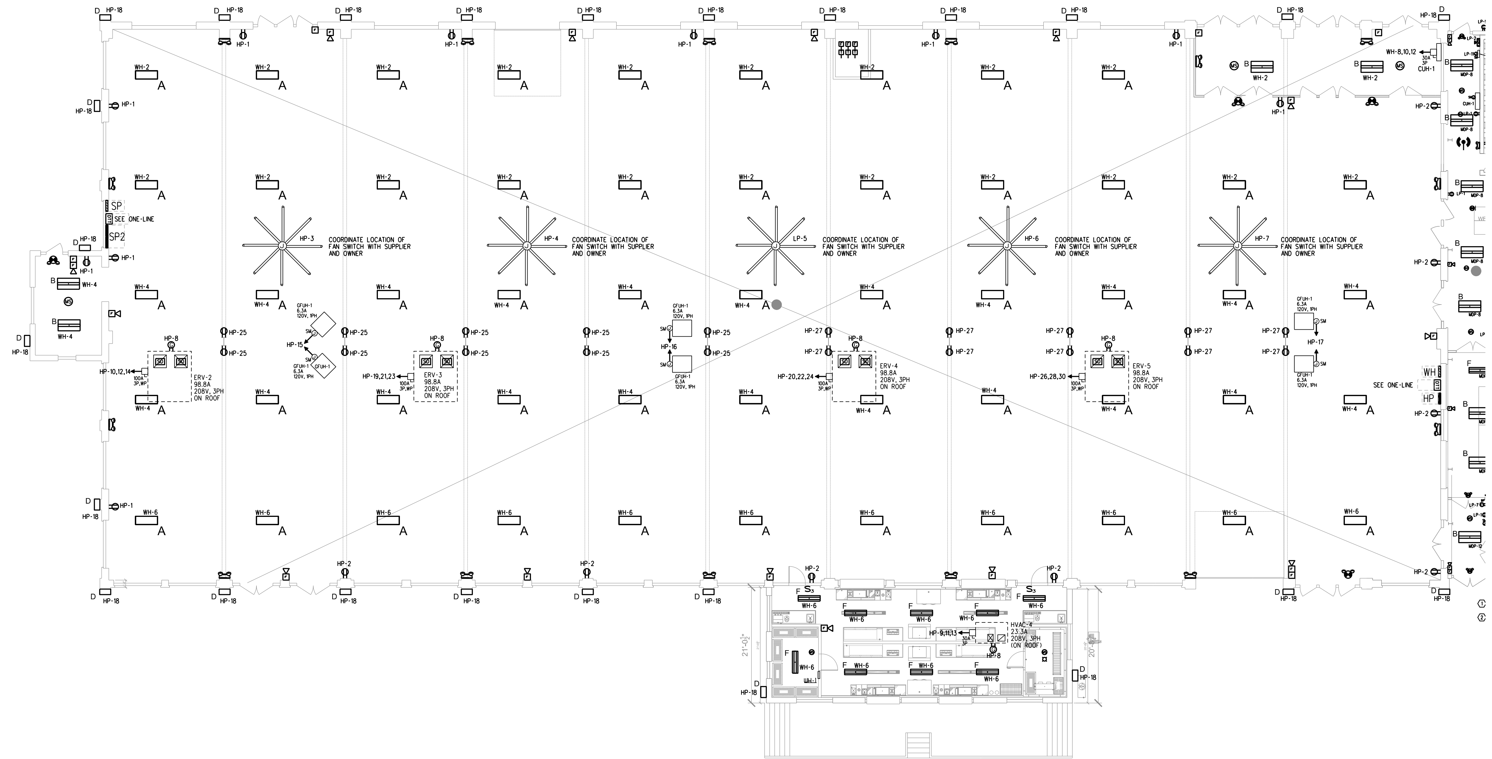
ELECTRICAL PLAN SCALE: 3/32"=1'-0" REFER TO BAR PLAN DRAWING E104 FOR BAR POWER REQUIREMENTS.
