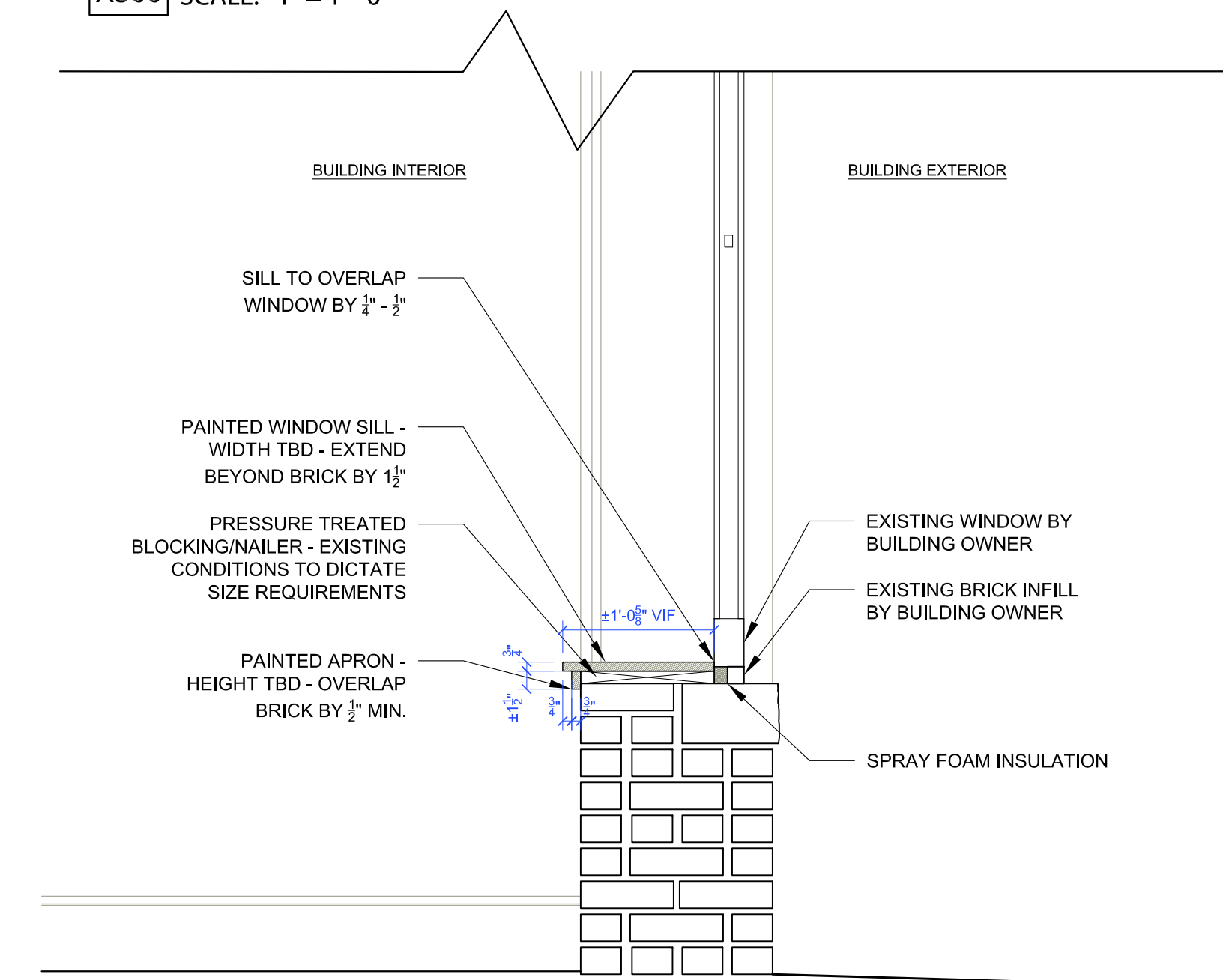
4 WINDOW SILL CASING DETAIL (LOWER WINDOWS ONLY) A300 SCALE: 1" = 1' - 0"
