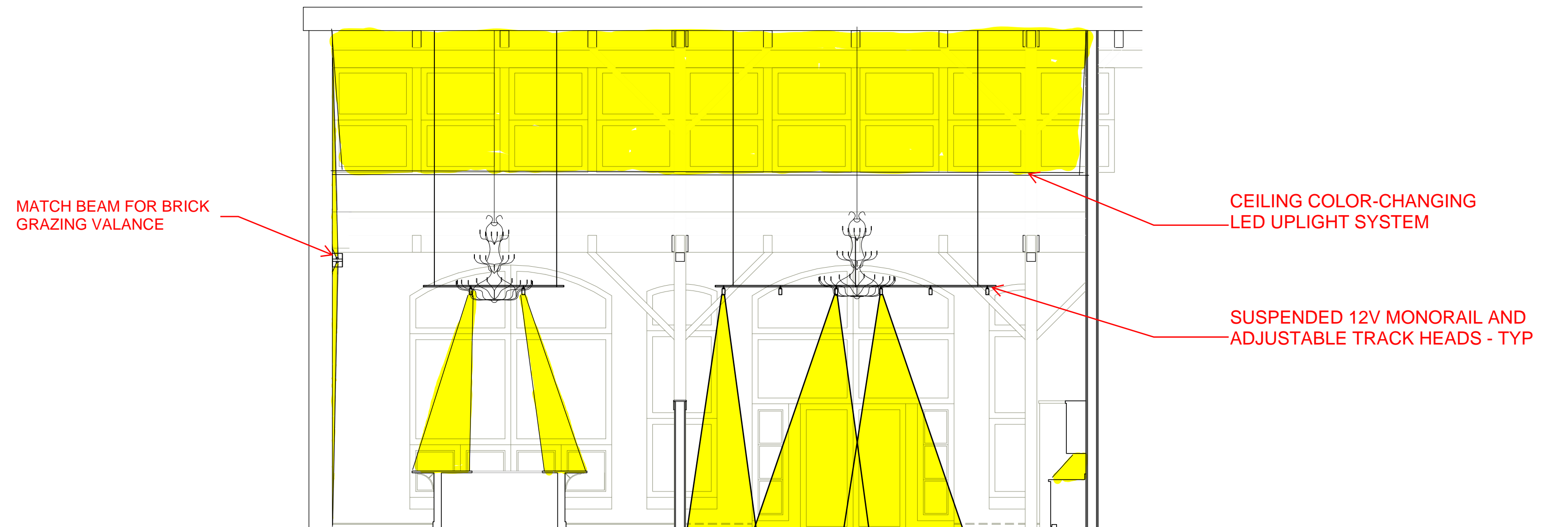
3 Preliminary Lighting Section B Scale: 3/16"=1'0"
