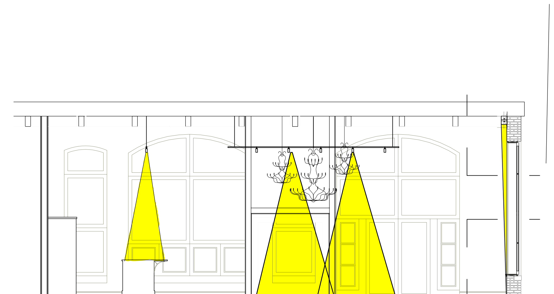
4 Preliminary Lighting Section C Scale: 3/16"=1'0"
