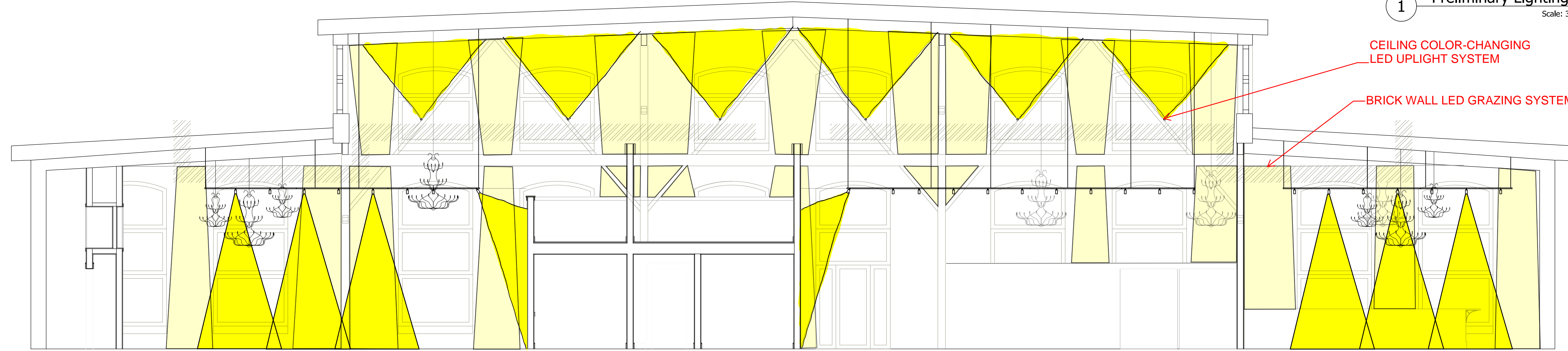
2 Preliminary Lighting Section A Scale: 3/16"=1'0"
