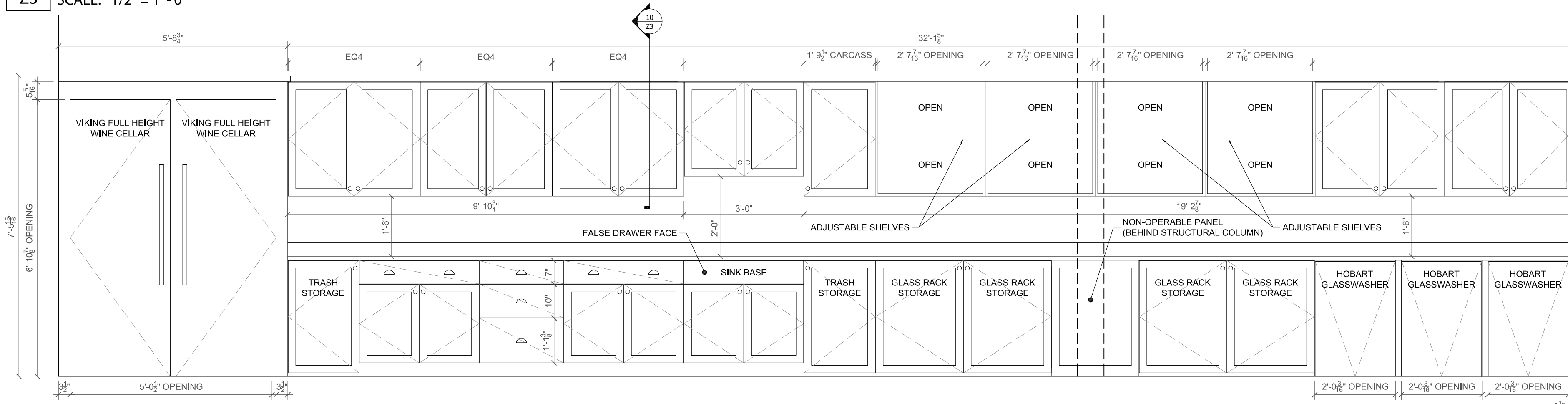
9 MARKET 109 WALL CABINERY: ELEVATION Z3 SCALE: 1/2" = 1' - 0"
