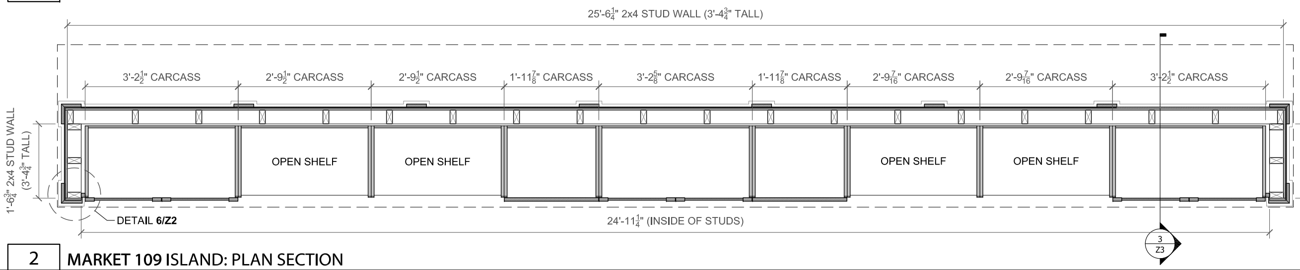
2 MARKET 109 ISLAND: PLAN SECTION Z3 SCALE: 1/2" = 1' - 0"
