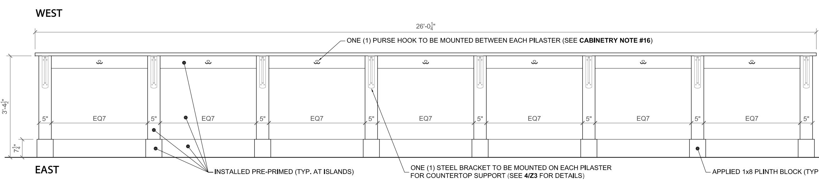
5 MARKET 109 ISLAND: ELEVATIONS Z3 SCALE: 1/2" = 1' - 0"
