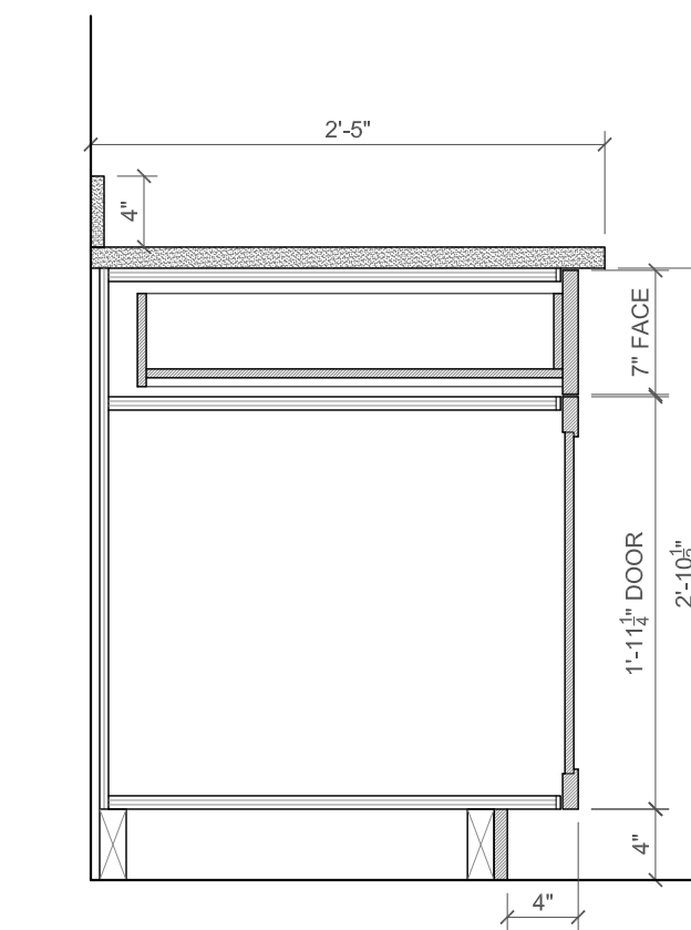
8 MARKET 109 BASE CABINERY - TYPICAL SECTION Z3 SCALE: 1" = 1' - 0"
