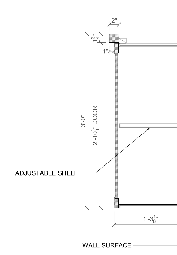
10 TYPICAL UPPER CABINET SECTION Z3 SCALE: 1" = 1' - 0"
