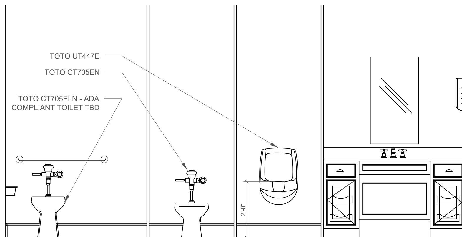
2 MEN'S ROOM FIXTURE WALL ELEVATION A400 SCALE: 1/2" = 1' - 0"
