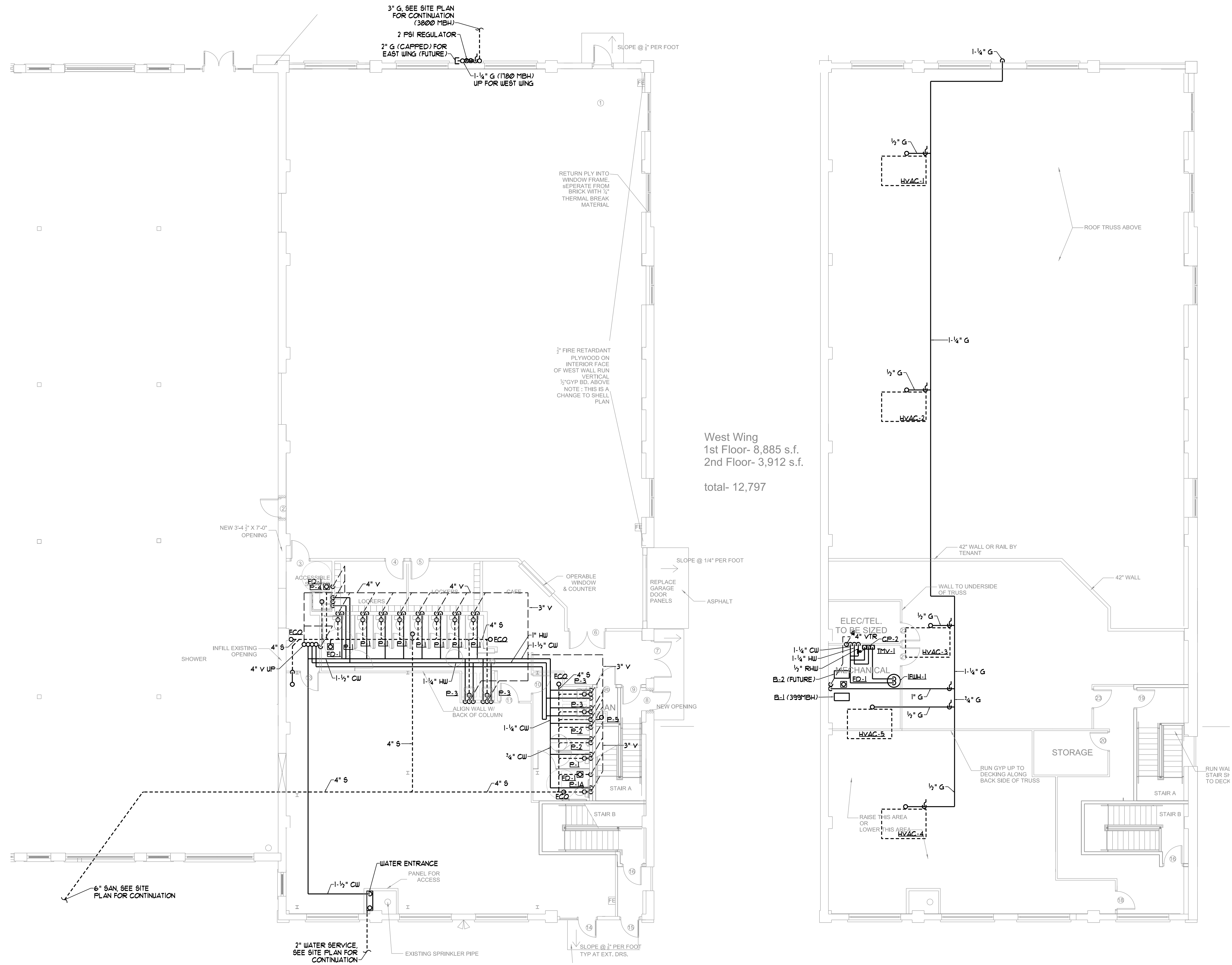
FIRST FLOOR PLUMBING PLAN SCALE - 1/8" = 1'-0"
