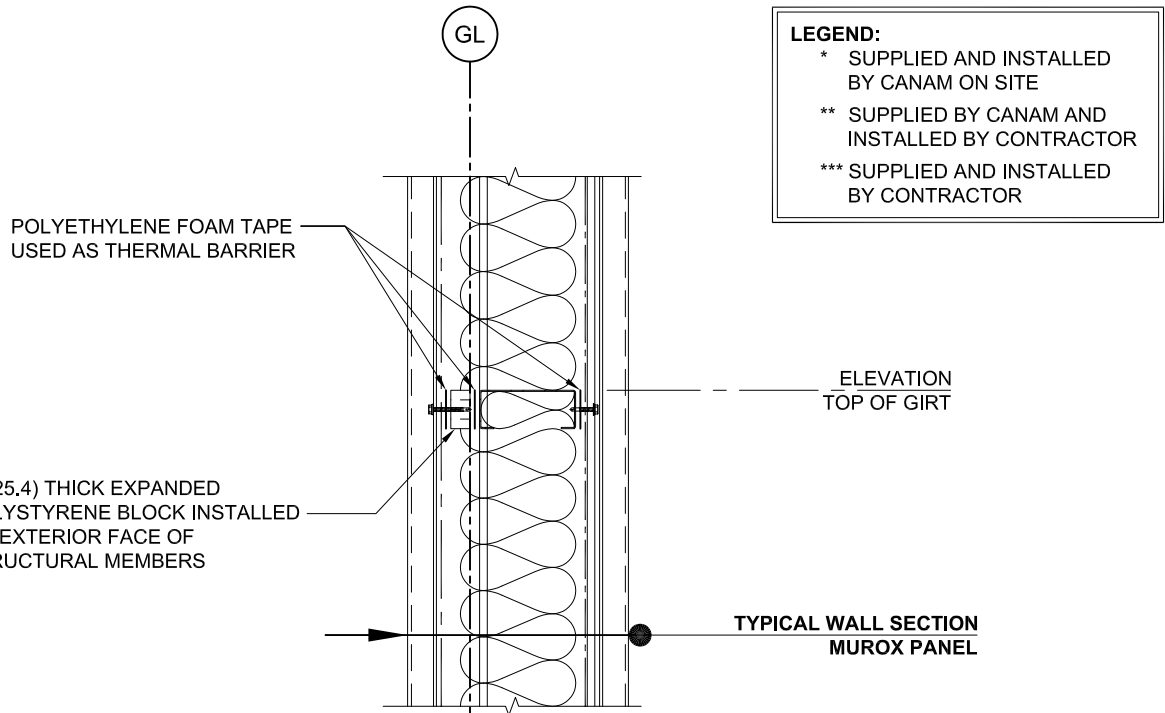
B 2 GIRT - TYPICAL DETAIL
