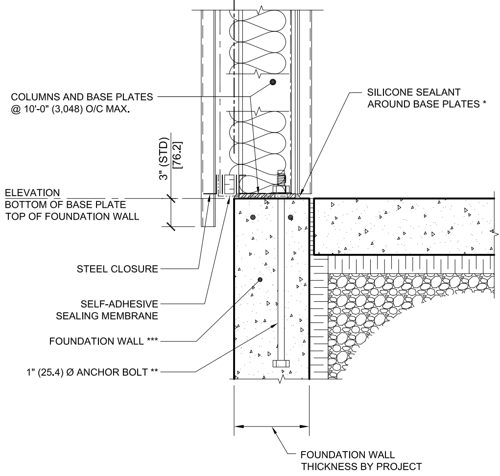
A 2 ANCHOR AT FOUNDATION DETAIL
