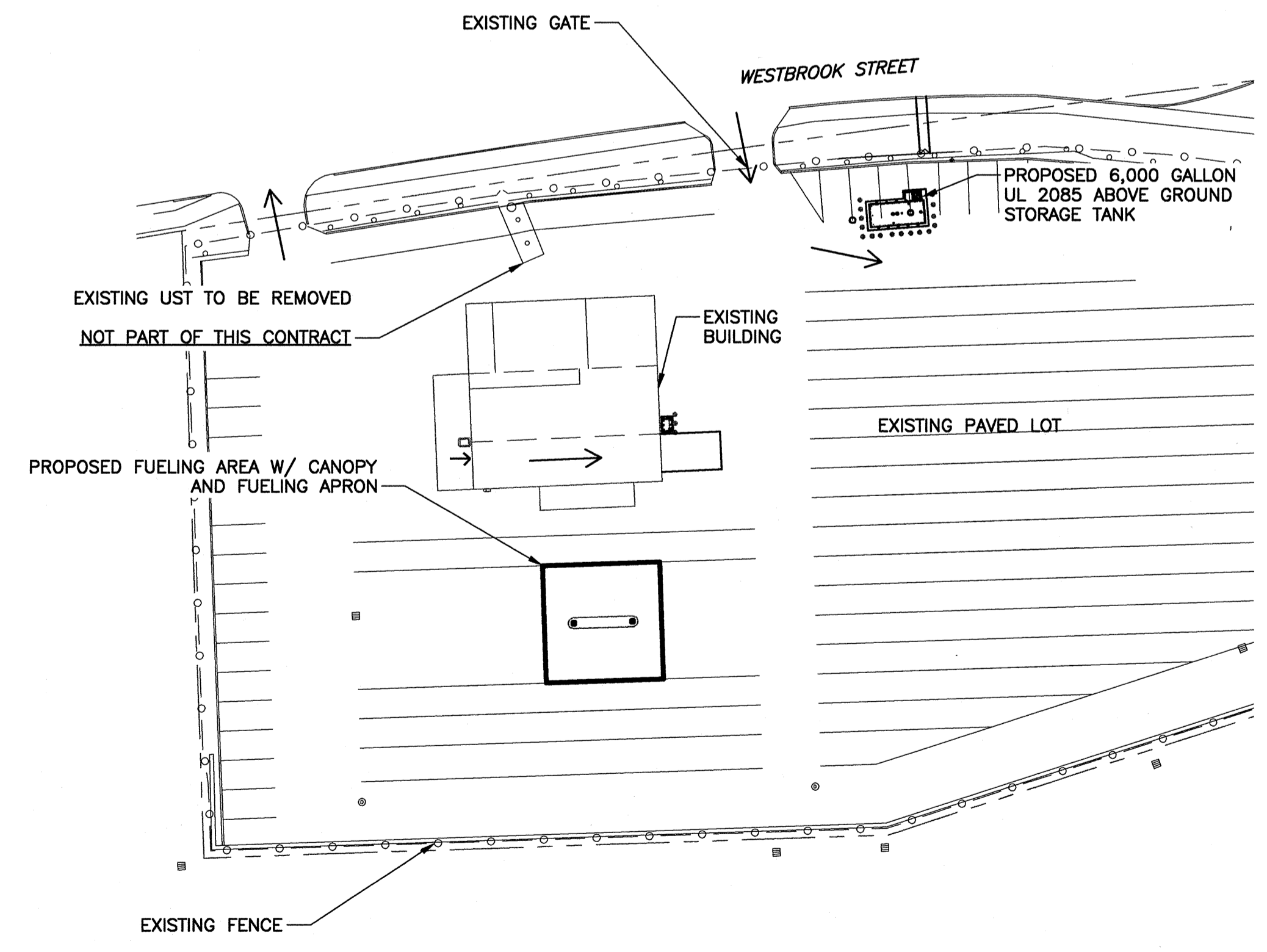
4 SITE KEY PLAN FS.G.3 SCALE: 1"=40'
