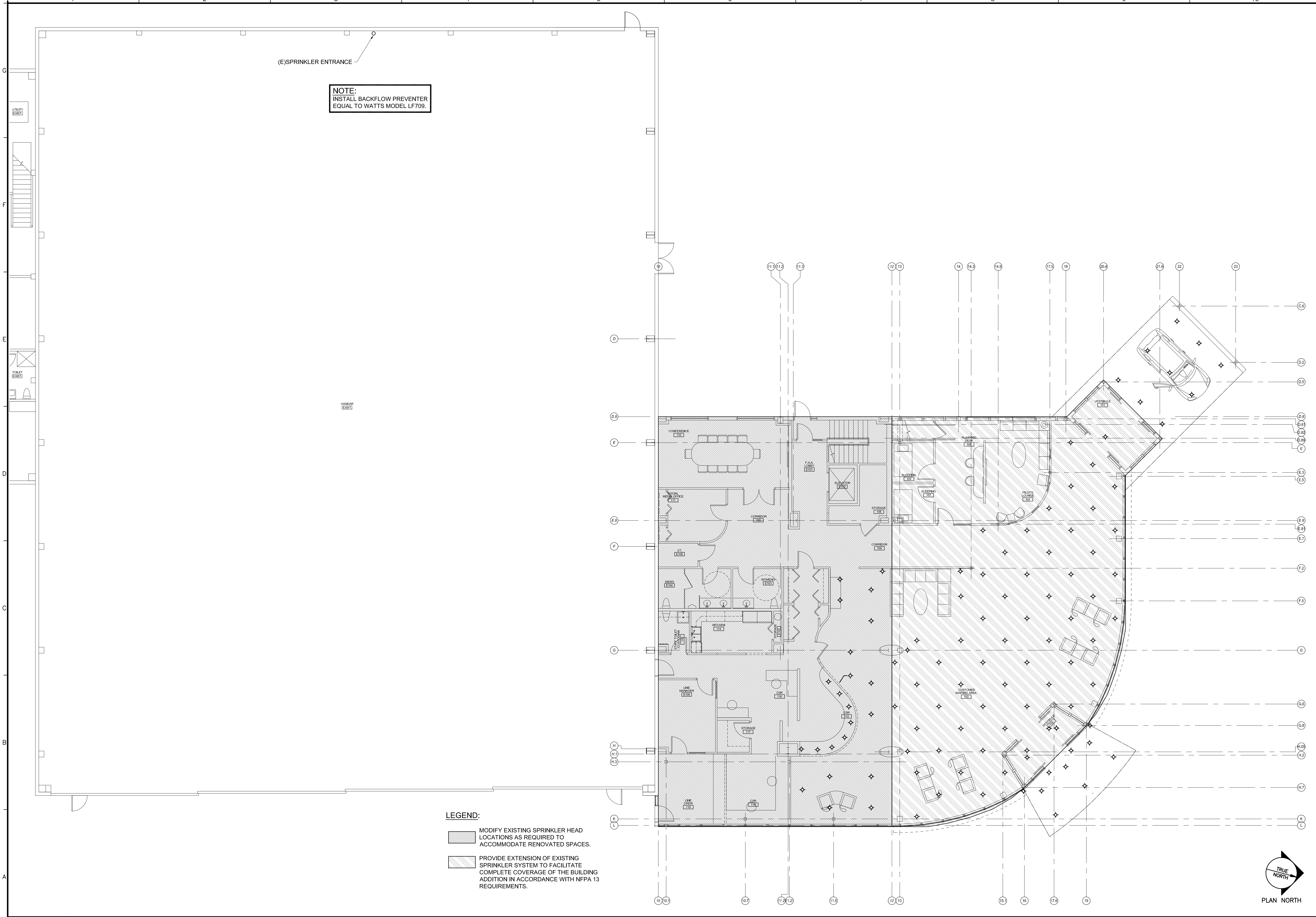
A1 MECHANICAL PLAN 1/8" = 1'-0"
