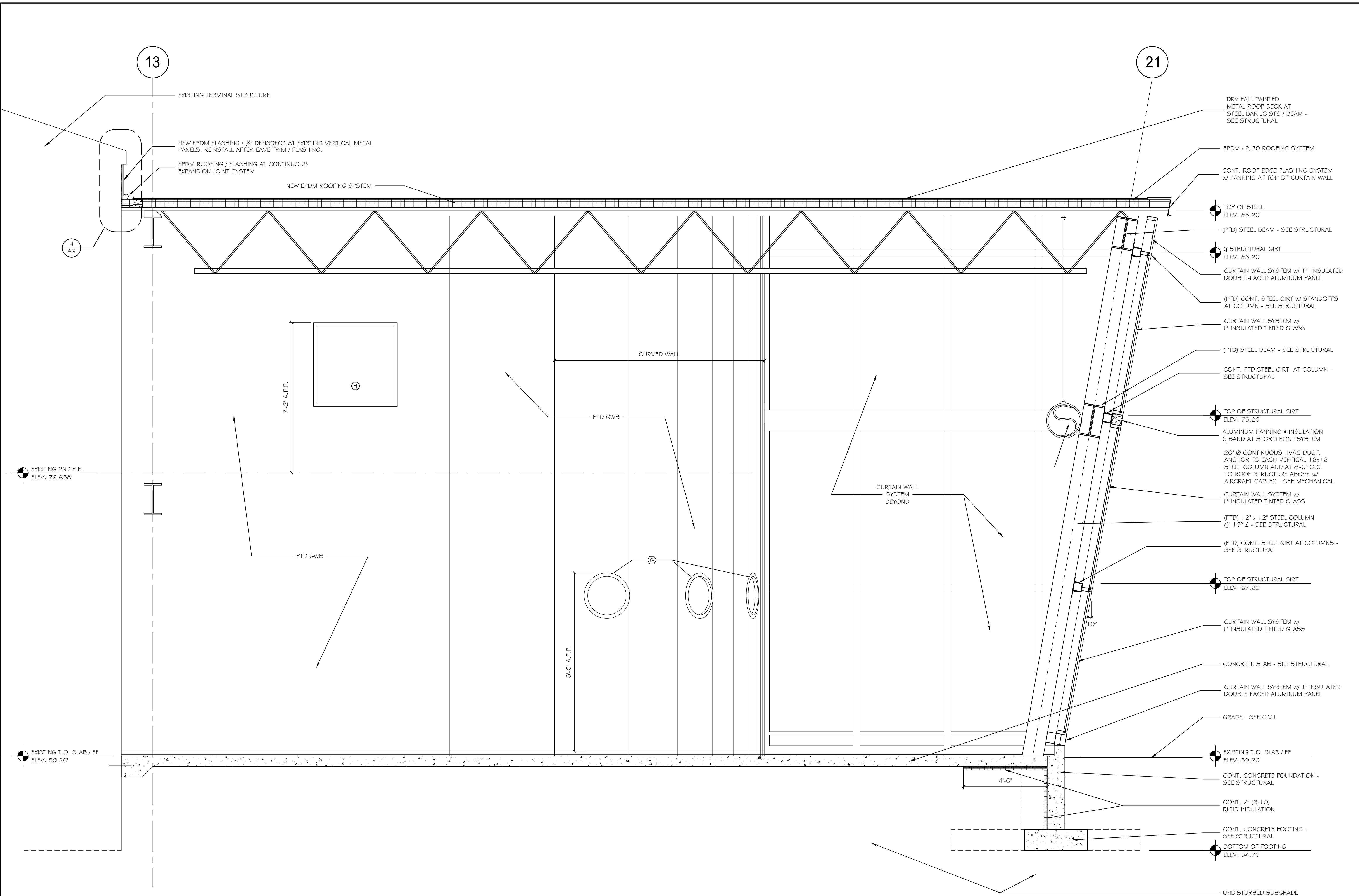
A TYPICAL BUILDING SECTION SCALE: 1/2" = 1'-0"
