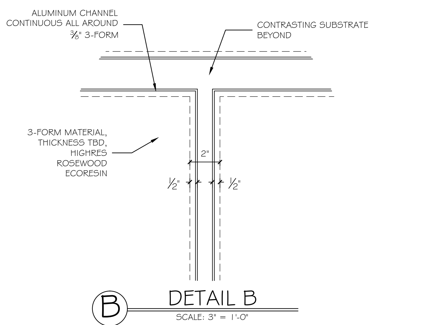
A CSR DESK SECTION SCALE: 1" = 1'-0"
