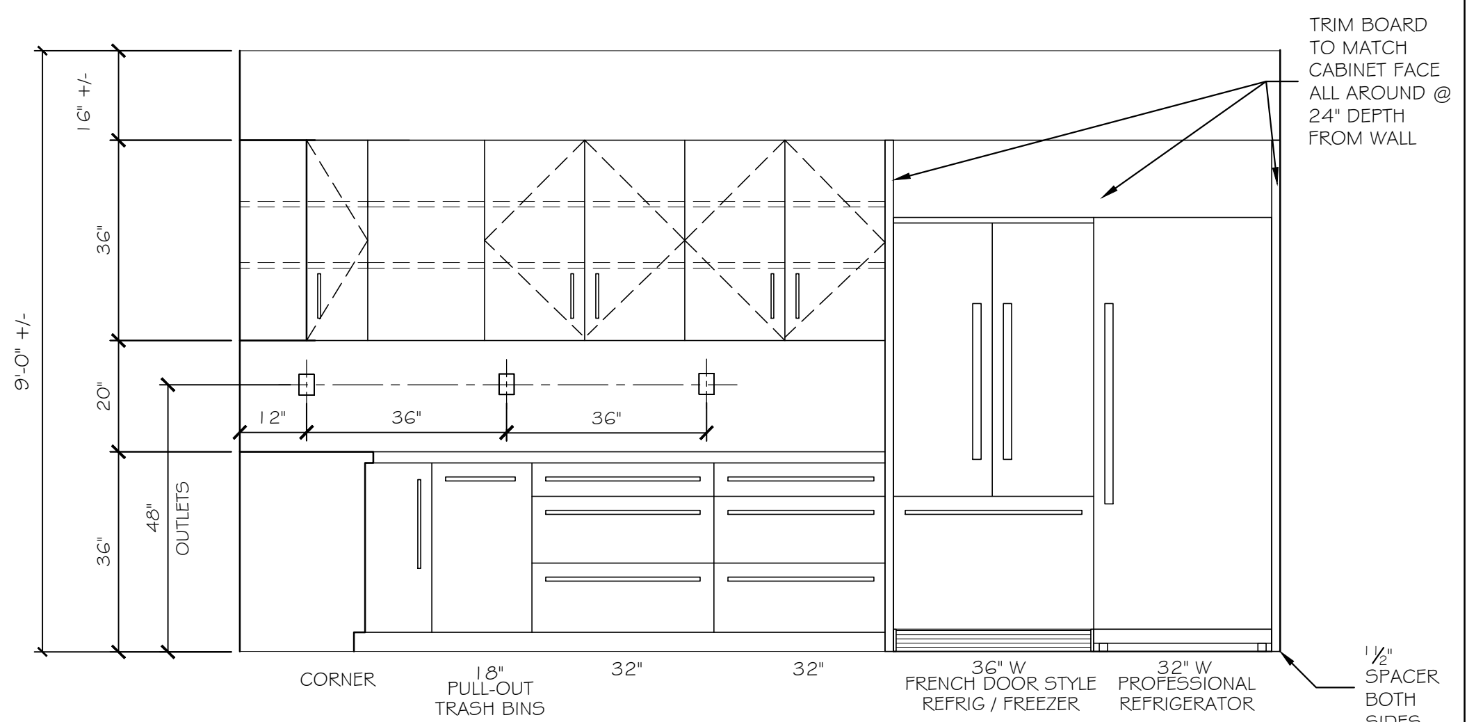
A ELEVATION A
