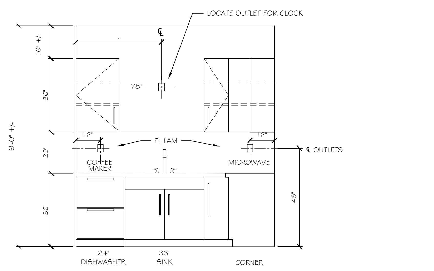
B ELEVATION B
