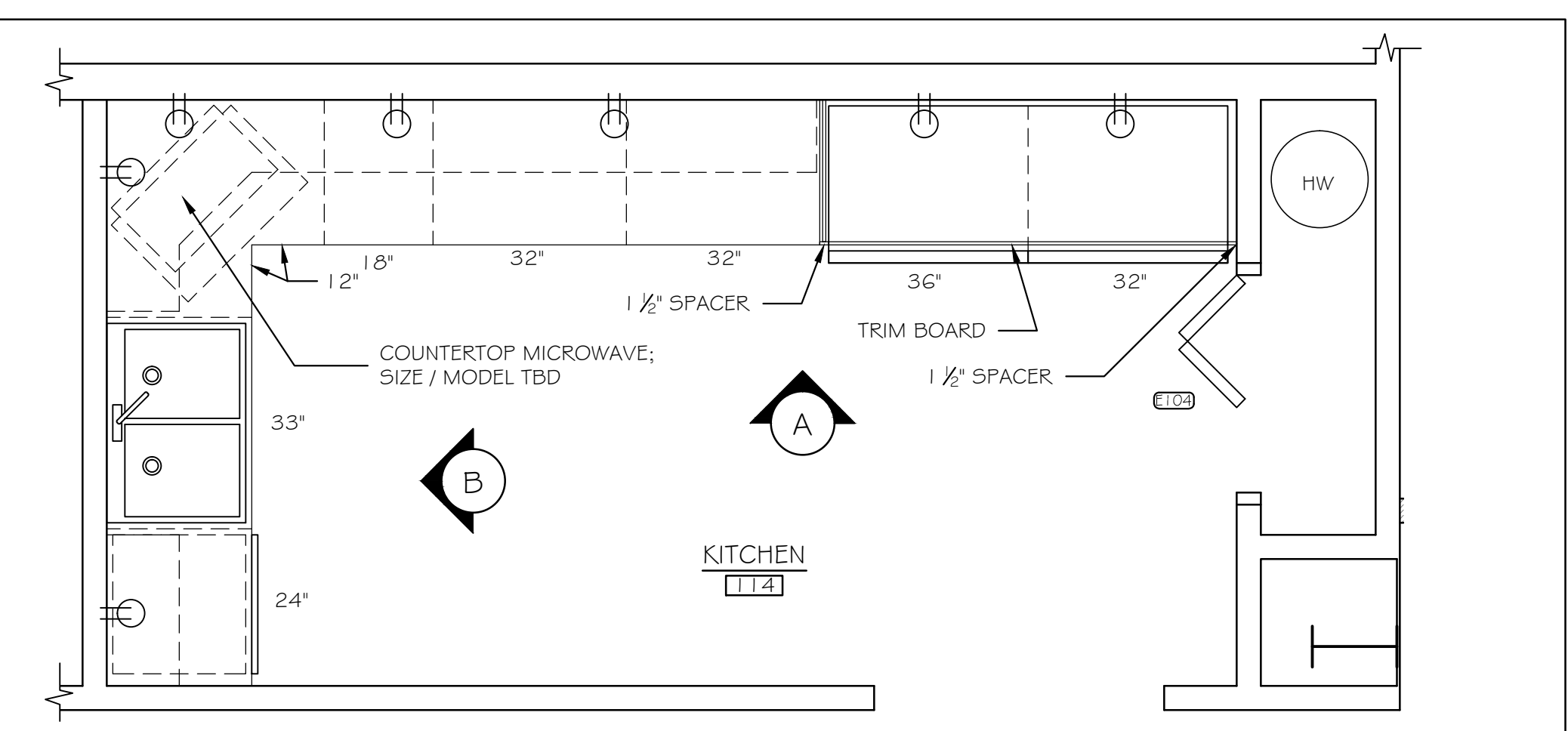
KITCHEN PLAN
