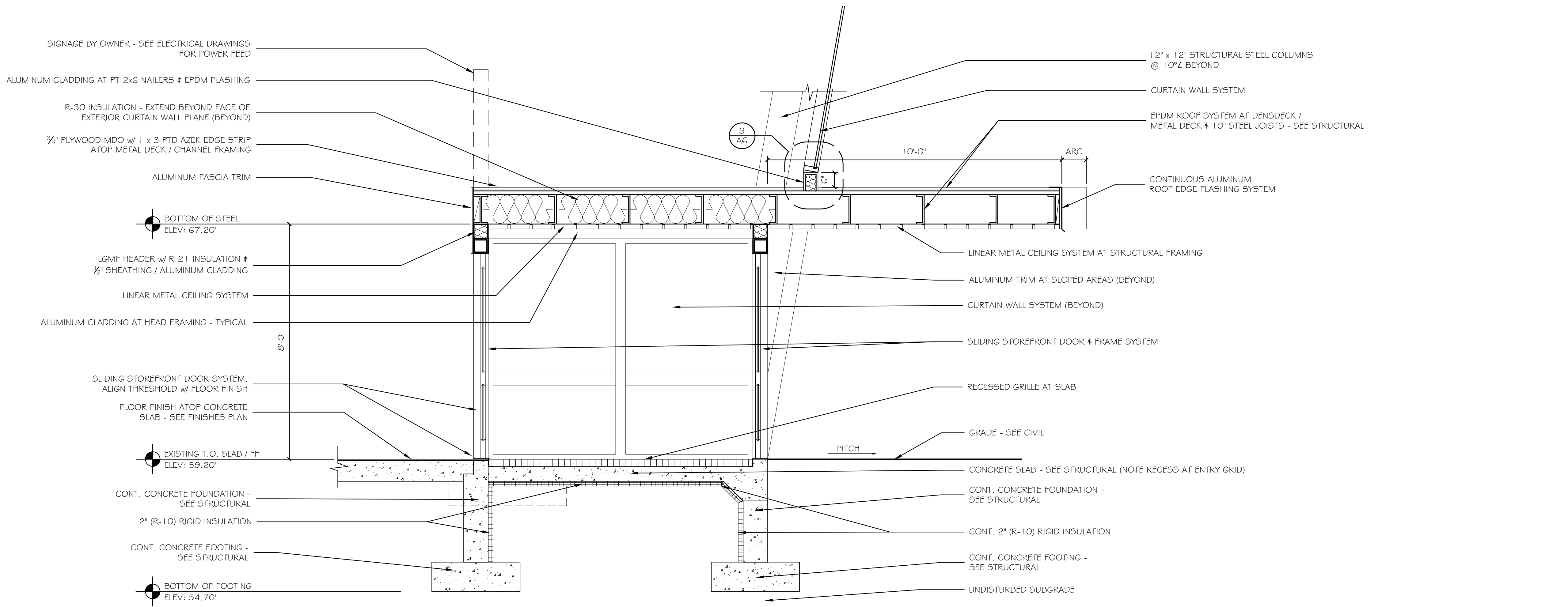
C BUILDING SECTION AT VESTIBULE [T02] SCALE: 1/2" = 1'-0"
