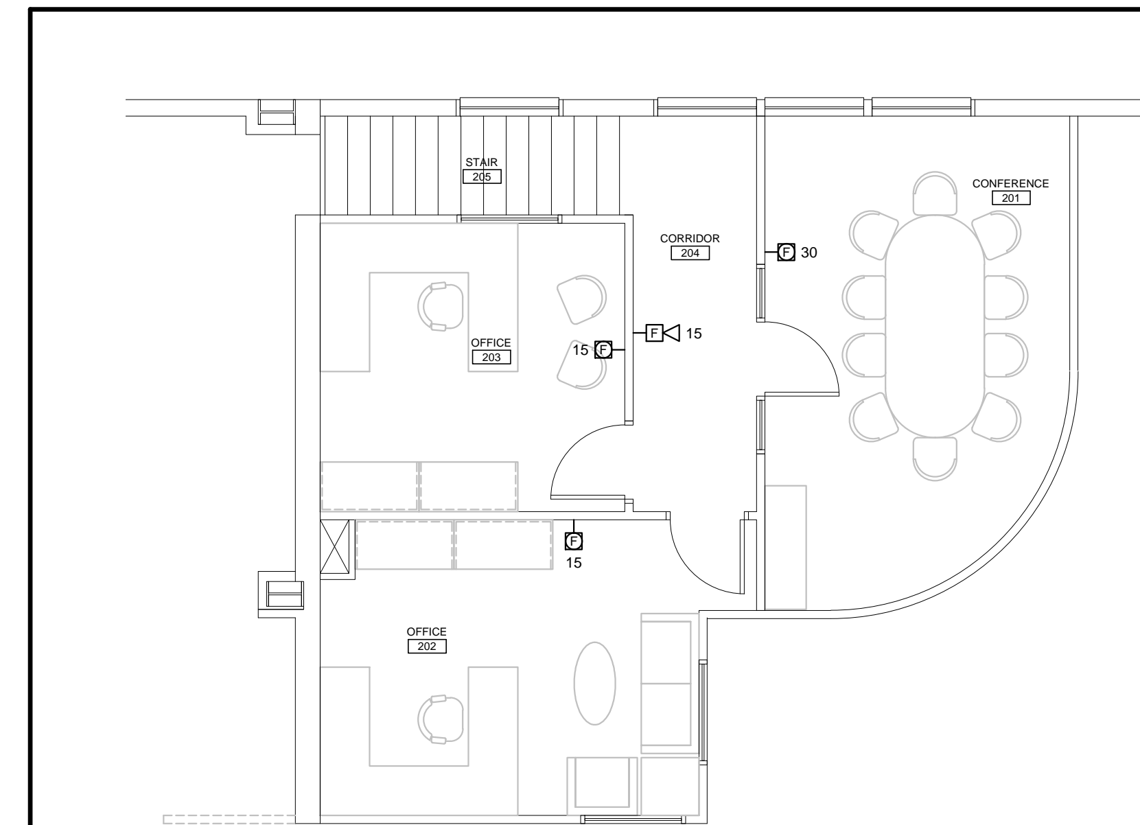
A8 SECOND FLOOR
