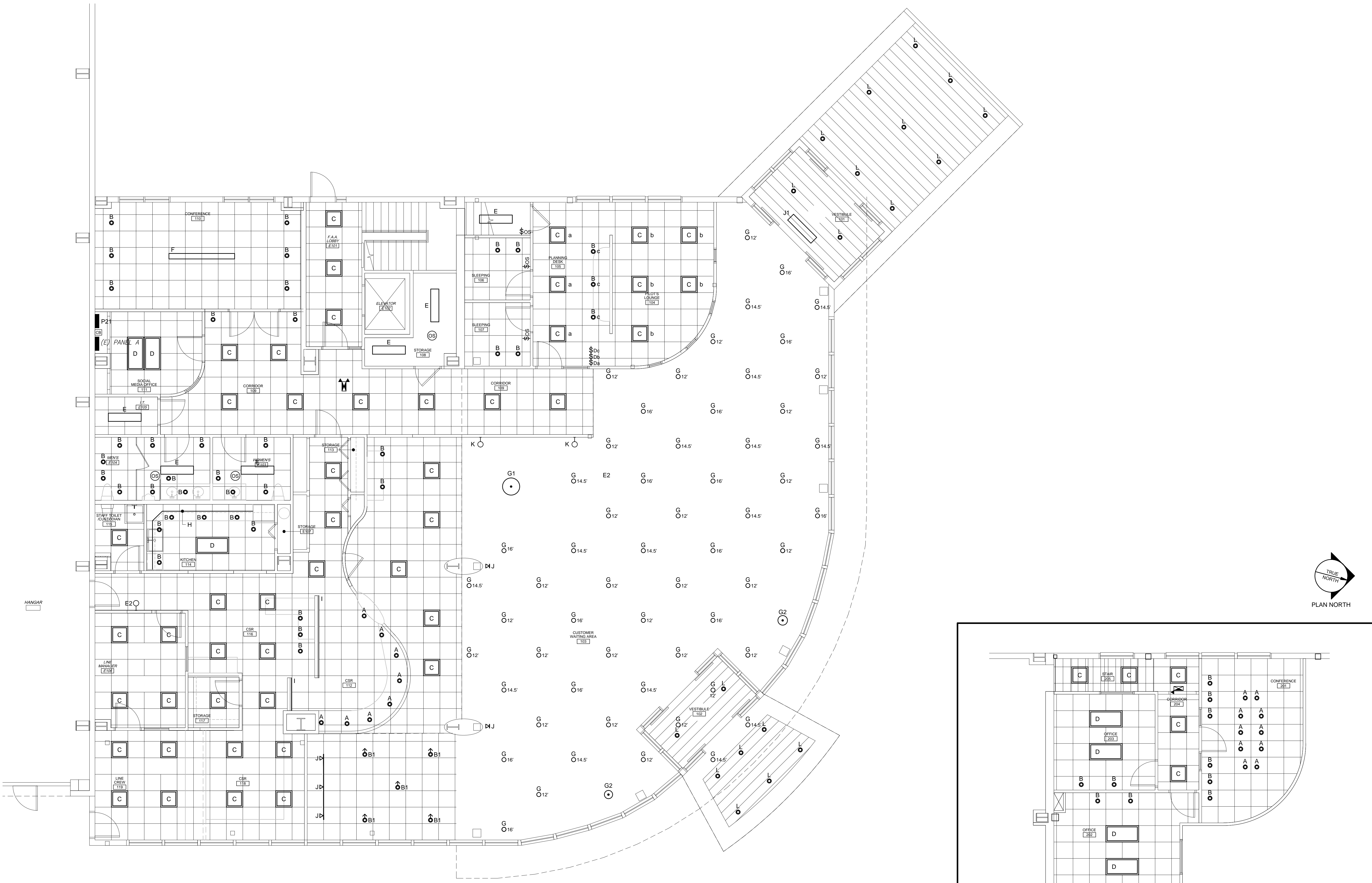
A1 LIGHTING PLAN 3/16" = 1'-0"
