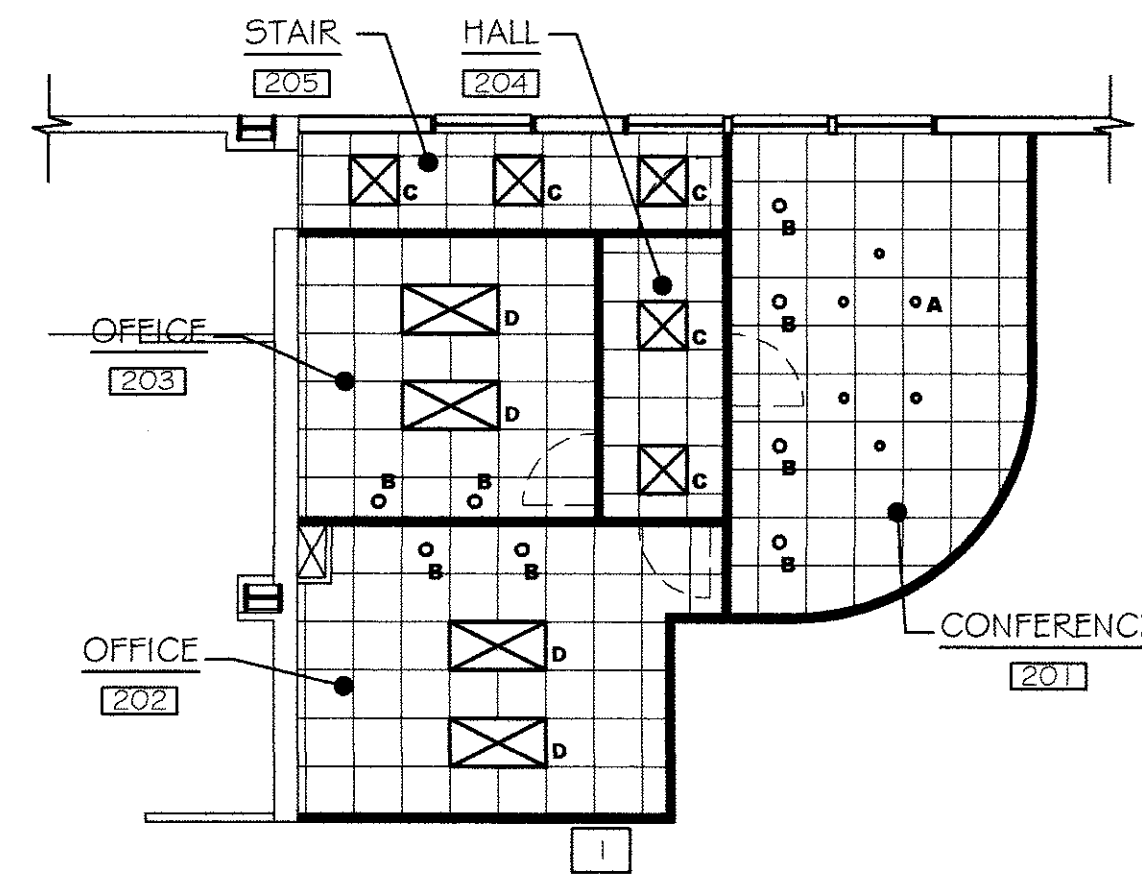
① OFFICES ABOVE PILOT'S SUITE SCALE: 1/8" = 1'-0"
