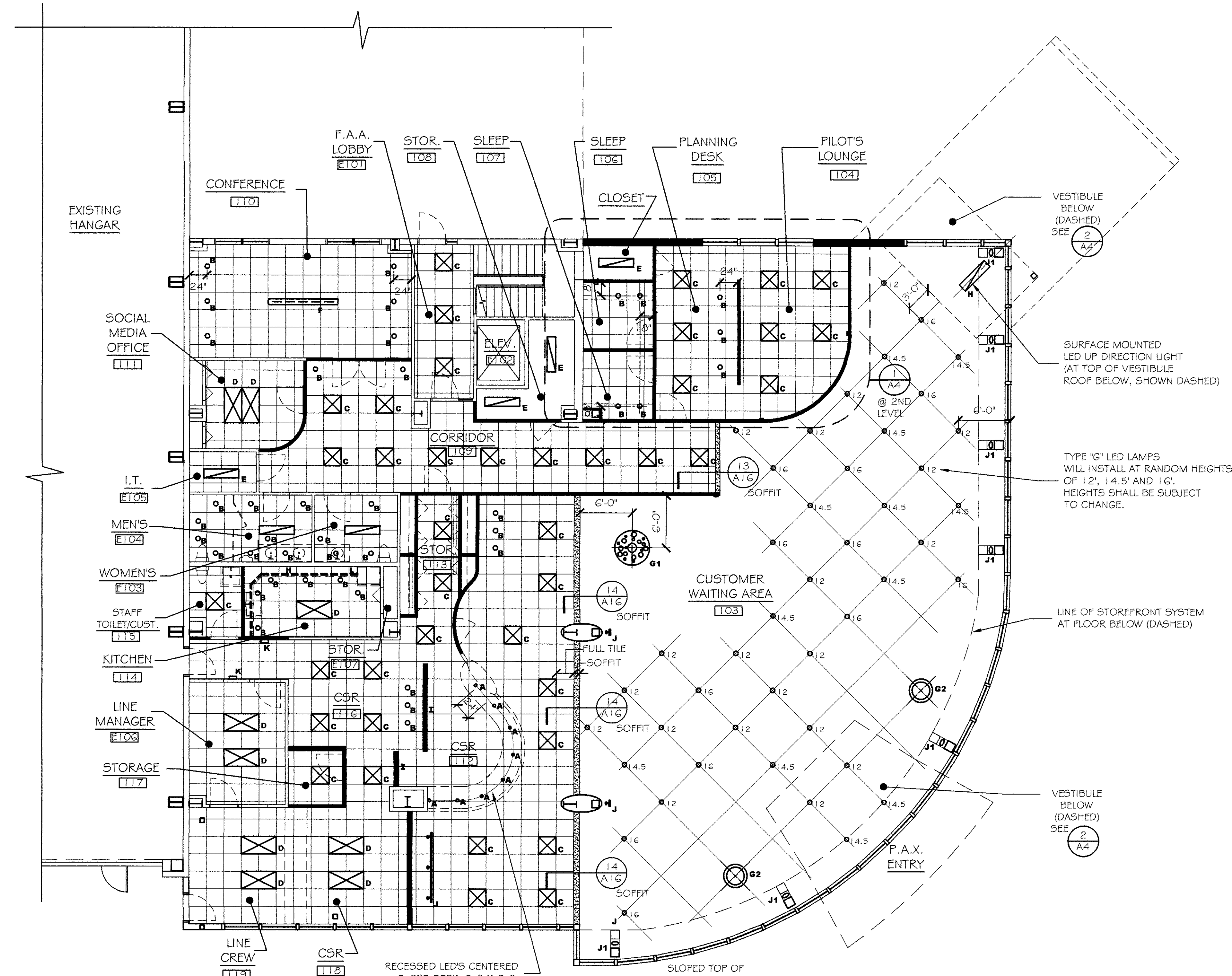
① OFFICES ABOVE PILOT'S SUITE SCALE: 1/8" = 1'-0"
