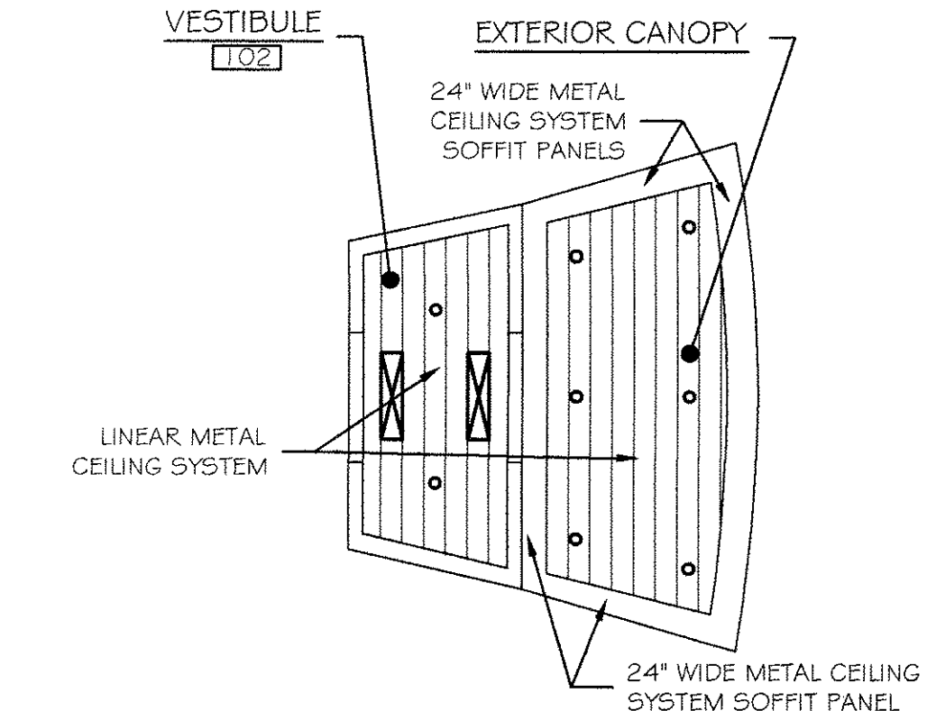
③ VESTIBULE 102 REFLECTED CEILING PLAN SCALE: 1/8" = 1'-0"
