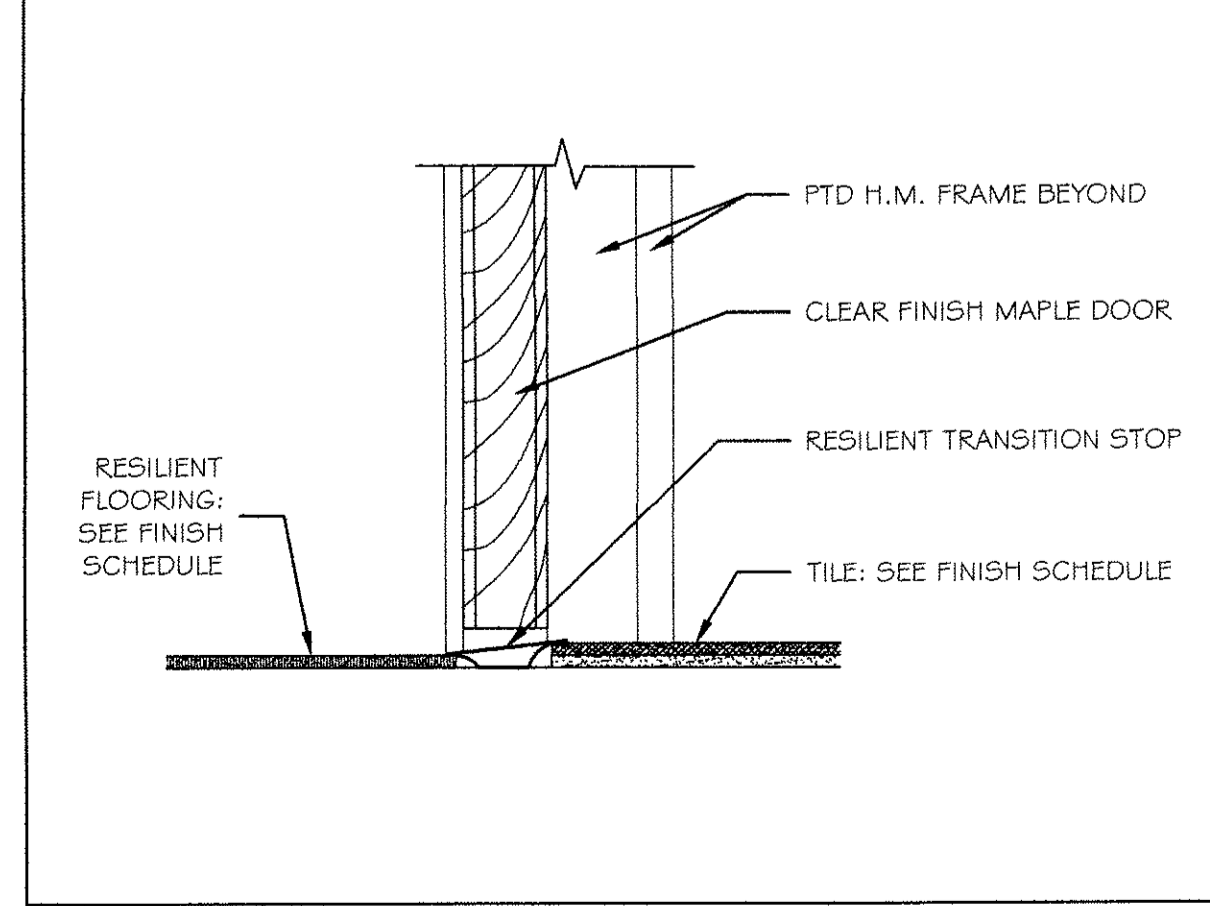
17 INTERIOR SILL DETAIL AT DOOR 3" = 1'-0"
