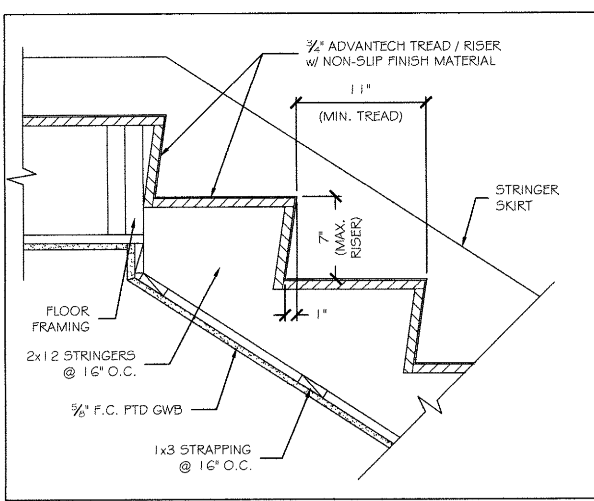
1 INTERIOR STAIR RISER / TREAD DETAIL 1/2" = 1'-0"
