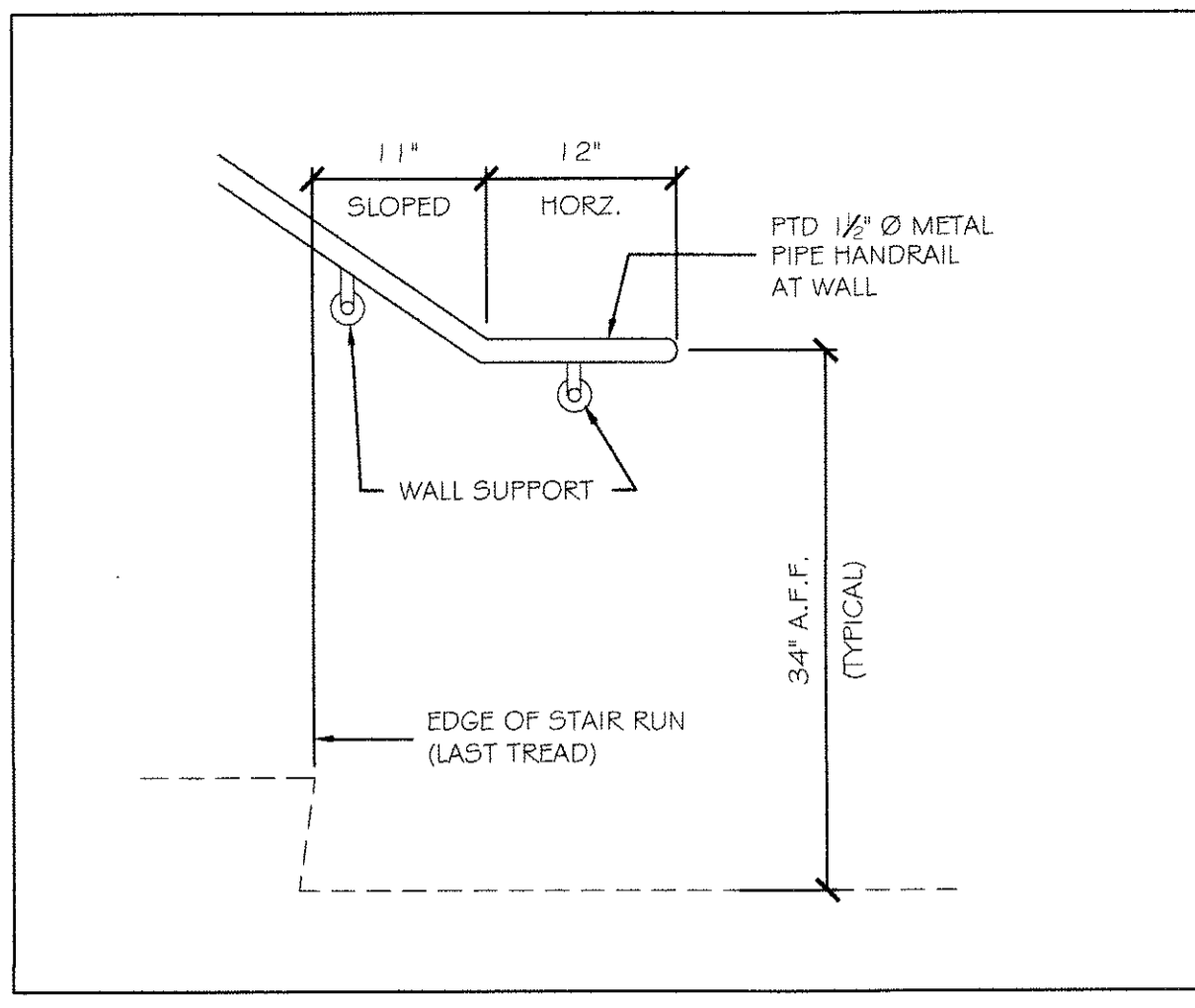
4 TYPICAL WALL HANDRAIL - BOTTOM 1" = 1'-0"
