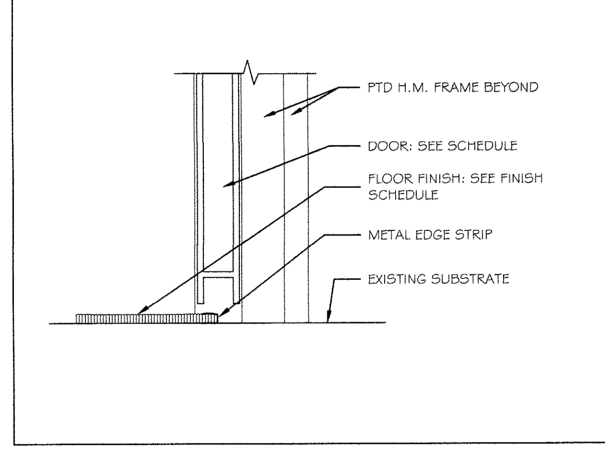
20 INTERIOR SILL DETAIL AT DOOR 3" = 1'-0"
