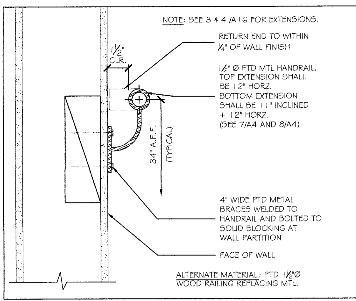
2 TYPICAL WALL HANDRAIL SECTION 3" = 1'-0"
