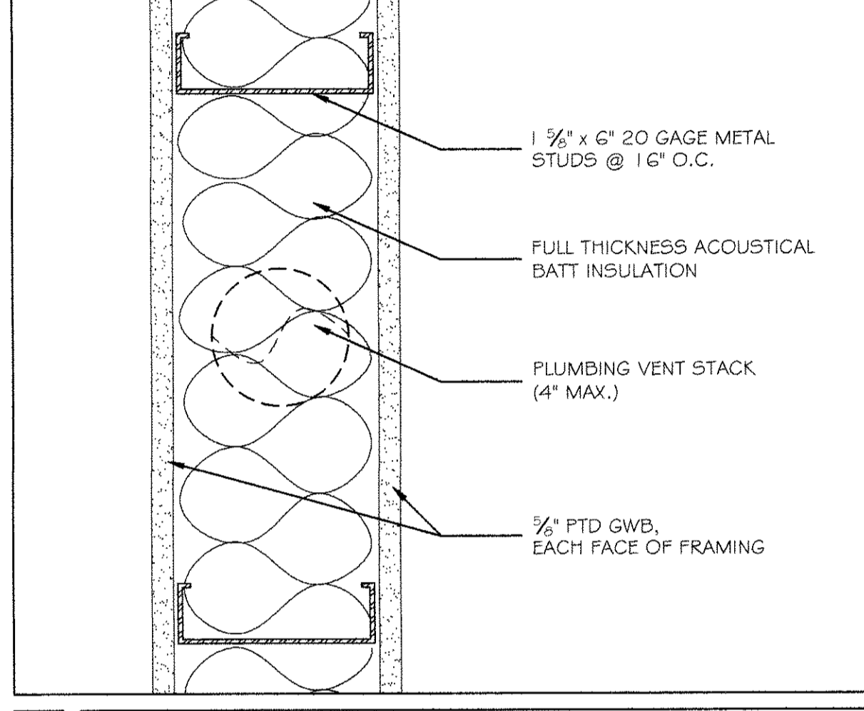
10 TYPICAL PARTITION 3" = 1'-0"
