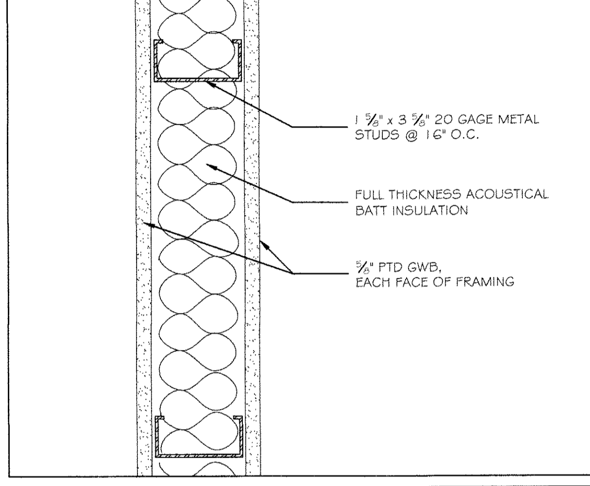
9 TYPICAL PARTITION 3" = 1'-0"
