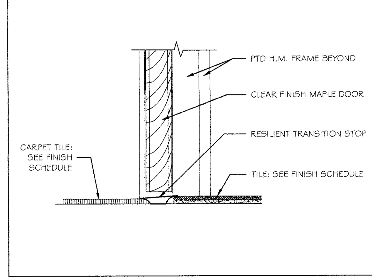
18 INTERIOR SILL DETAIL AT DOOR 3" = 1'-0"
