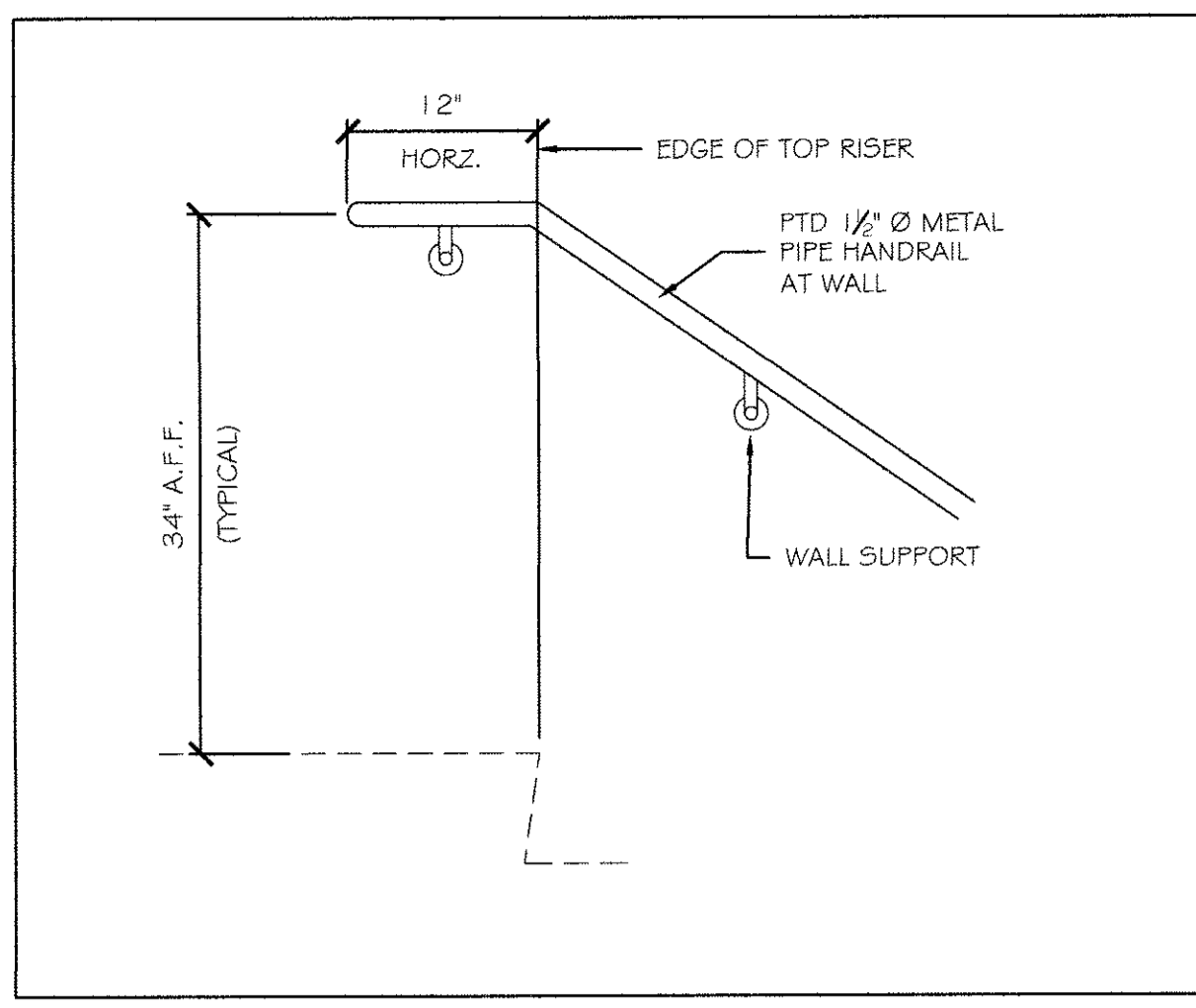
3 TYPICAL WALL HANDRAIL - TOP 1" = 1'-0"
