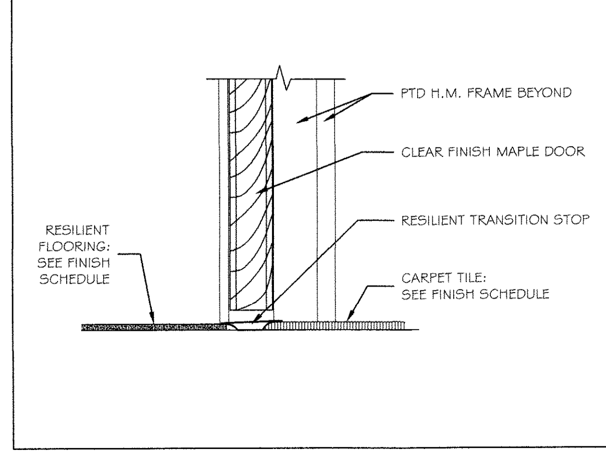
19 INTERIOR SILL DETAIL AT DOOR 3" = 1'-0"
