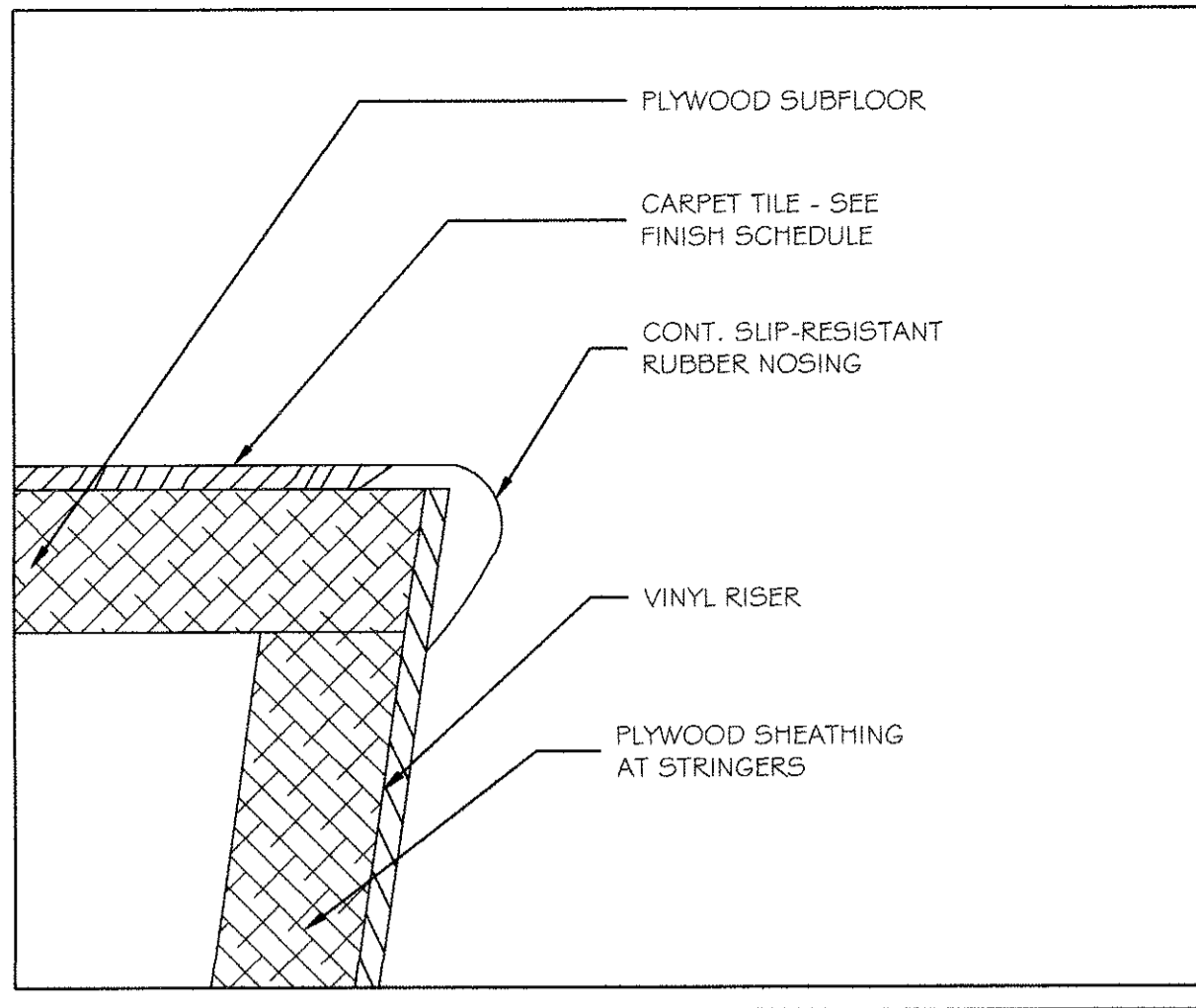
5 STAIR NOSING DETAIL FULL SIZE
