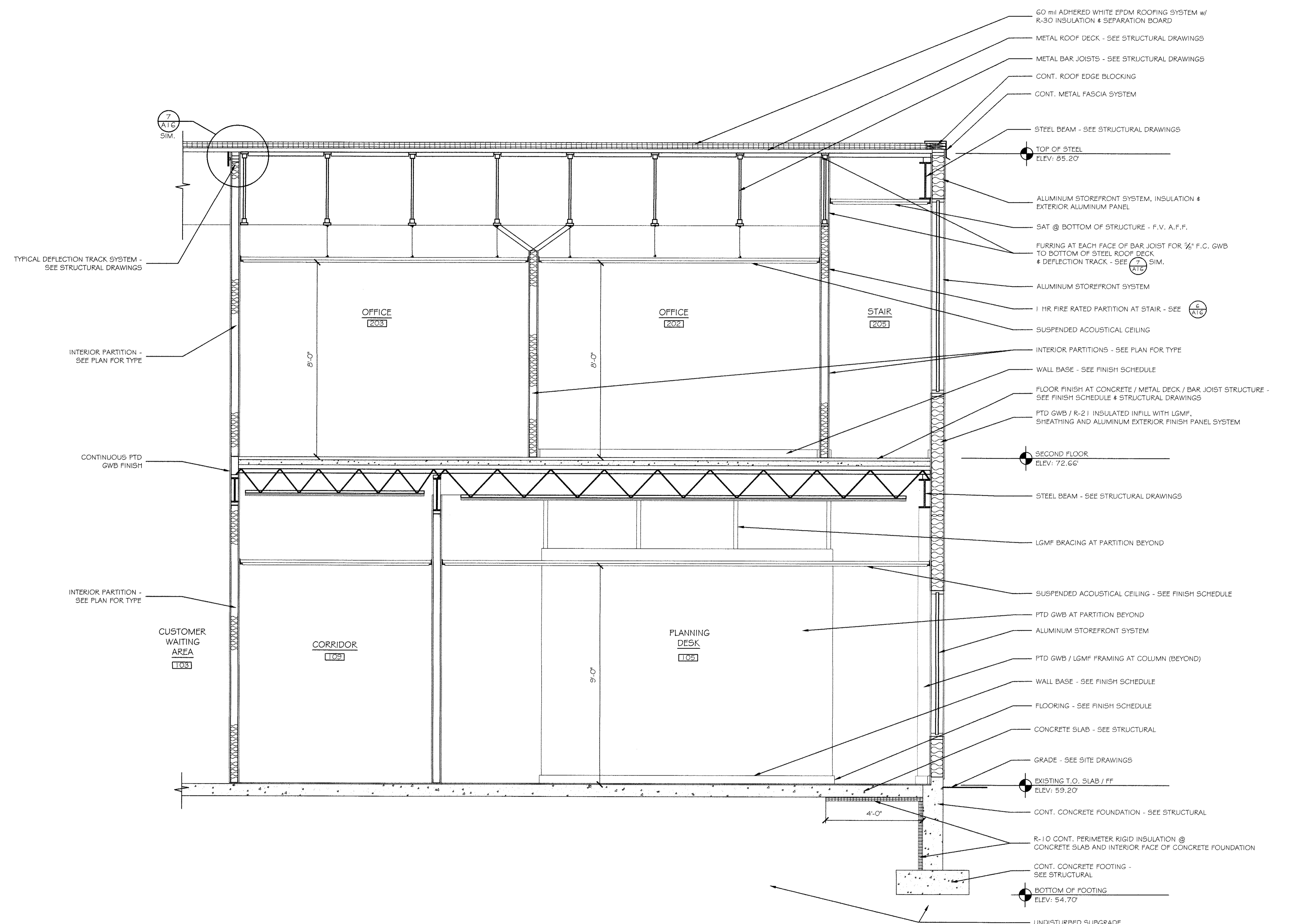
D BUILDING SECTION AT PLANNING DESK 105 & OFFICES 202 / 203
