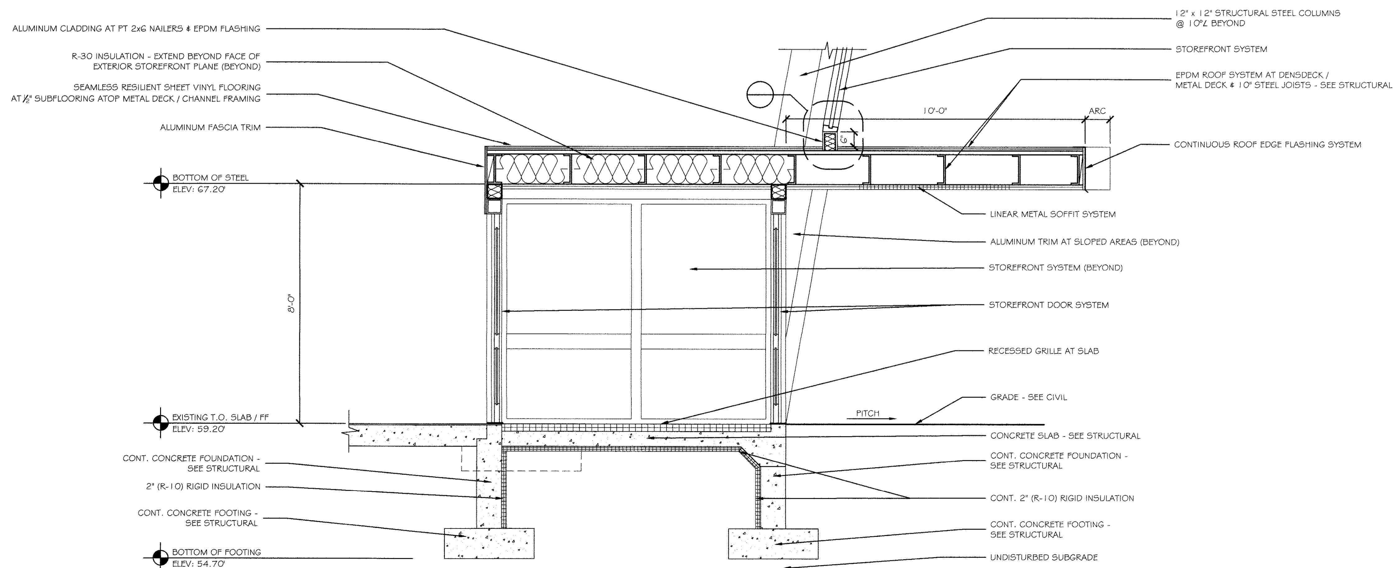
C BUILDING SECTION AT VESTIBULE [T03] SCALE: 1/2" = 1'-0"
