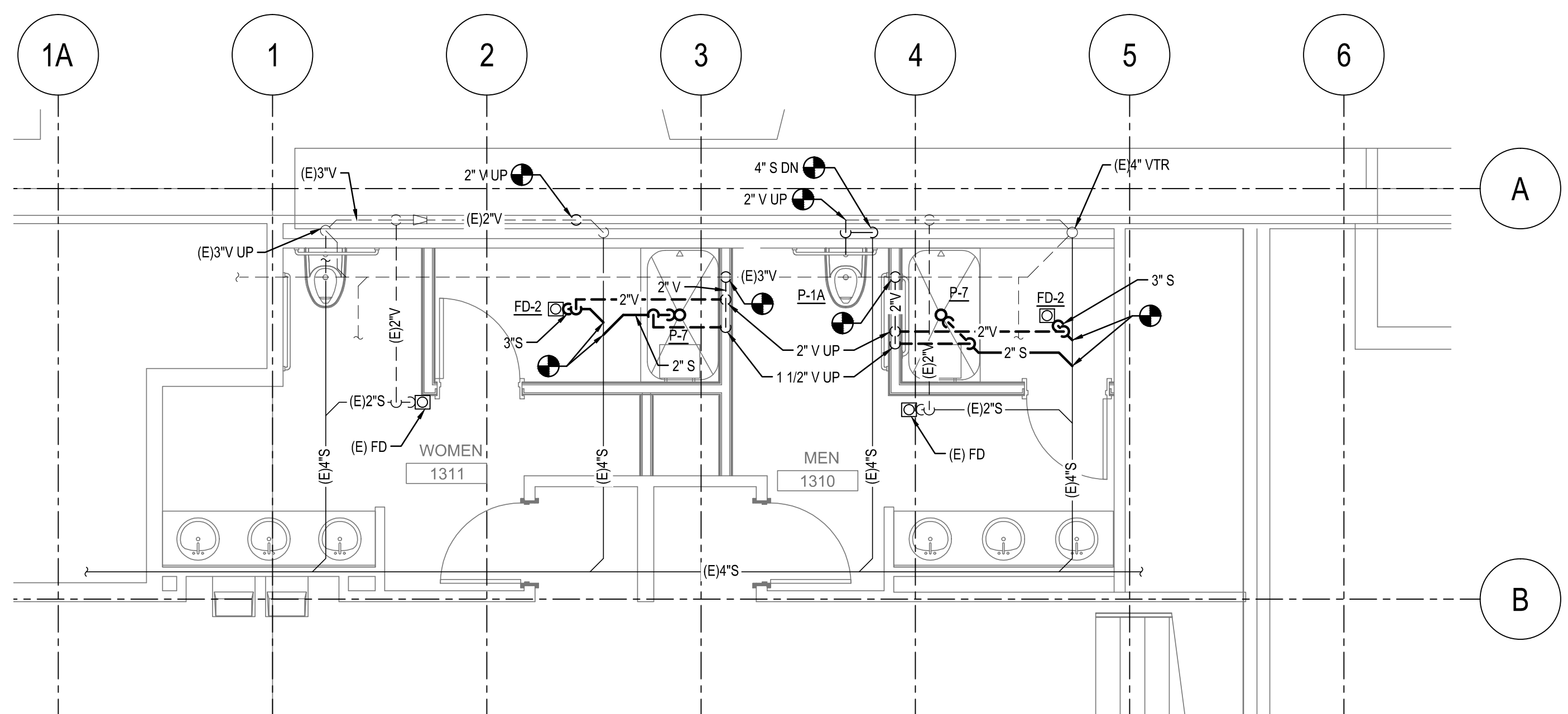
LEVEL 1 TOILET ROOM DRAIN, WASTE, & VENT PLAN SCALE: 1/4" = 1'-0" 3
