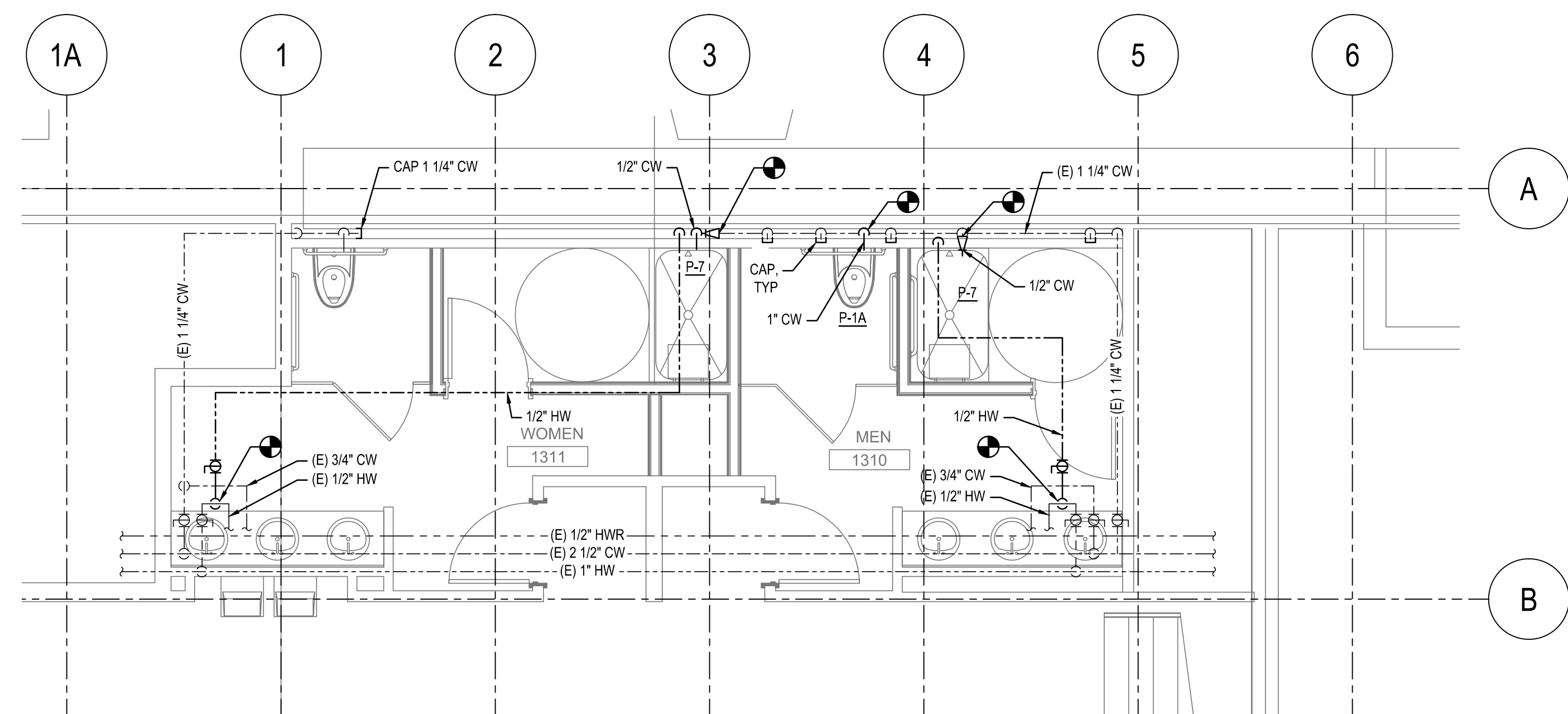
LEVEL 1 TOILET ROOM DOMESTIC WATER PLAN SCALE: 1/4" = 1'-0" 5
