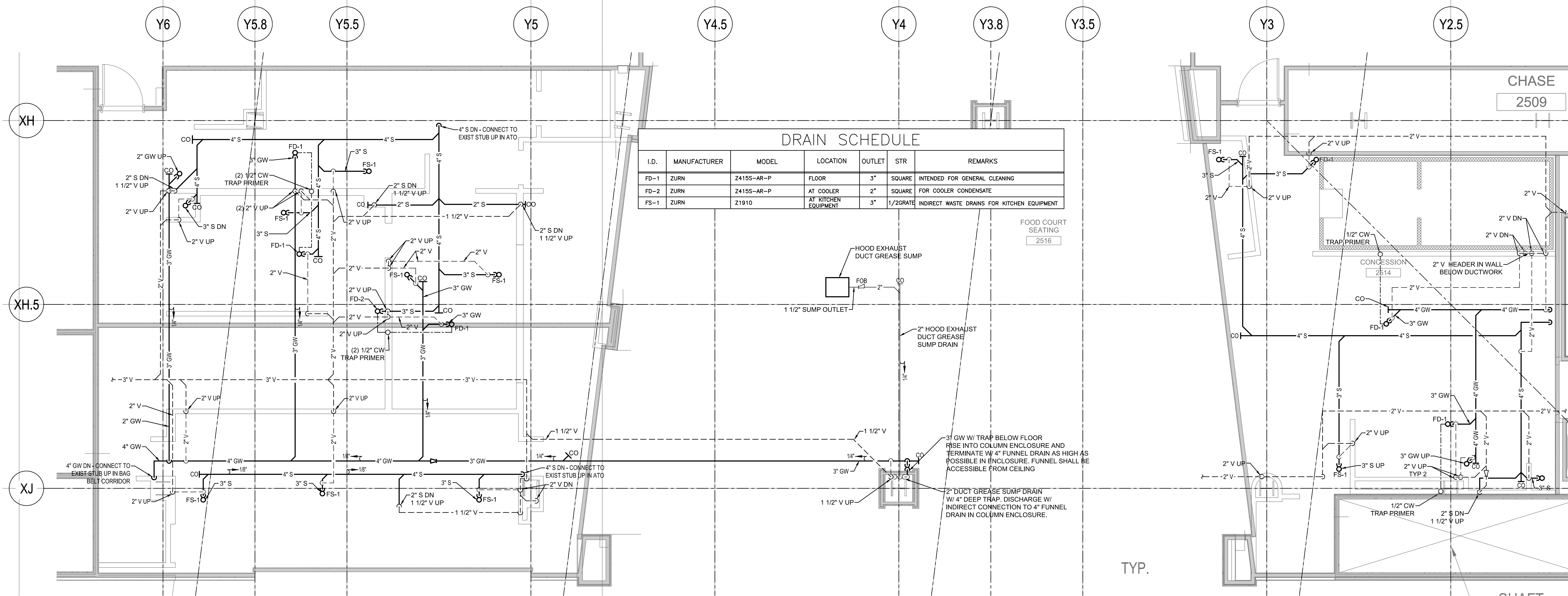
LEVEL 3 CONCESSIONS DRAIN, WASTE & VENT ENLARGED PLAN SCALE: 1/4" = 1'-0" 1
