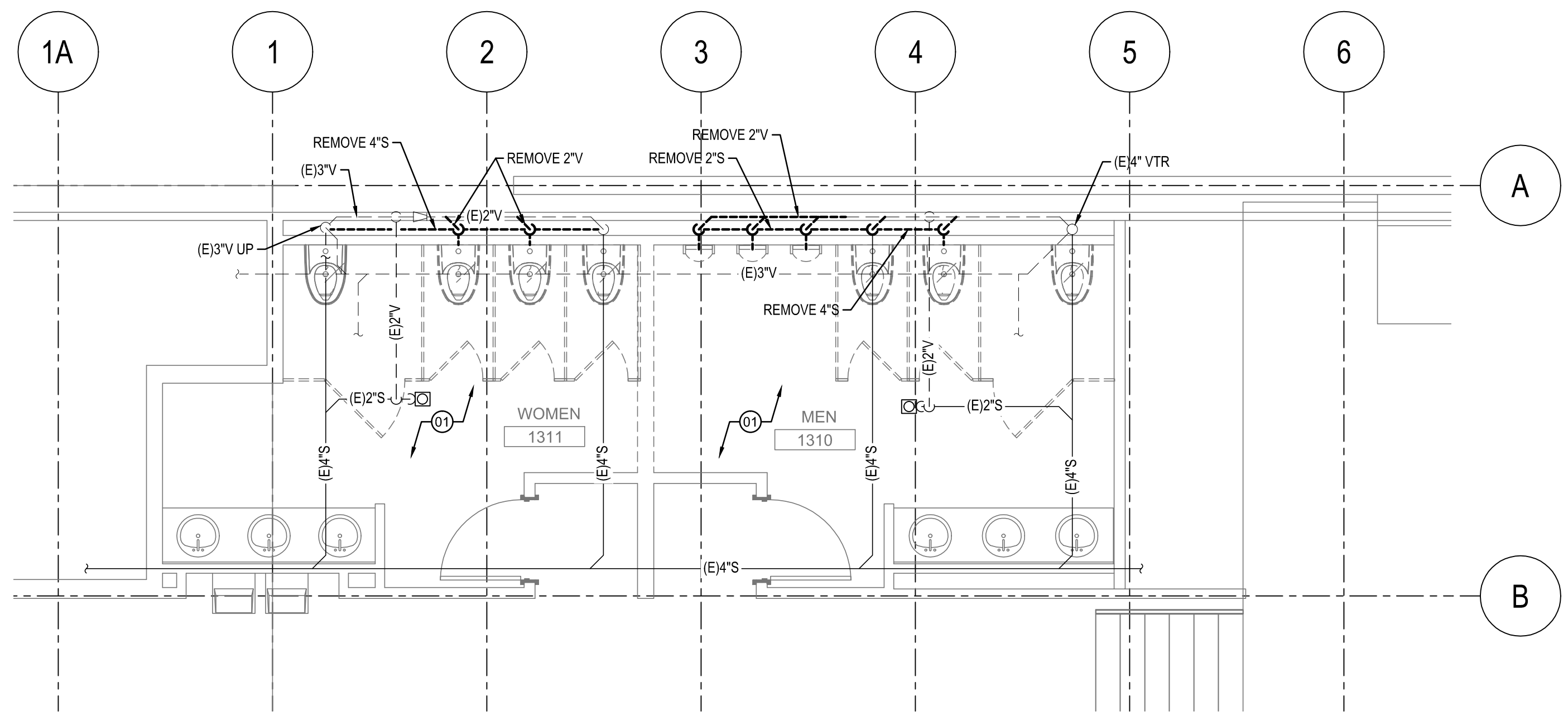
LEVEL 1 TOILET ROOM DRAIN, WASTE, & VENT DEMOLITION PLAN SCALE: 1/4" = 1'-0" 2
