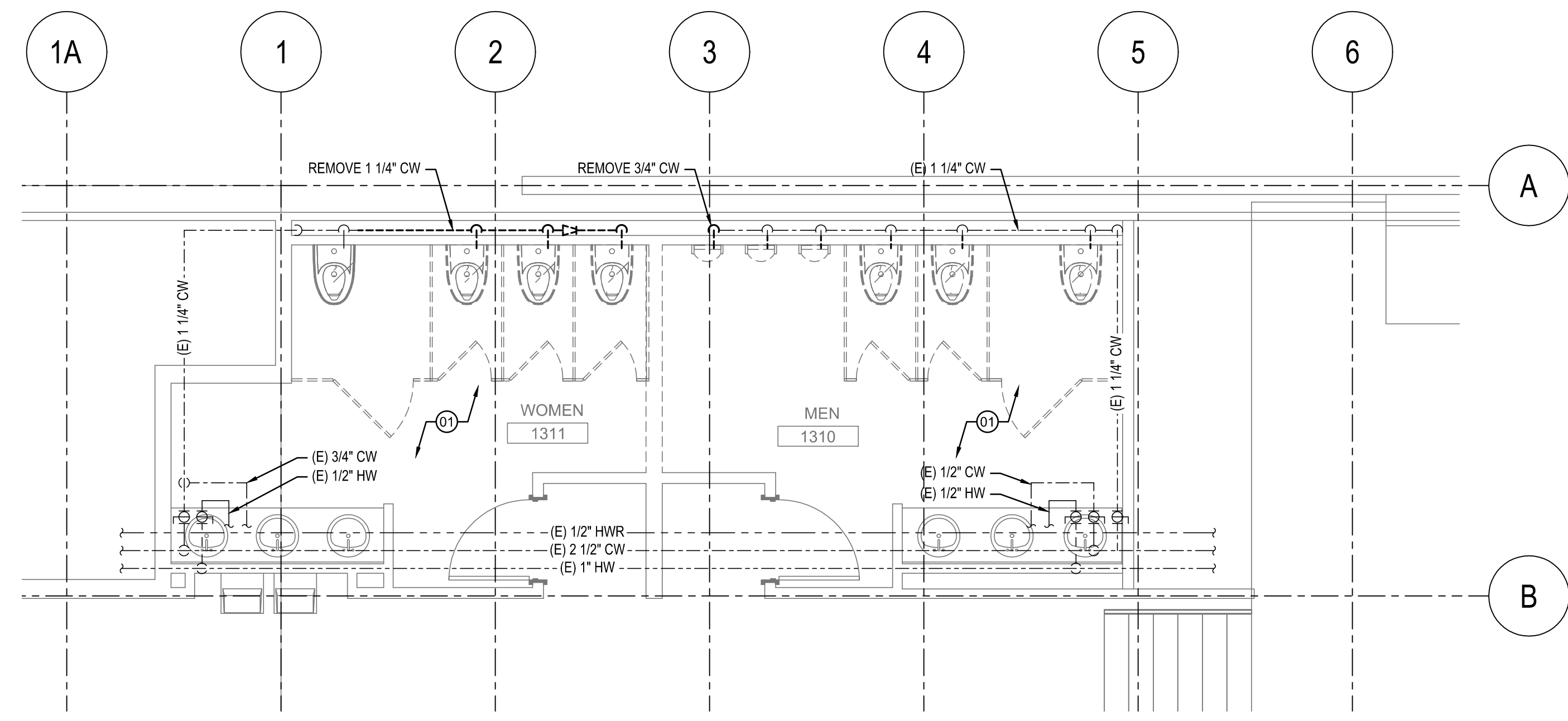
LEVEL 1 TOILET ROOM DOMESTIC WATER DEMOLITION PLAN SCALE: 1/4" = 1'-0" 4
