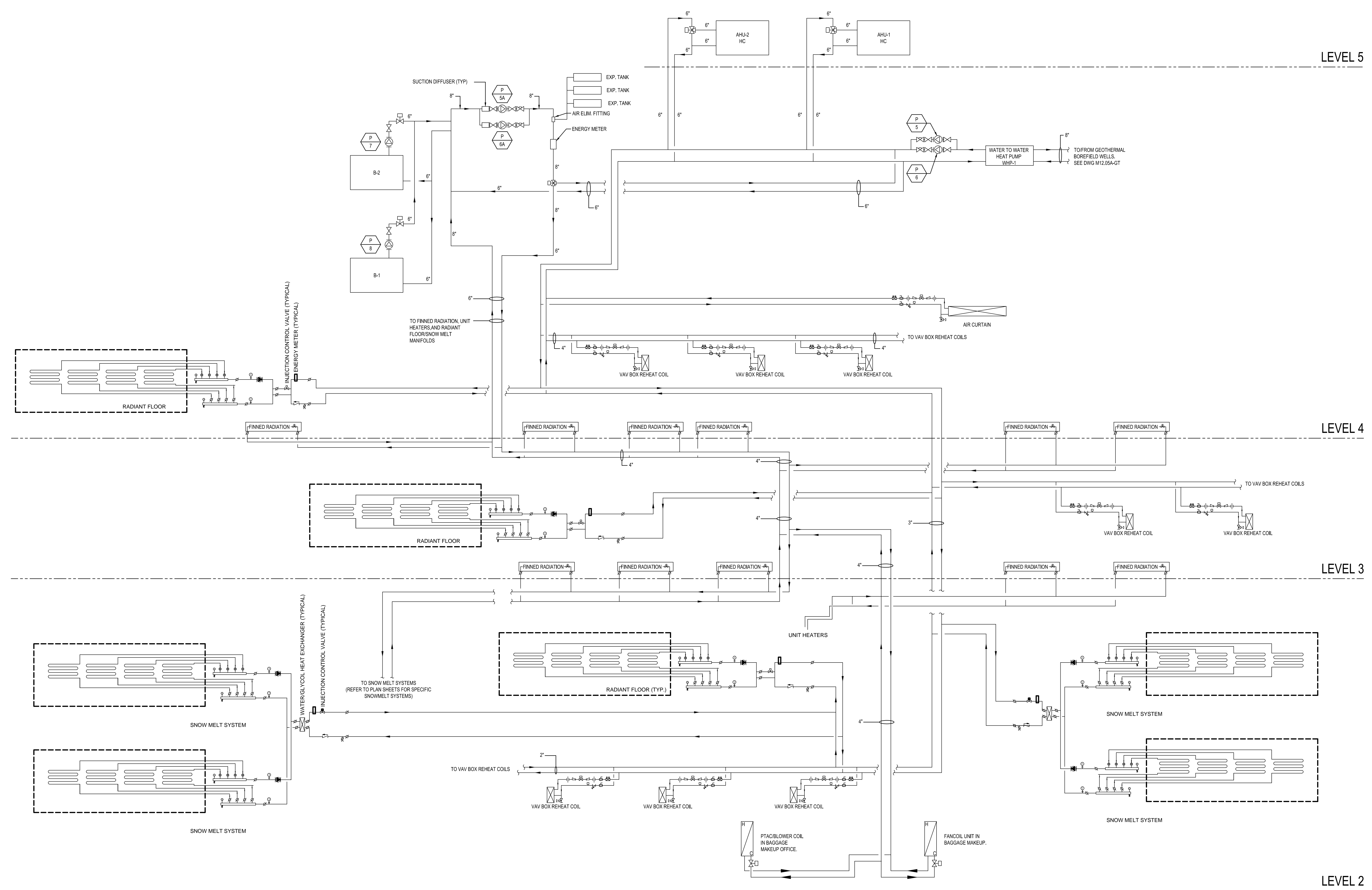
MECHANICAL PIPING SYSTEM SCHEMATIC SCALE: NOT TO SCALE 1
