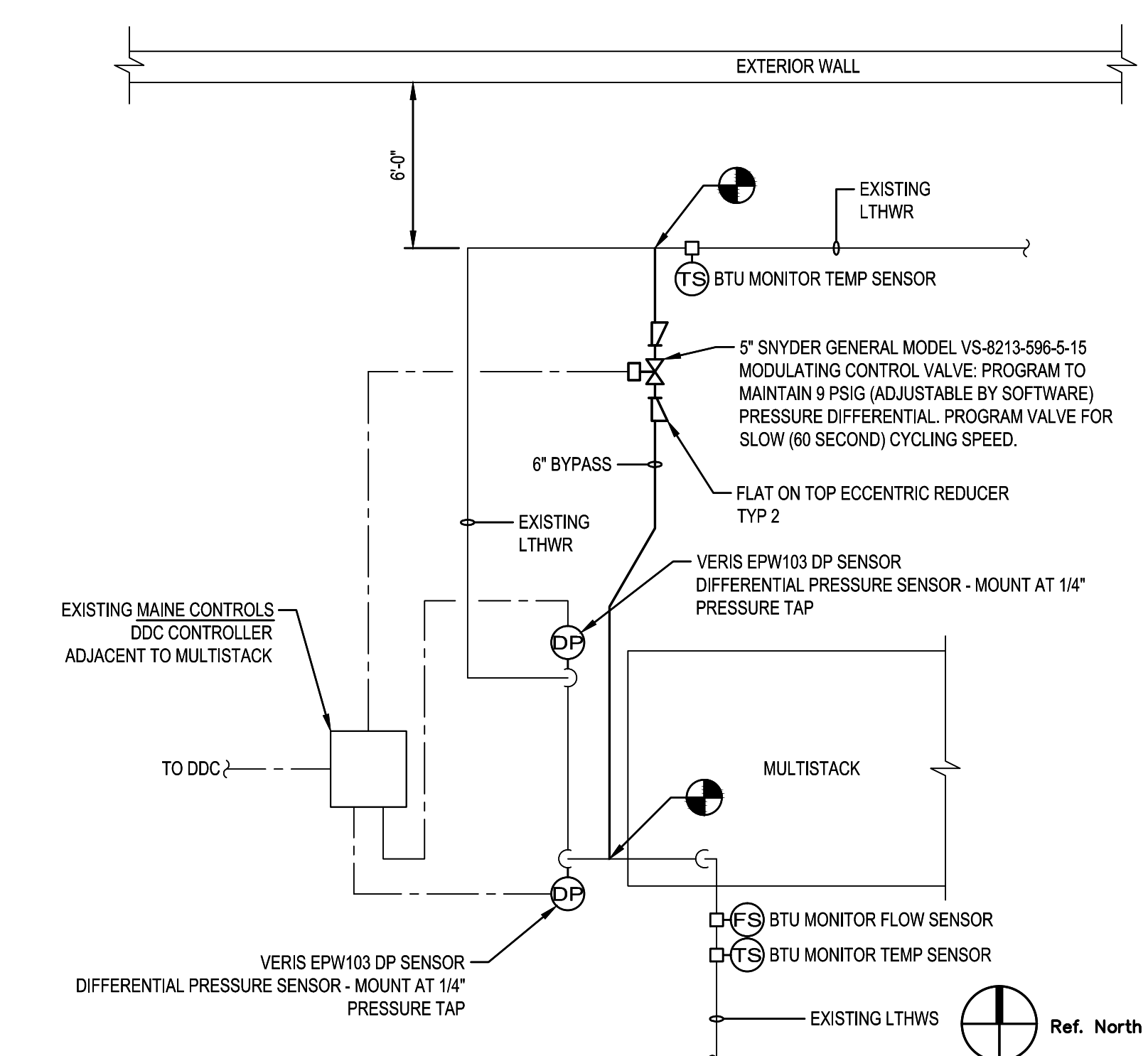
MULTISTACK LTHW BYPASS SCALE: NOT TO SCALE 2
