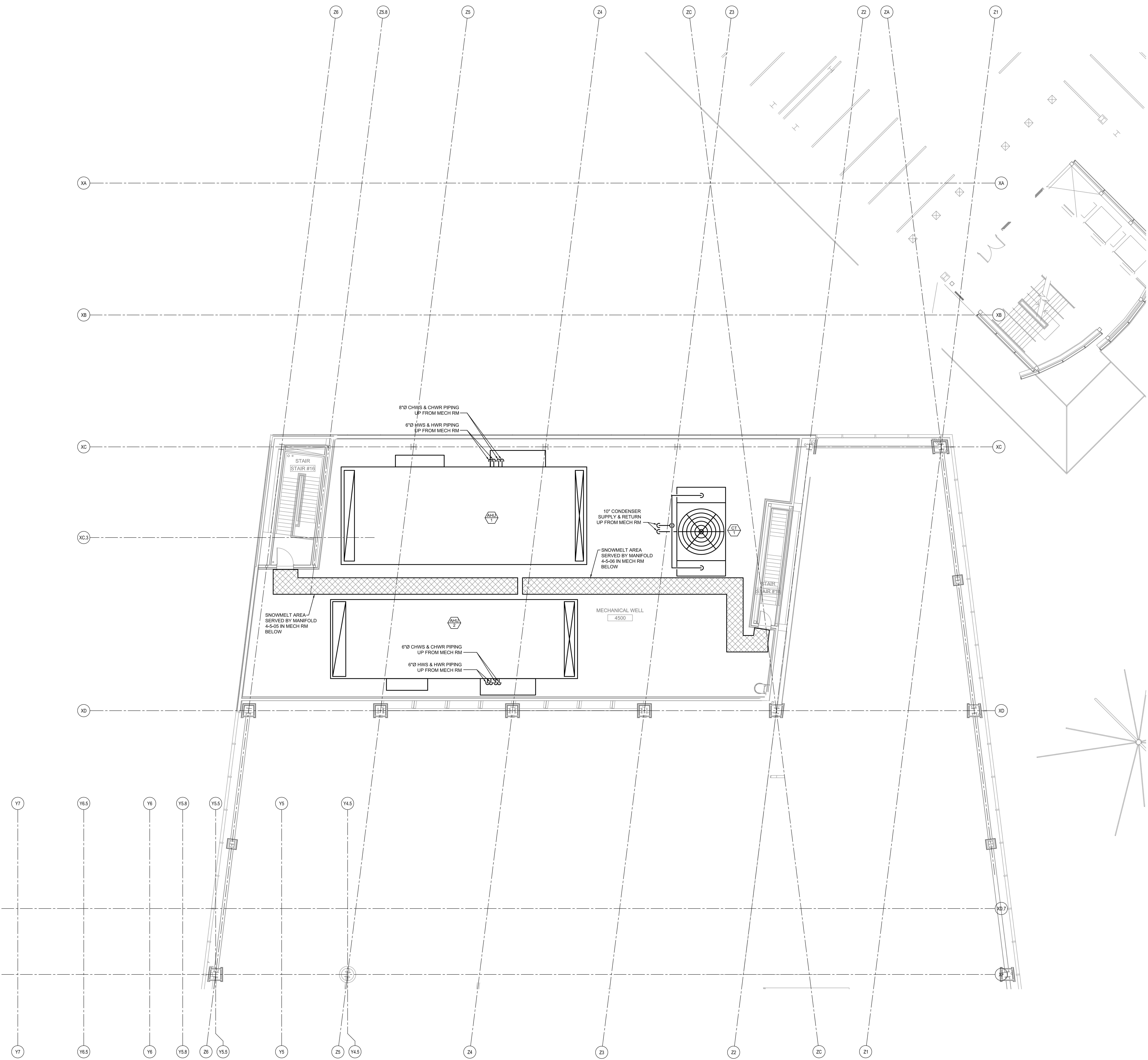
MECHANICAL PIPING PLAN - LEVEL 5 - ZONE 6 SCALE: 1/8" = 1'-0"
