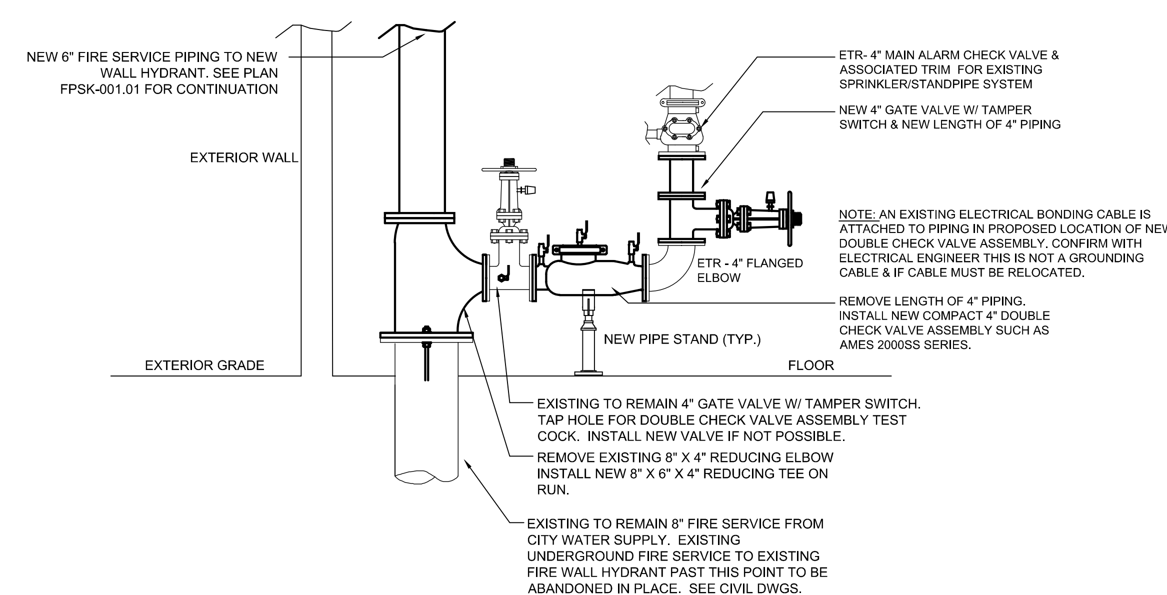
DETAIL- EXISTING TERMINAL WESTERLY SPRINKLER VALVE ROOM- NEW WORK SCALE: NTS
