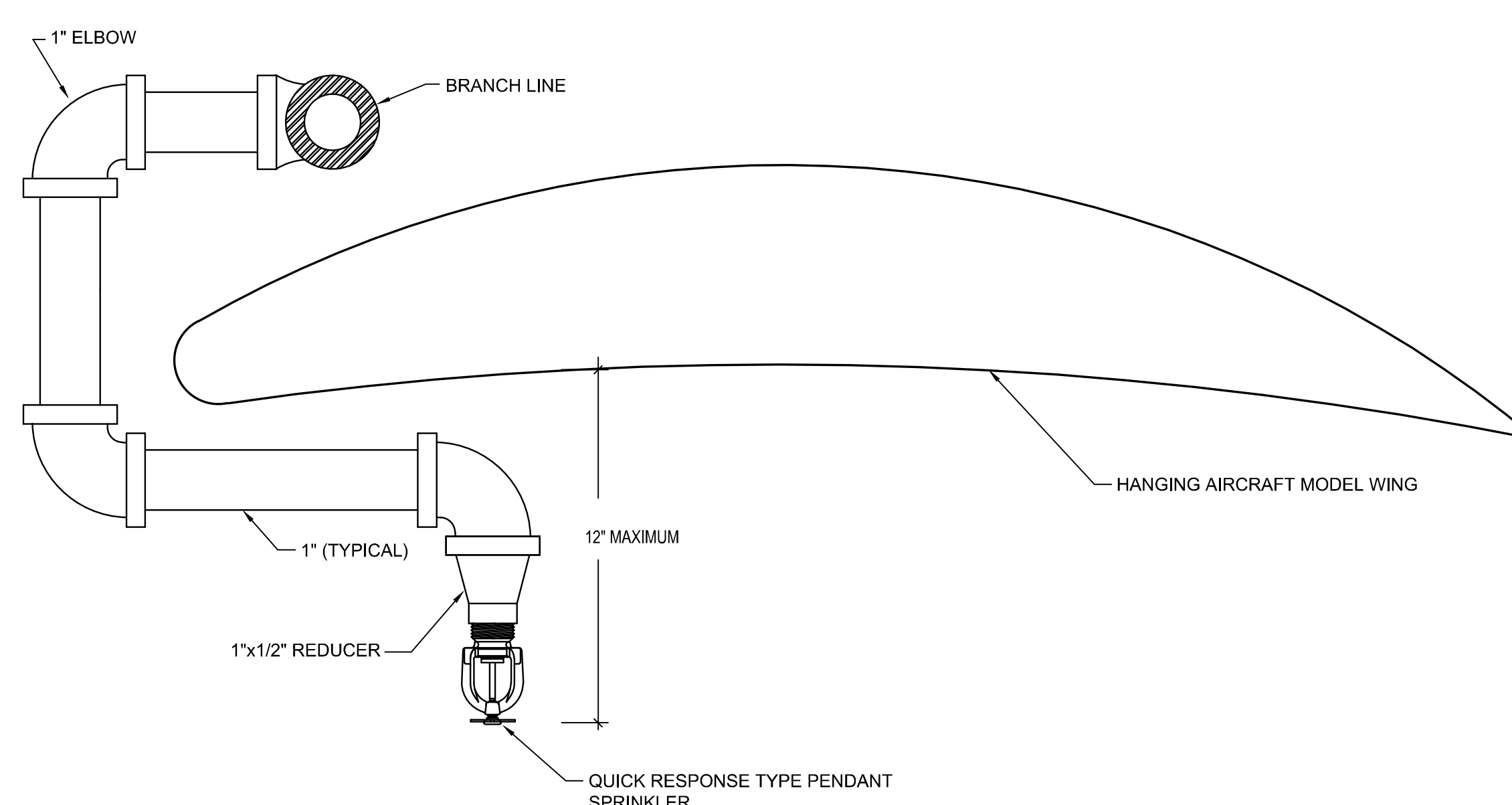
DETAIL- SPRINKLER "ARM UNDER" CROSS SECTION OF AIRCRAFT WING SCALE: NTS
