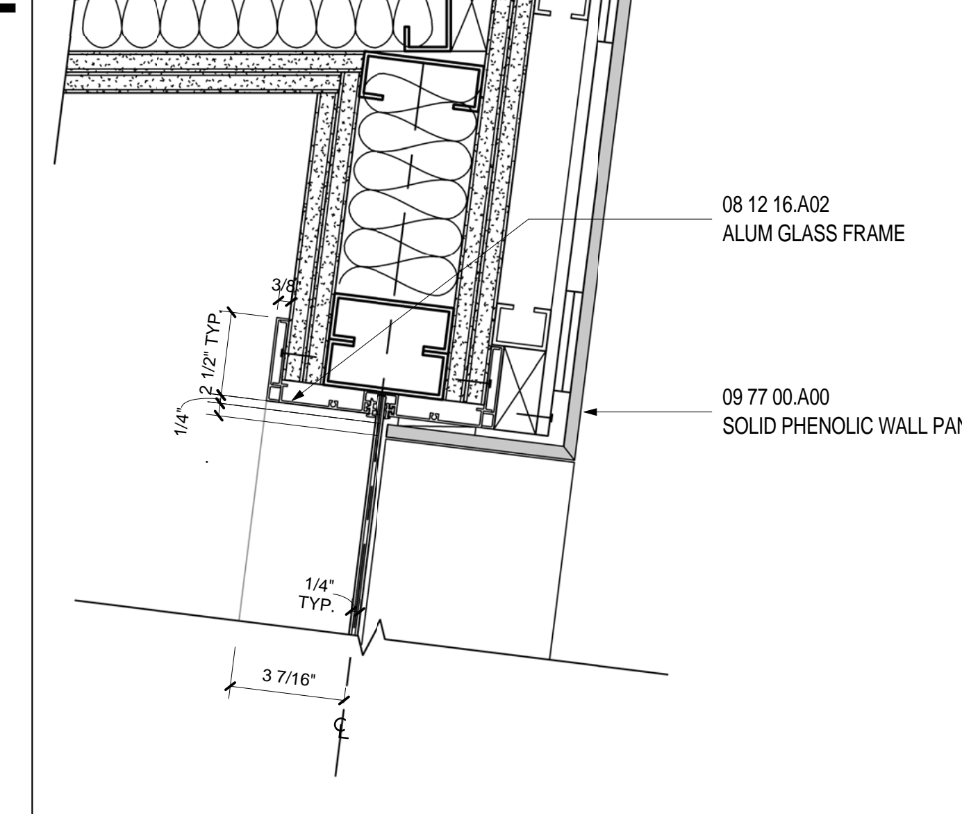
JAMB-INT.CUR.WALL AT LEO ROOM SCALE: 3" = 1'-0" A02.04.04 2
