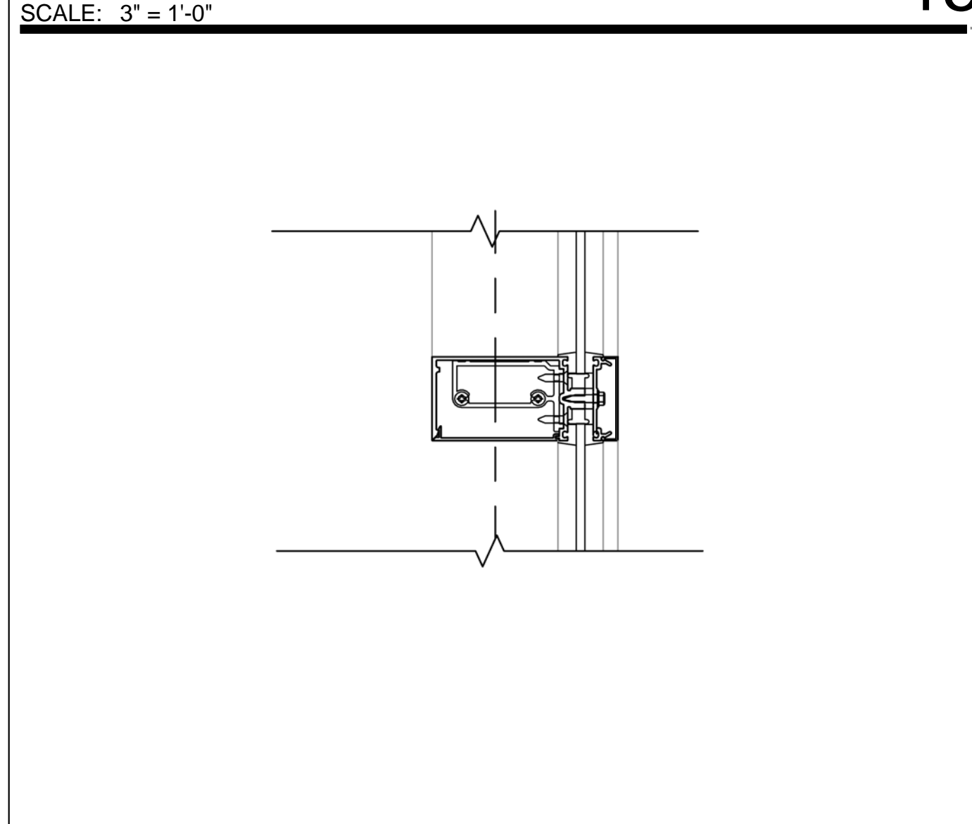
INTERMED MULLION- SSCP/TICKETING SCALE: 3" = 1'-0" A11.02 16
