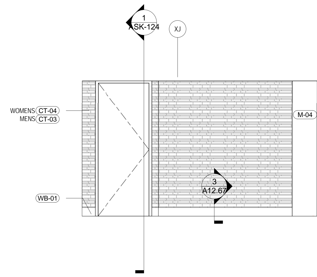
1B WOMENS ENTRY 2507 - EAST SCALE: 3/8" = 1'-0" A08.01
