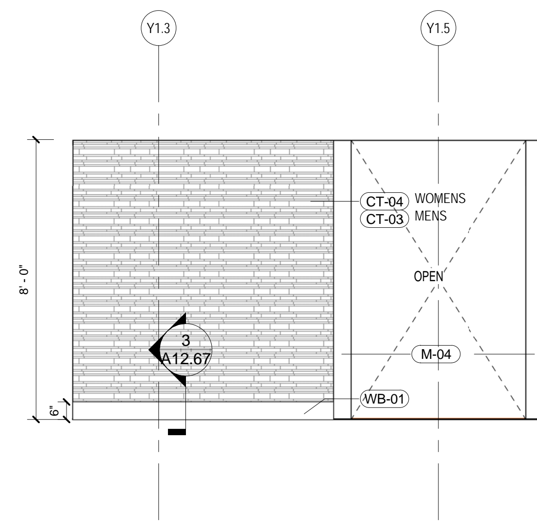
1C WOMENS ENTRY 2507 - SOUTH SCALE: 3/8" = 1'-0" A08.01
