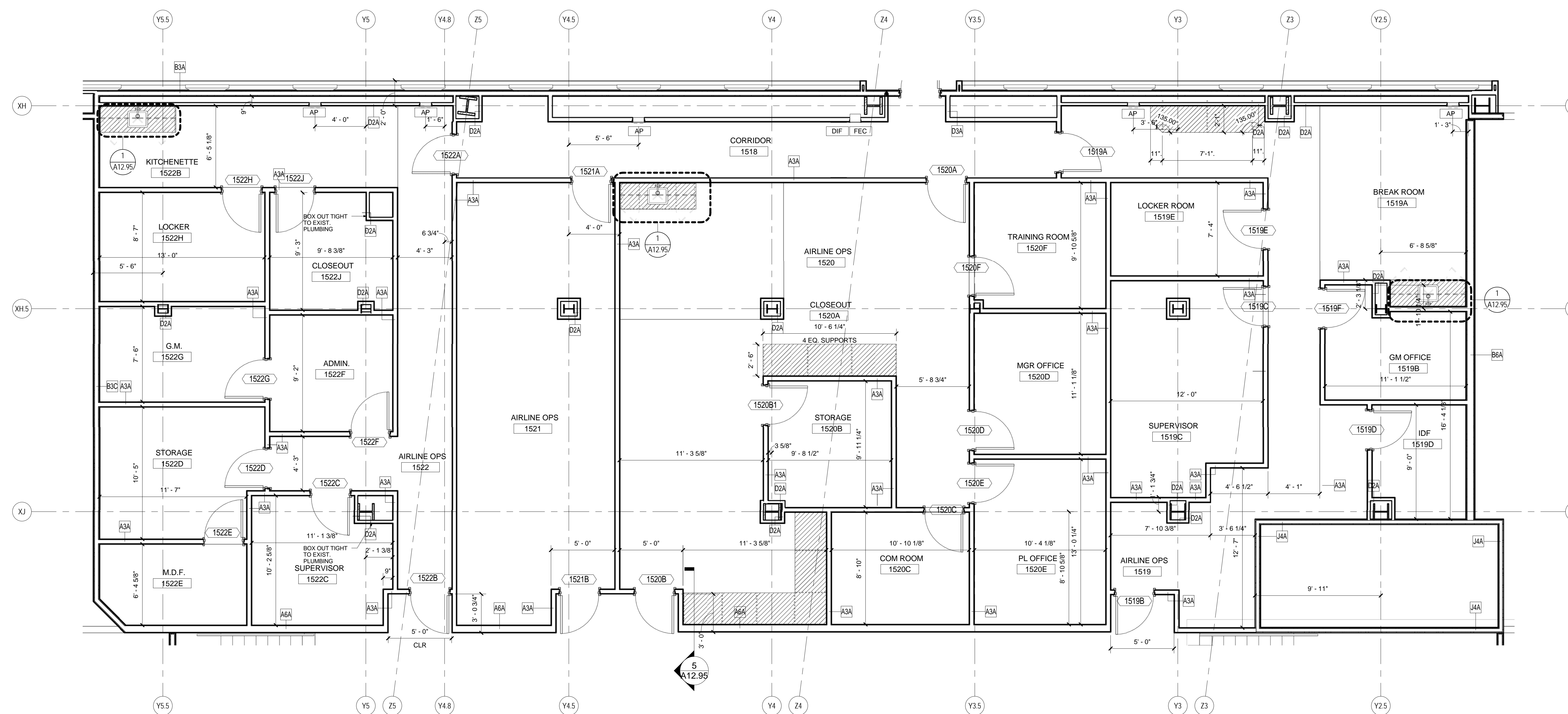
ENLARGED PLAN - LEVEL 2 - ATO
