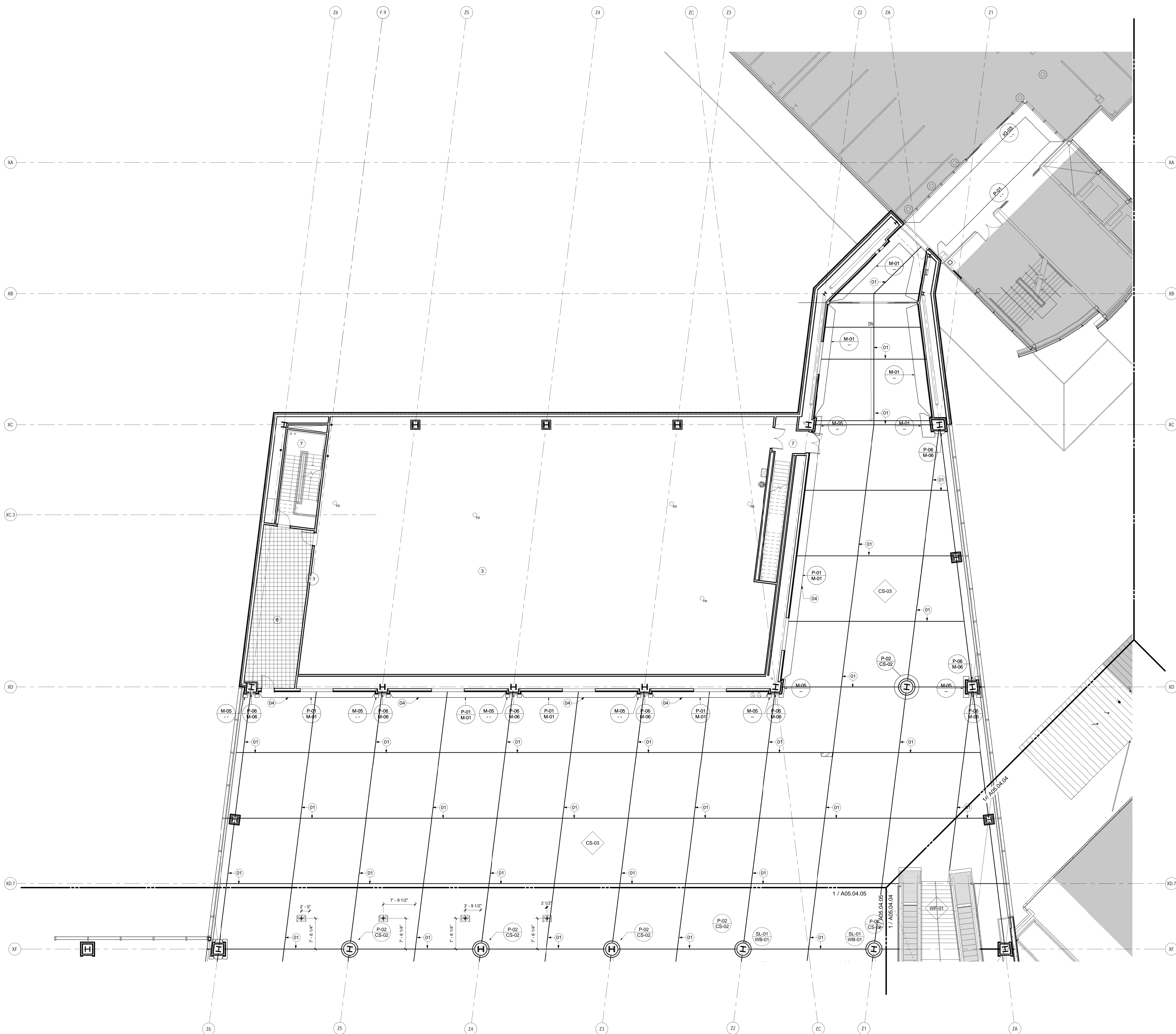
FINISH PLAN - LEVEL 4 - ZONE 6 SCALE: 1/8" = 1'-0"
