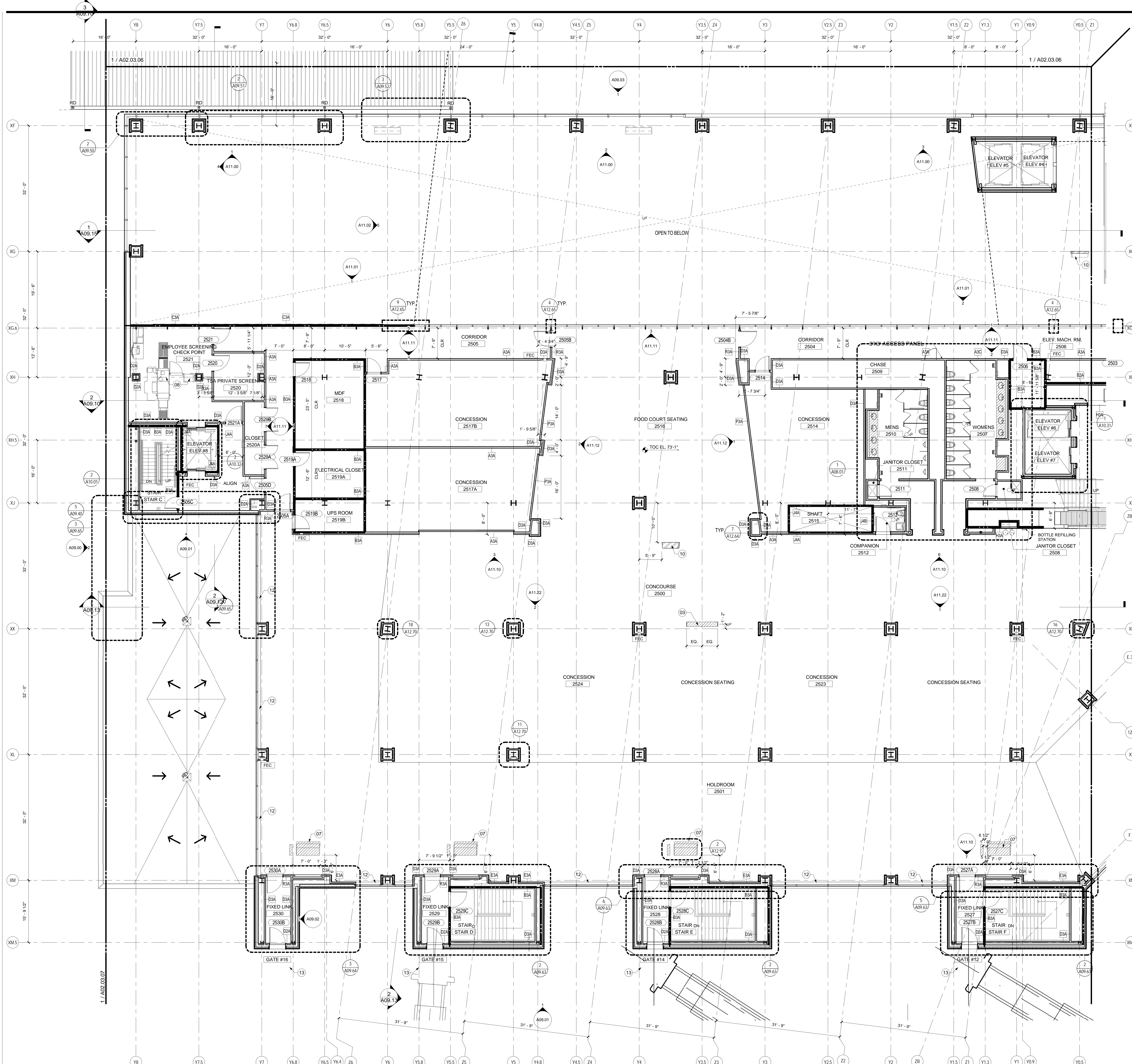
CONSTRUCTION PLAN - LEVEL 3 - ZONE 5
