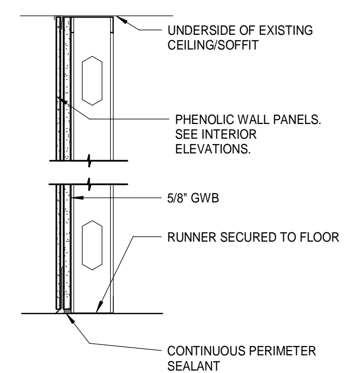
TYPE F3.b NON-RATED
