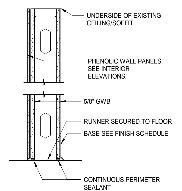
TYPE S3.b NON-RATED
