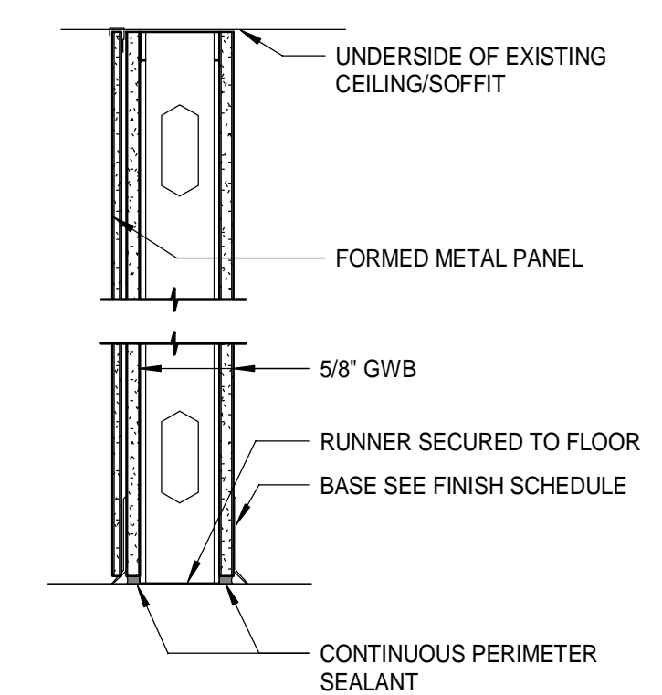
TYPE S3.c NON-RATED
