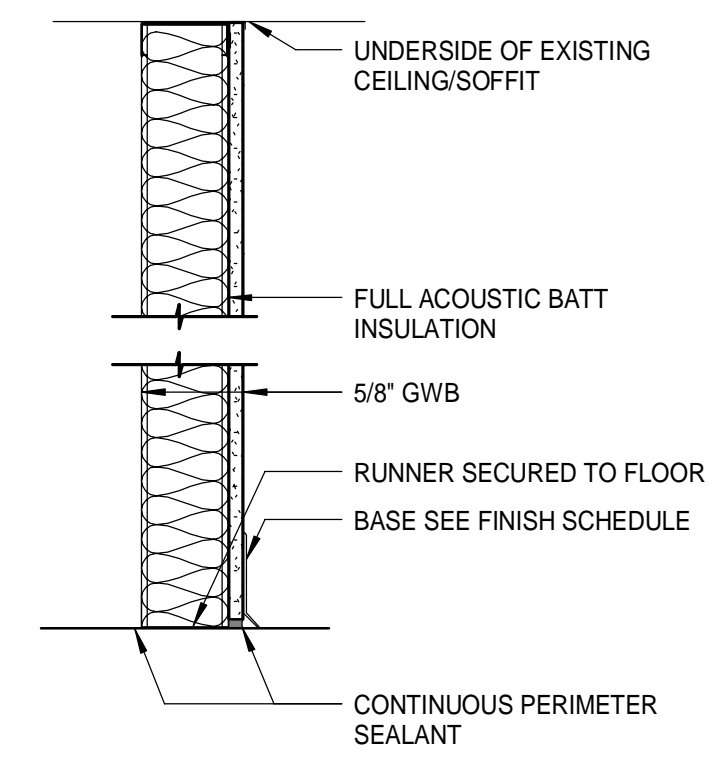
TYPE F3.a NON-RATED
