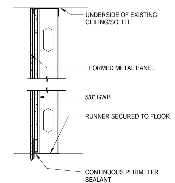
TYPE F3.c NON-RATED
