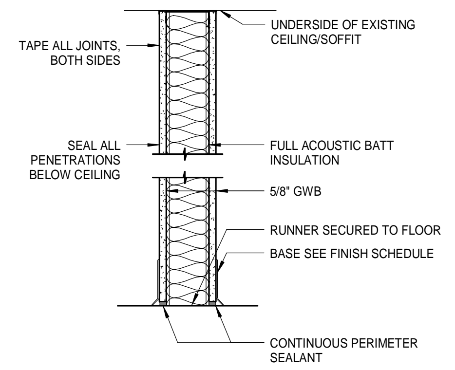
TYPE S3.a NON-RATED
