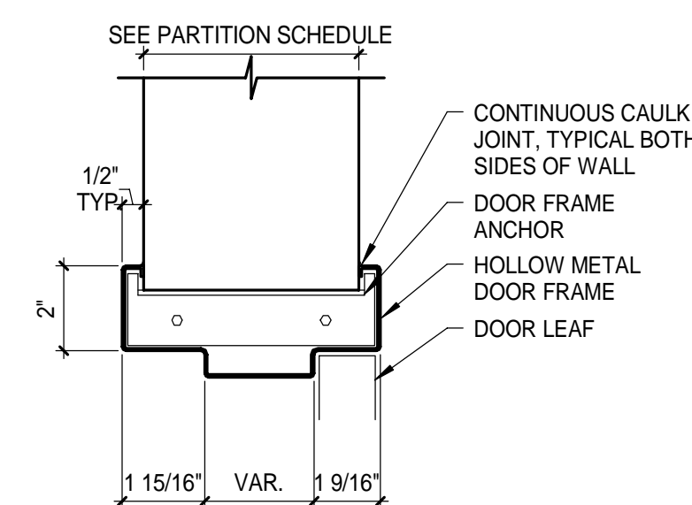
2 DOOR HEAD DETAIL 3" = 1'-0"
