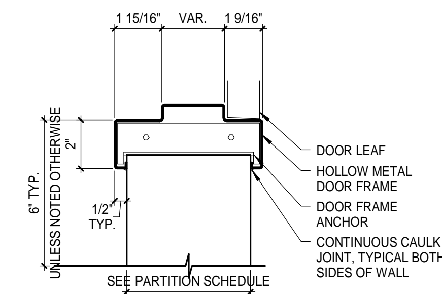
1 DOOR JAMB DETAIL 3" = 1'-0"
