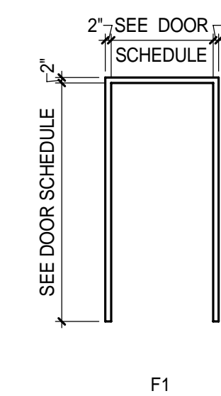
3 TYPE DOOR FRAME 1/4" = 1'-0"
