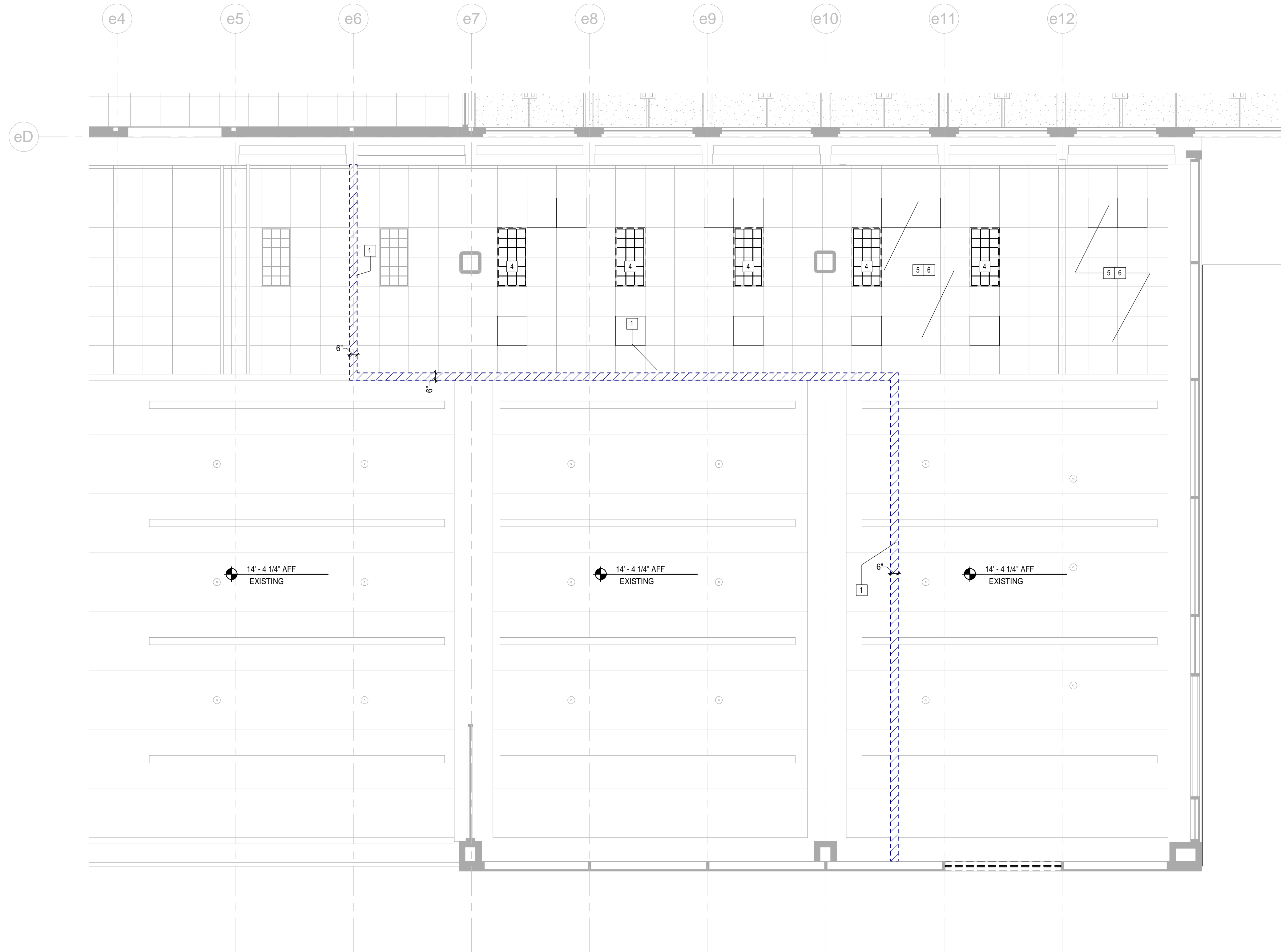
1 2ND FLOOR - 1 DEMO REFLECTED CEILING PLAN 1/4" = 1'-0"
