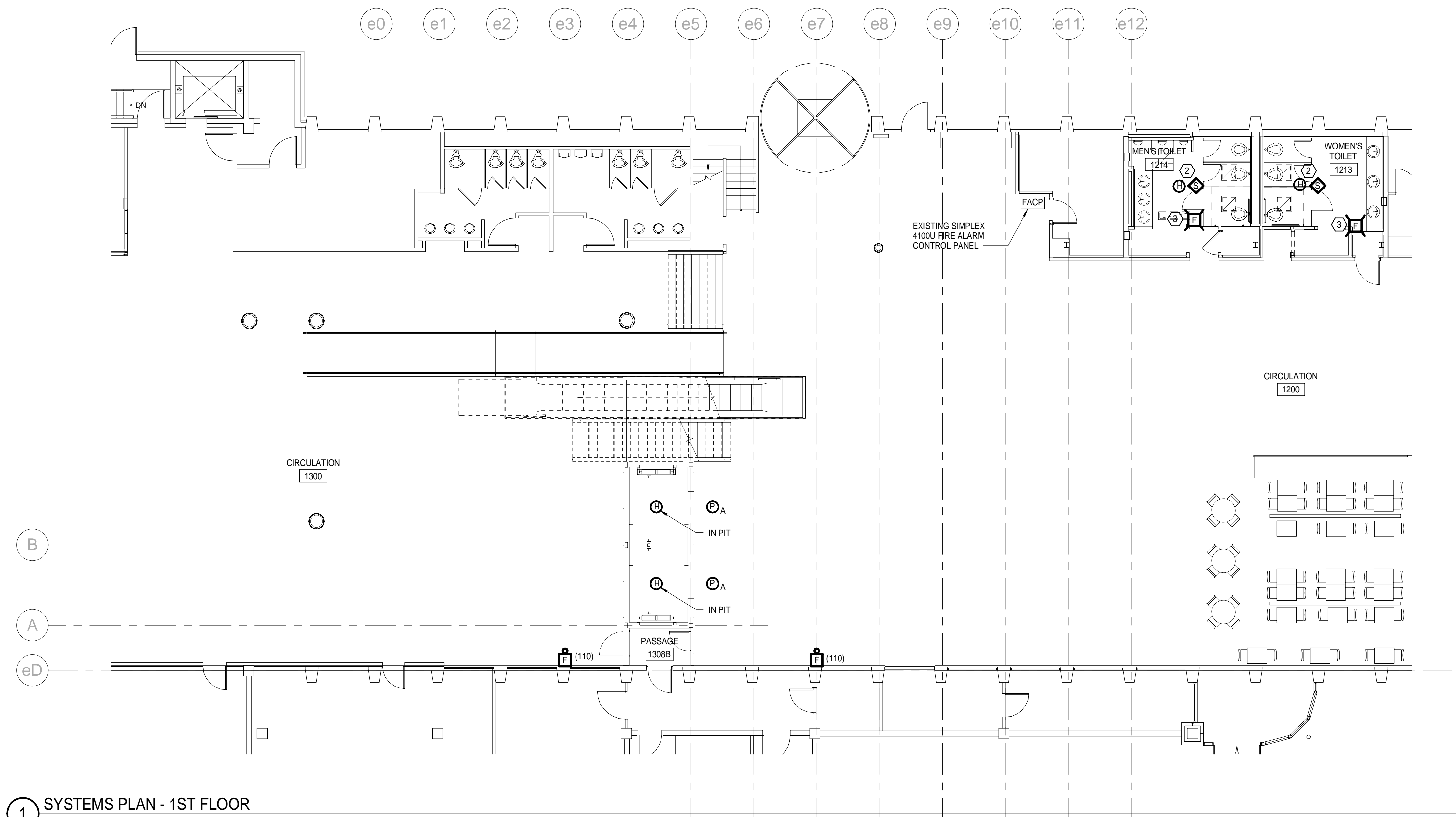
1 SYSTEMS PLAN - 1ST FLOOR 1/8" = 1'-0"
